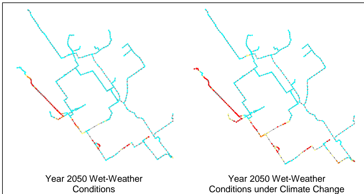
Figure 10.3 Calculated Collection System Surcharging for Design Storm with Existing Conditions and Climate Change Conditions in Year 2050
