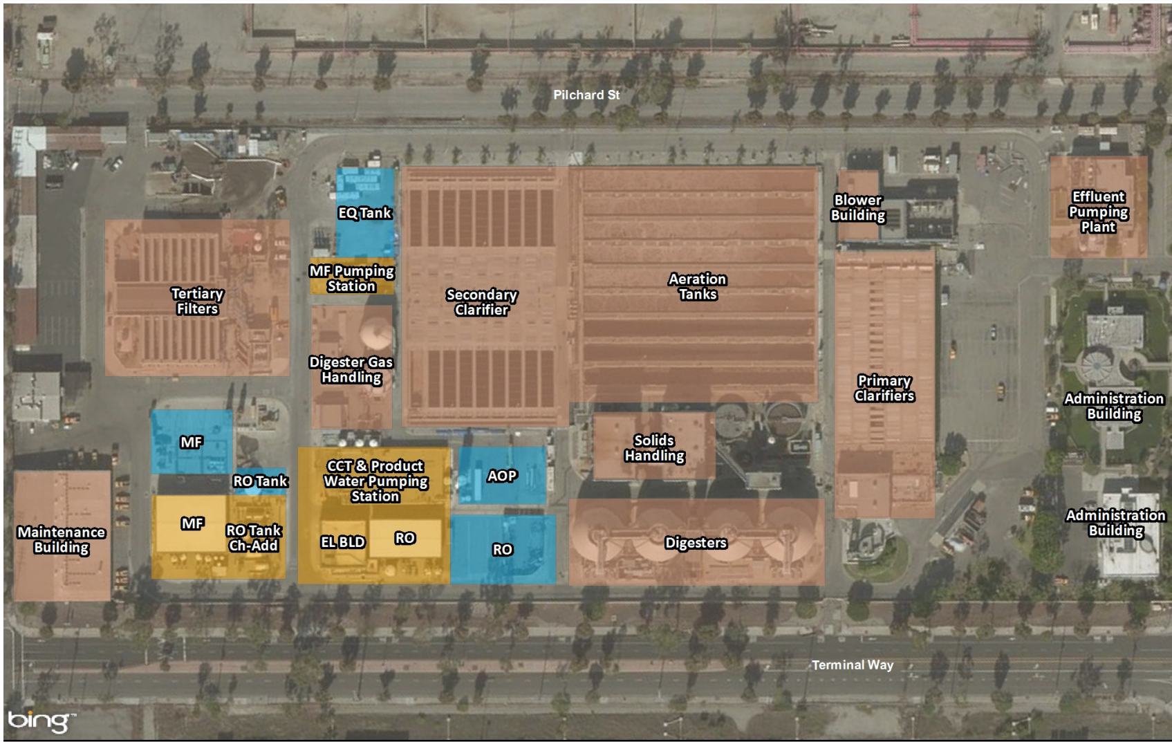
Figure 7.6 Site Layout for Phase 1 and Phase 2 AWP at TIWRP One Water LA 2040 Plan
