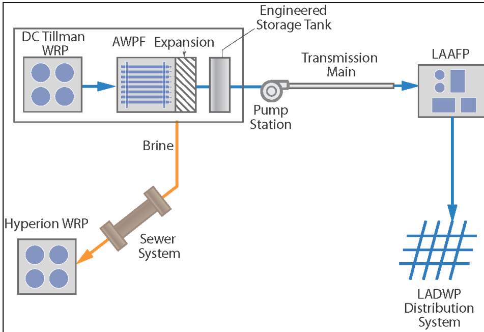
Figure D.7 Process Flow Schematic for Concept Option # 15 (DCTWRP to LAAFP)
