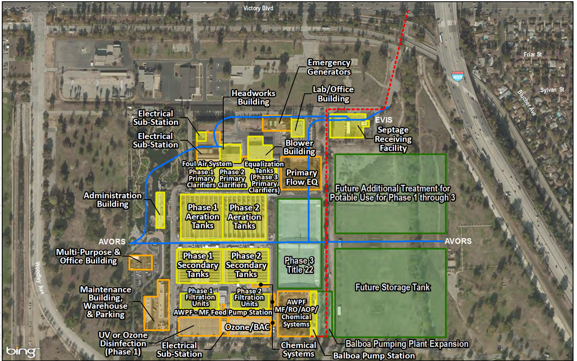
Figure 5.9 Potential Upgrades for Concept Option #15 (DCTWRP to LAAFP) One Water LA 2040 Plan
