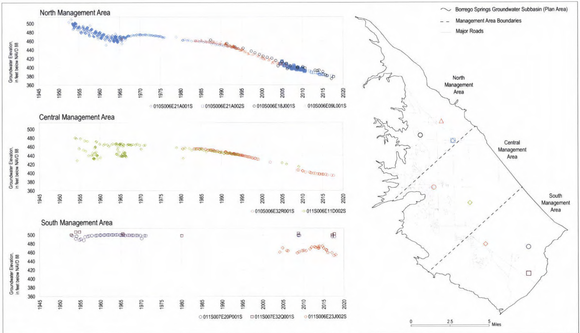
FIGURE 2.2-13E Groundwater Levels in Selected Wells in Parts of the Plan Area, 1952 - 2018 Groundwater Sustainability Plan for the Borrego Springs Groundwater Subbasin
