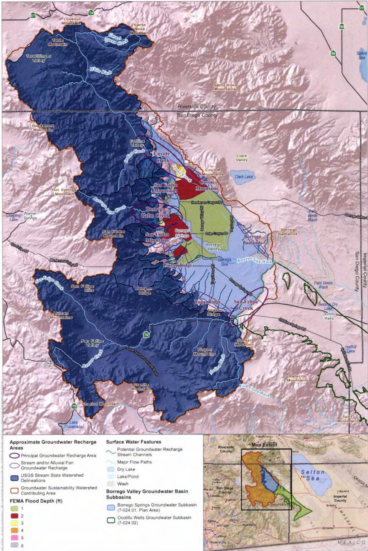
Figure 2.2-11 Areas of Focused Stream Recharge in the Plan Area Groundwater Sustainability Plan for the Borrego Springs Groundwater Subbasin
