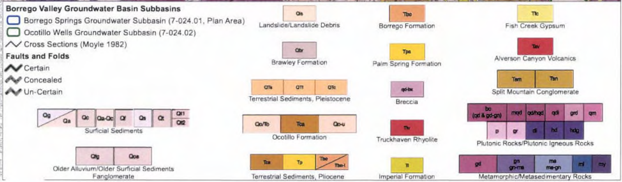
Figure 2.2-8 Geologic Map
