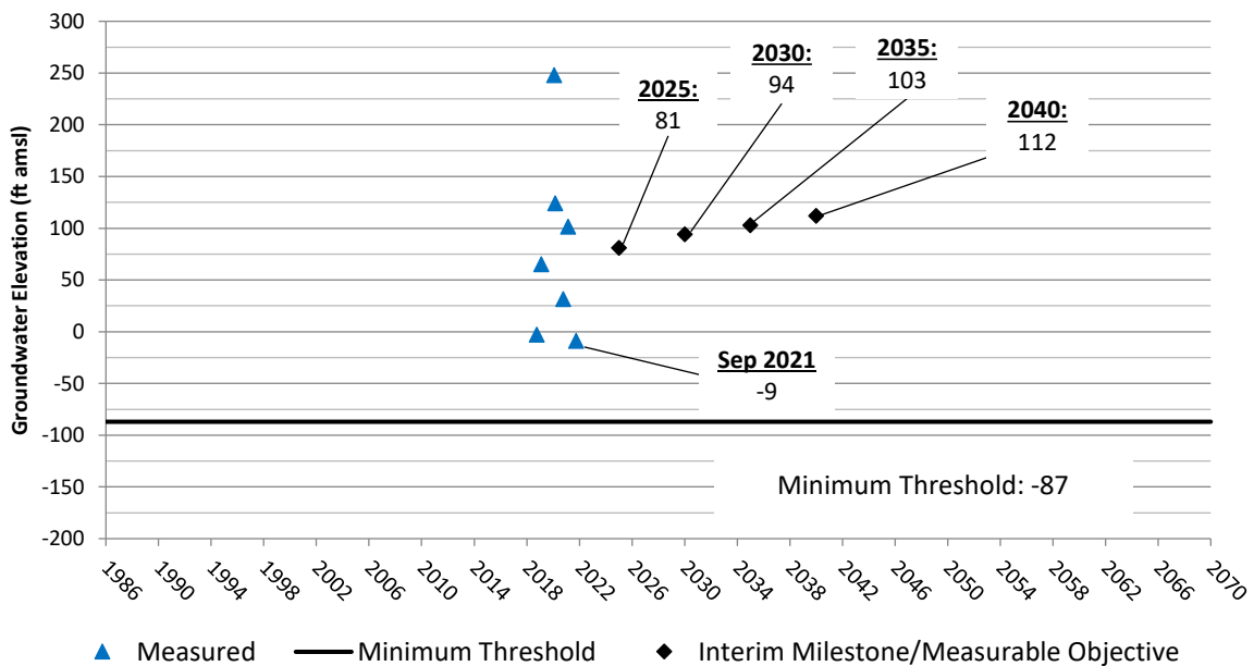
23S/27E-27 (Santa Margarita Formation) ETGSA
