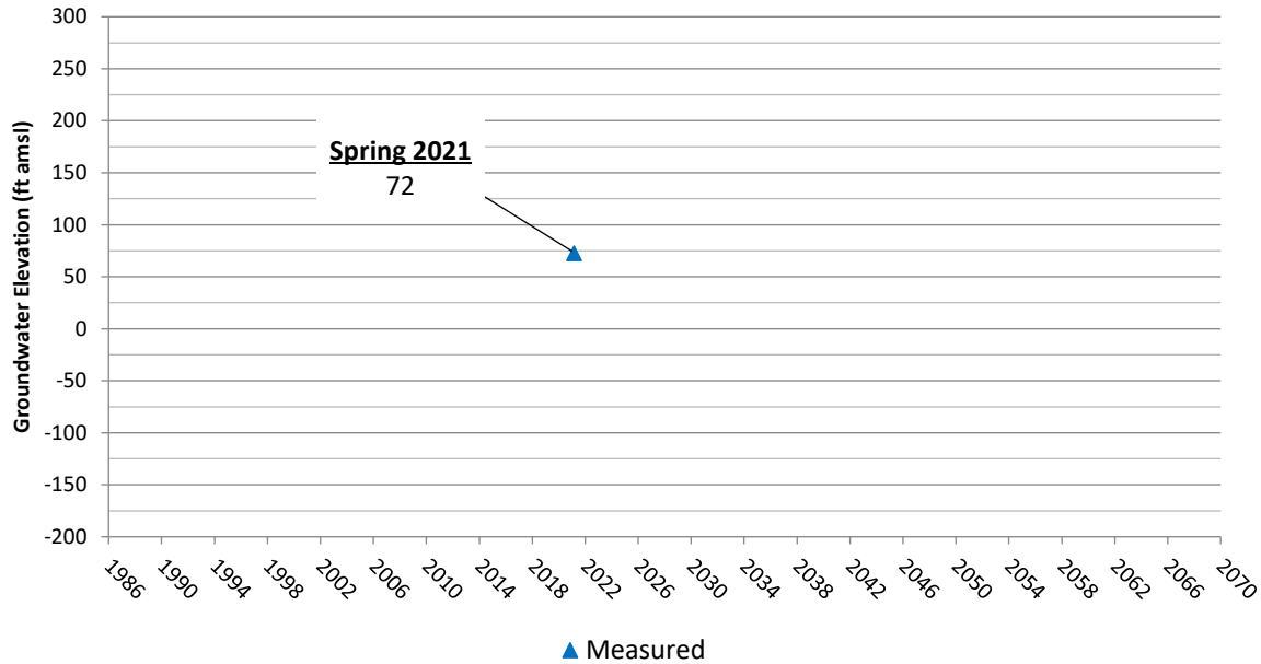
21S/23E-31 (Upper) LTRID GSA
