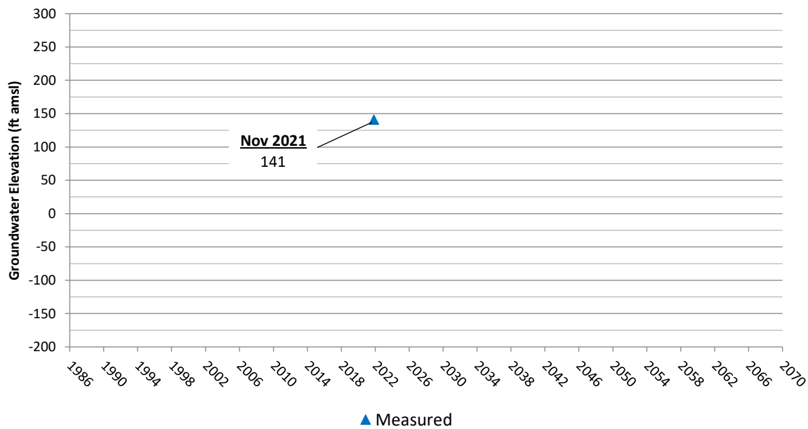
TSS PIDGSA-01 U (Upper) Pixley ID GSA
