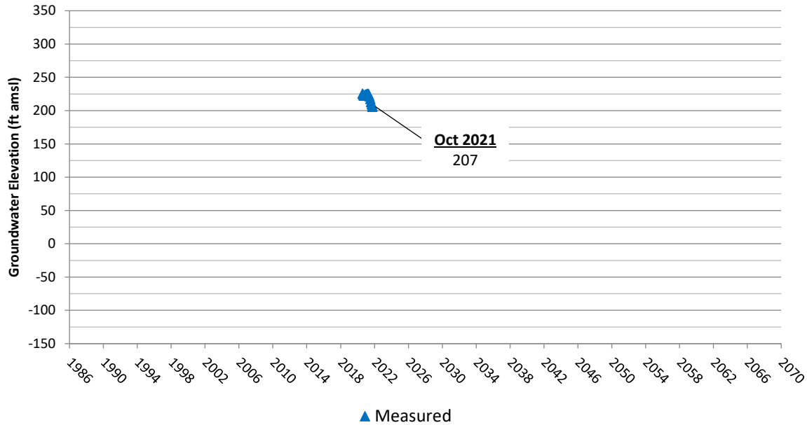
TSMW 6L (Lower) ETGSA
