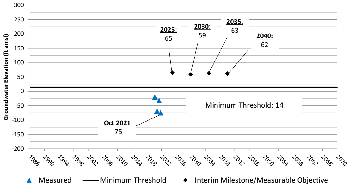
23S/25E-16N04 (Upper) Pixley ID GSA
