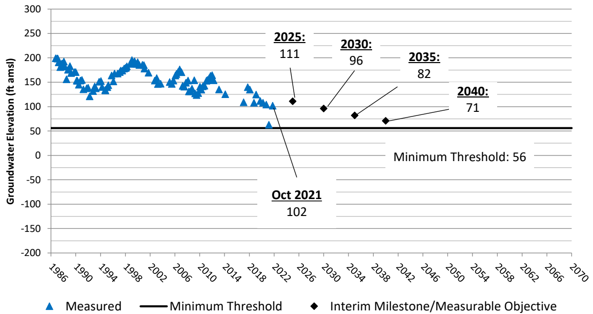
21S/23E-32K01 (Upper) LTRID GSA
