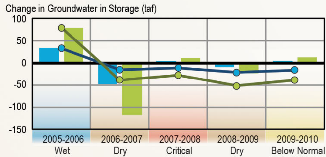
Figure E-27 Annual Change in Groundwater in Storage for the East Butte Subbasin (5-21.59) in the Sacramento River Hydrologic Region (Spring 2005-2010)
