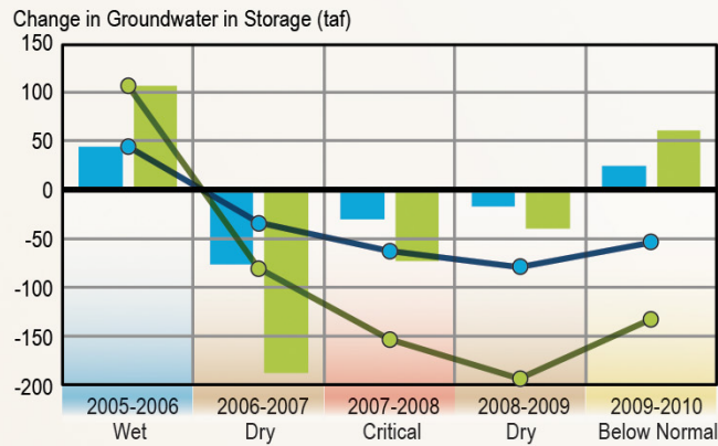
Figure E-33 Annual Change in Groundwater in Storage for the Solano Subbasin (5-21.66) in the Sacramento River Hydrologic Region (Spring 2005-Spring 2010)
