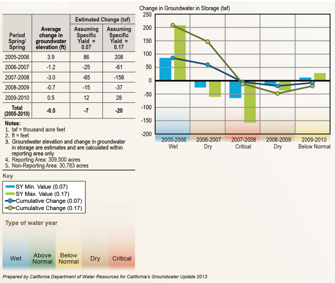
Figure E-31 Annual Change in Groundwater in Storage for the North American Subbasin (5-21.64) in the Sacramento River Hydrologic Region (Spring 2005-2010)
