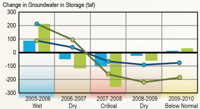
Figure E-10 Annual Change in Groundwater in Storage for the Southeast Sacramento Valley Subbasin Group in the Sacramento River Hydrologic Region (Spring 2005-Spring 2010)
