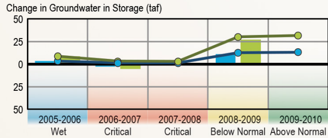
Figure E-49 Annual Change in Groundwater in Storage for the Tracy Subbasin (5-21.15) in the San Joaquin River Hydrologic Region (Spring 2005-Spring 2010)
