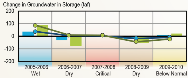
Figure E-9 Annual Change in Groundwater in Storage for the Redding Area Subbasin Group in the Sacramento River Hydrologic Region (Spring 2005-Spring 2010)
