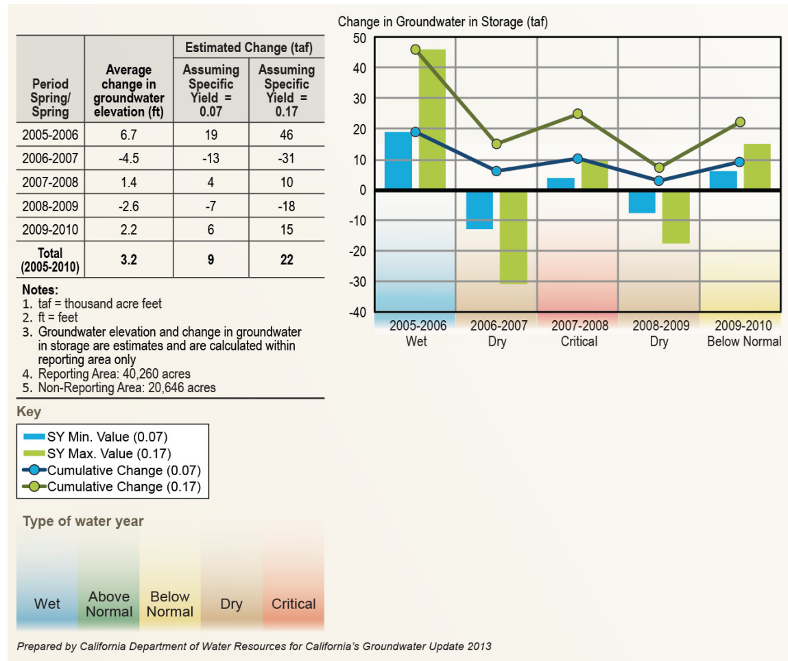
Figure E-17 Annual Change in Groundwater in Storage for the Enterprise Subbasin (5-6.04) in the Sacramento River Hydrologic Region (Spring 2005-Spring 2010)
