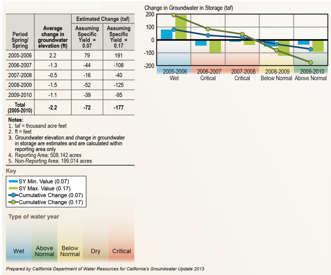
Figure E-36 Annual Change in Groundwater in Storage for the Eastern San Joaquin Subbasin (5-22.01) in the San Joaquin River Hydrologic Region (Spring 2005-2010)
