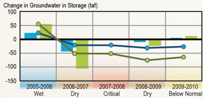
Figure E-25 Annual Change in Groundwater in Storage for the Vina Subbasin (5-21.57) in the Sacramento River Hydrologic Region (2005-2010)
