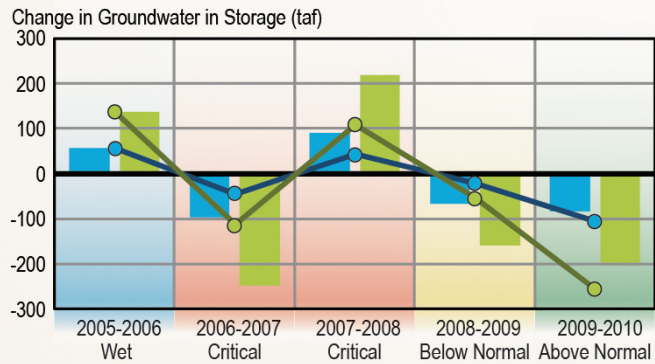
Figure E-41 Annual Change in Groundwater in Storage for the Madera Subbasin (5-22.06) in the San Joaquin River Hydrologic Region (Spring 2005-Spring 2010)
