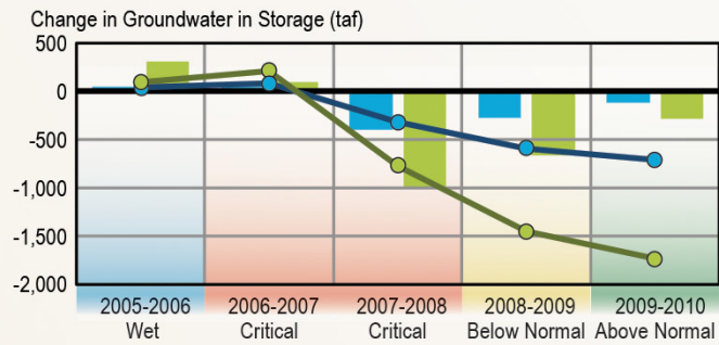
Figure E-43 Annual Change in Groundwater in Storage for the Kings Subbasin (5-22.08) in the Tulare Lake Hydrologic Region (Spring 2005-Spring 2010)
