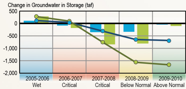
Figure E-47 Annual Change in Groundwater in Storage for the Tule Subbasin (5-22.13) in the Tulare Lake Hydrologic Region (Spring 2005-Spring 2010)
