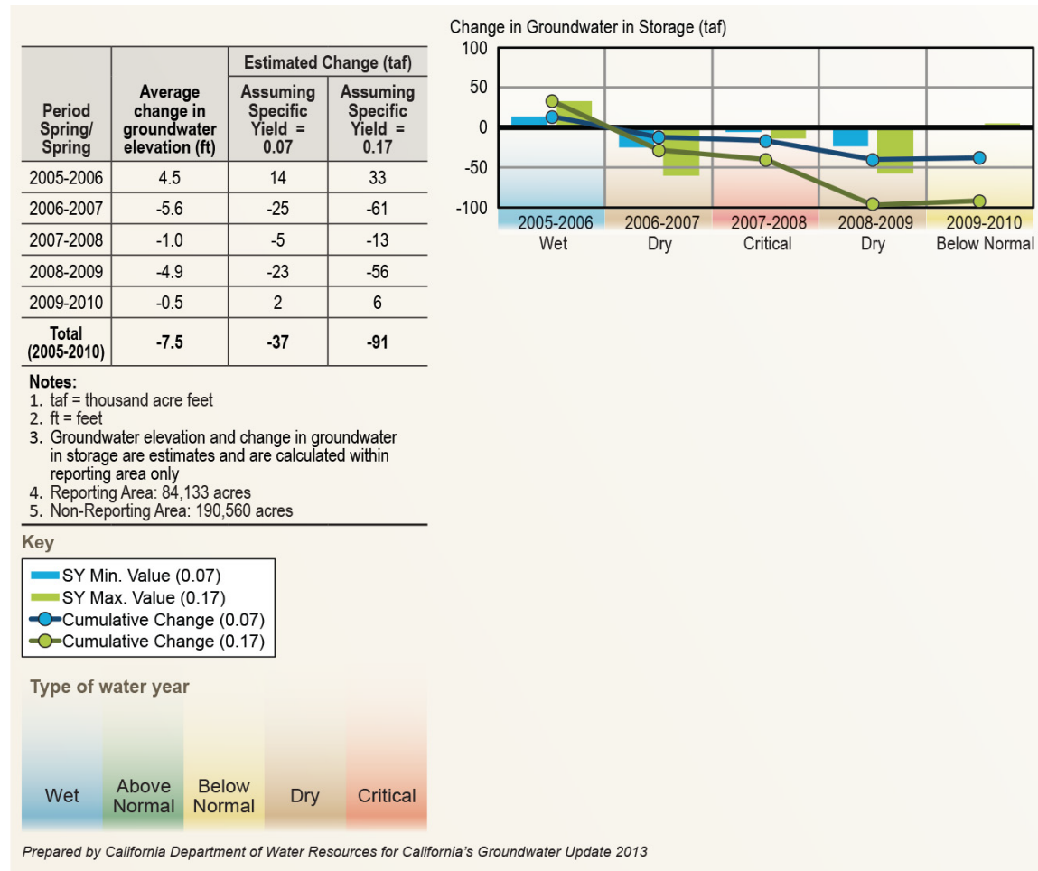
Figure E-19 Annual Change in Groundwater in Storage for the Red Bluff Subbasin (5-21.50) in the Sacramento River Hydrologic Region (Spring 2005-Spring 2010)
