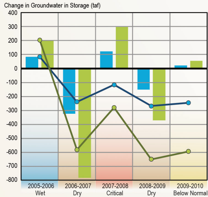
Figure E-21 Annual Change in Groundwater in Storage for the Colusa Subbasin (5-21.52) in the Sacramento River Hydrologic Region (Spring 2005-Spring 2010)
