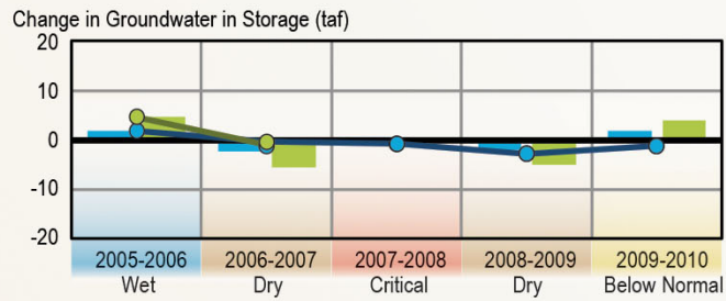
Figure E-23 Annual Change in Groundwater in Storage for the Dye Creek Subbasin (5-21.55) in the Sacramento River Hydrologic Region (Spring 2005-Spring 2010)
