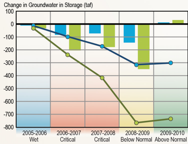
Figure E-39 Annual Change in Groundwater in Storage for the Merced Subbasin (5-22.04) in the San Joaquin River Hydrologic Region (Spring 2005-Spring 2010)
