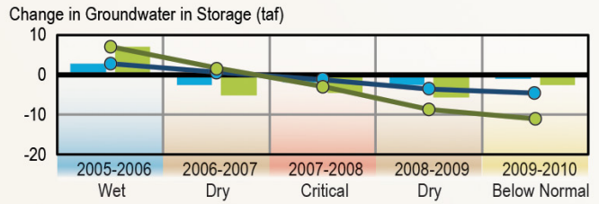
Figure E-14 Annual Change in Groundwater in Storage for the Bowman Subbasin (5-6.01) in the Sacramento River Hydrologic Region (Spring 2005-Spring 2010)
