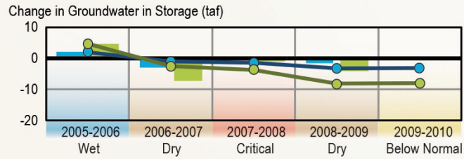
Figure E-15 Annual Change in Groundwater in Storage for the Rosewood Subbasin (5-6.02) in the Sacramento River Hydrologic Region (Spring 2005-Spring 2010)
