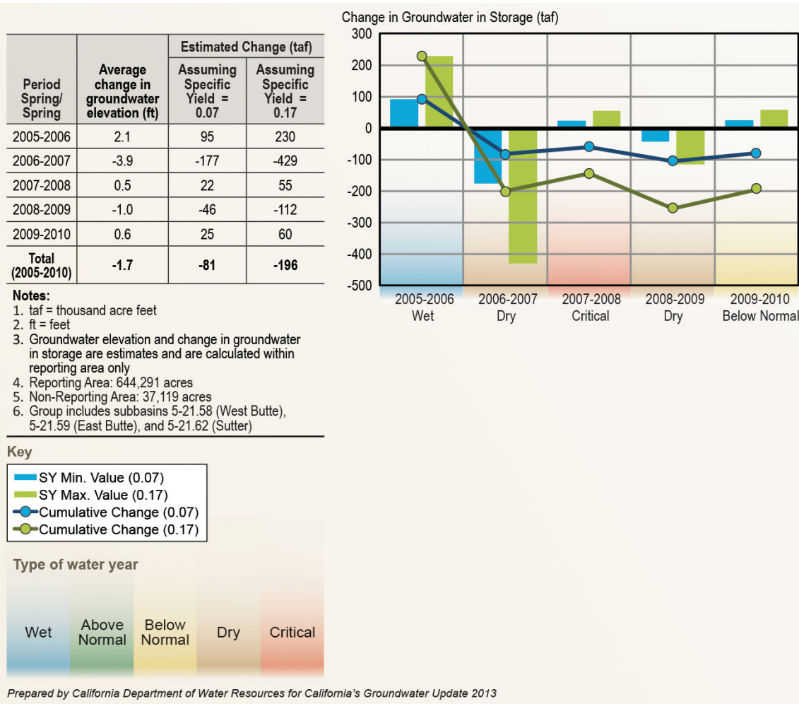
Figure E-5 Annual Change in Groundwater in Storage for the Central Sacramento Valley Subbasin Group in the Sacramento River Hydrologic Region (Spring 2005-2010)
