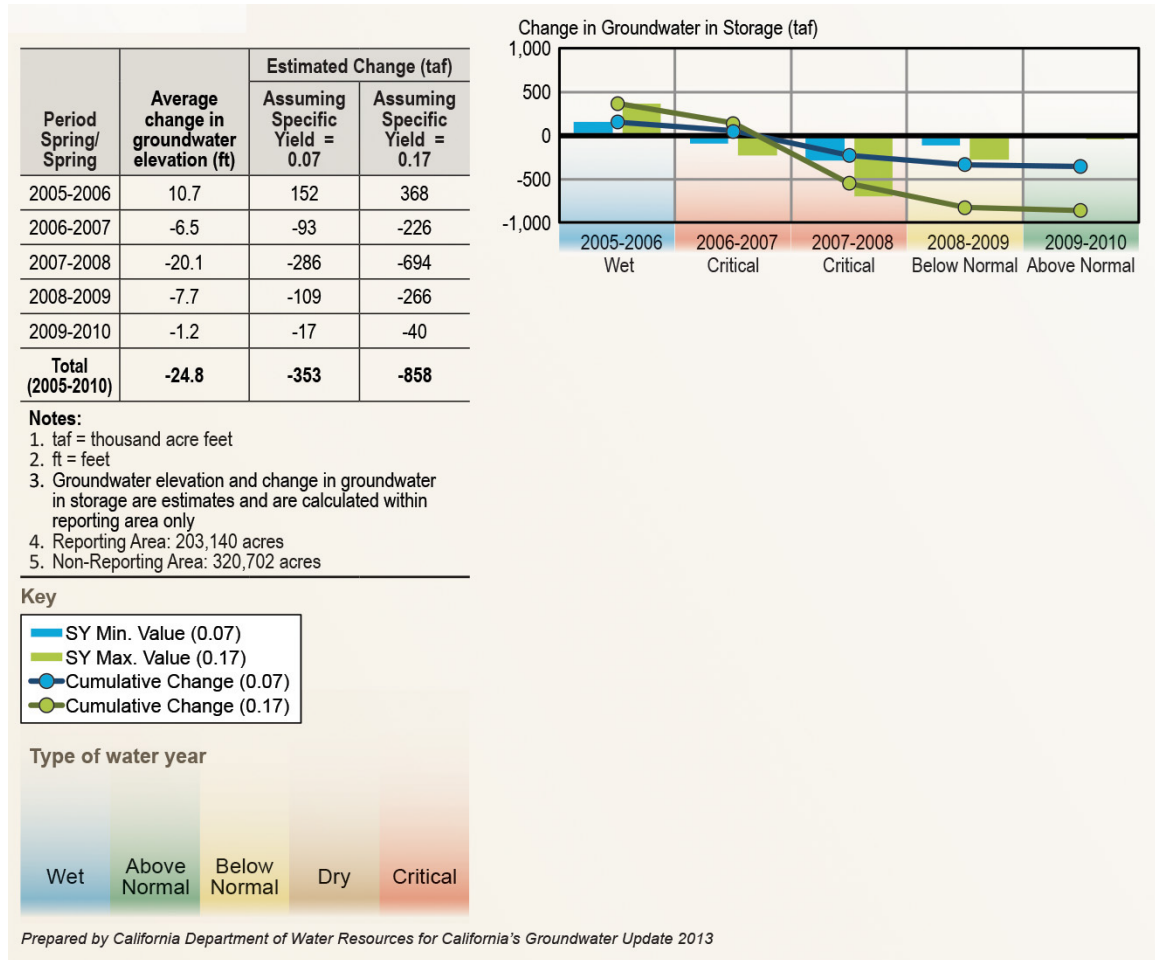
Figure E-46 Annual Change in Groundwater in Storage for the Tulare Lake Subbasin (5-22.12) in the Tulare Lake Hydrologic Region (Spring 2005-Spring 2010)
