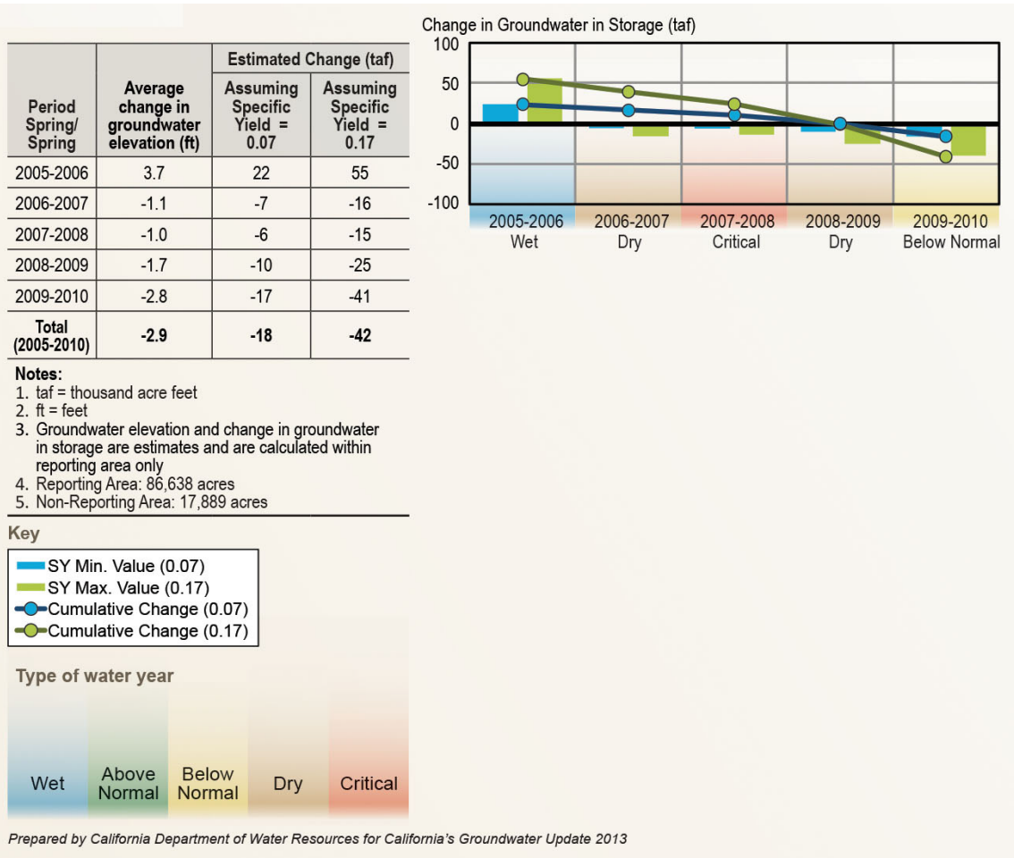
Figure E-29 Annual Change in Groundwater in Storage for the South Yuba Subbasin (5-21.61) in the Sacramento River Hydrologic Region (Spring 2005-Spring 2010)
