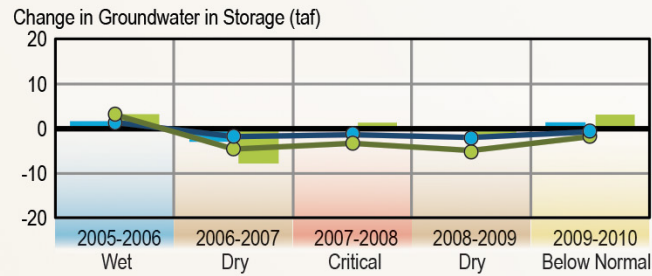
Figure E-35 Annual Change in Groundwater in Storage for the Capay Valley Subbasin (5-21.68) in the Sacramento River Hydrological Region (Spring 2005-Spring 2010)
