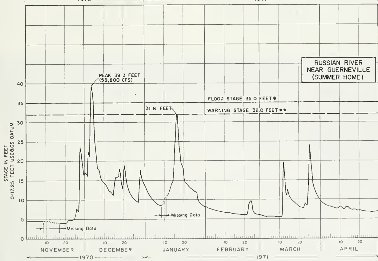
Figure 9 : HYDROGRAPHS OF RUSSIAN RIVER
