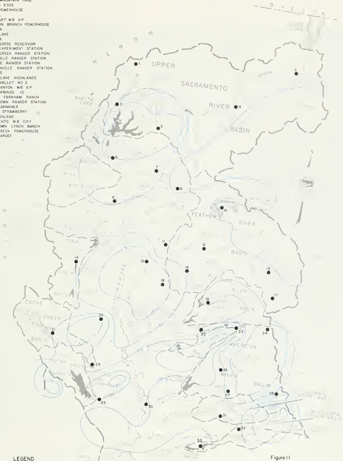
Figure II SACRAMENTO VALLEY AREA PRECIPITATION STATION LOCATION AND PERCENT OF NORMAL RAINFALL MAP
