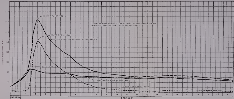
HIGH WATER OF 1962 - 63 JANUARY - FEBRUARY 1963 STORM HYDROGRAPHS OF CACHE CREEK AND FLOW PAST LATITUDE OF SACRAMENTO PUTAH CREEK, LAKE BERRYESSA RESERVOIR OPERATION
