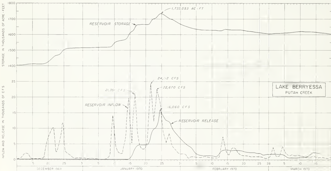
HYDROGRAPHS OF FOLSOM AND BERRYESSA LAKES
