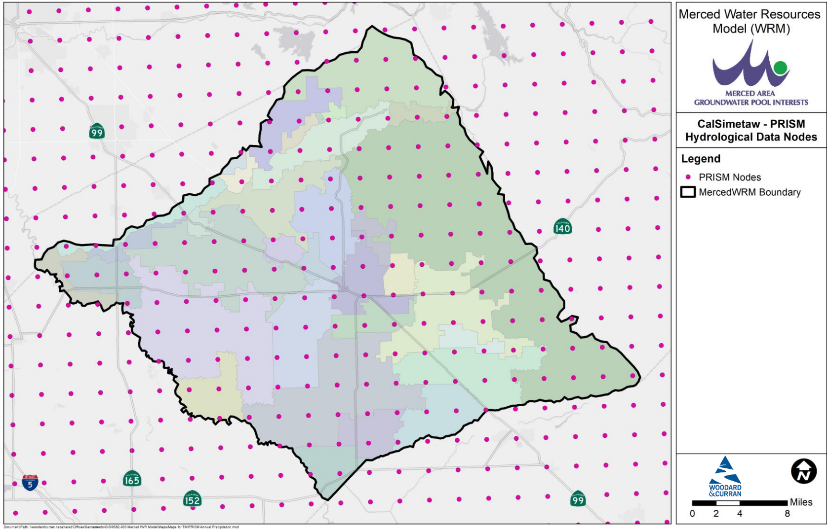
Figure 5: PRISM Grid
