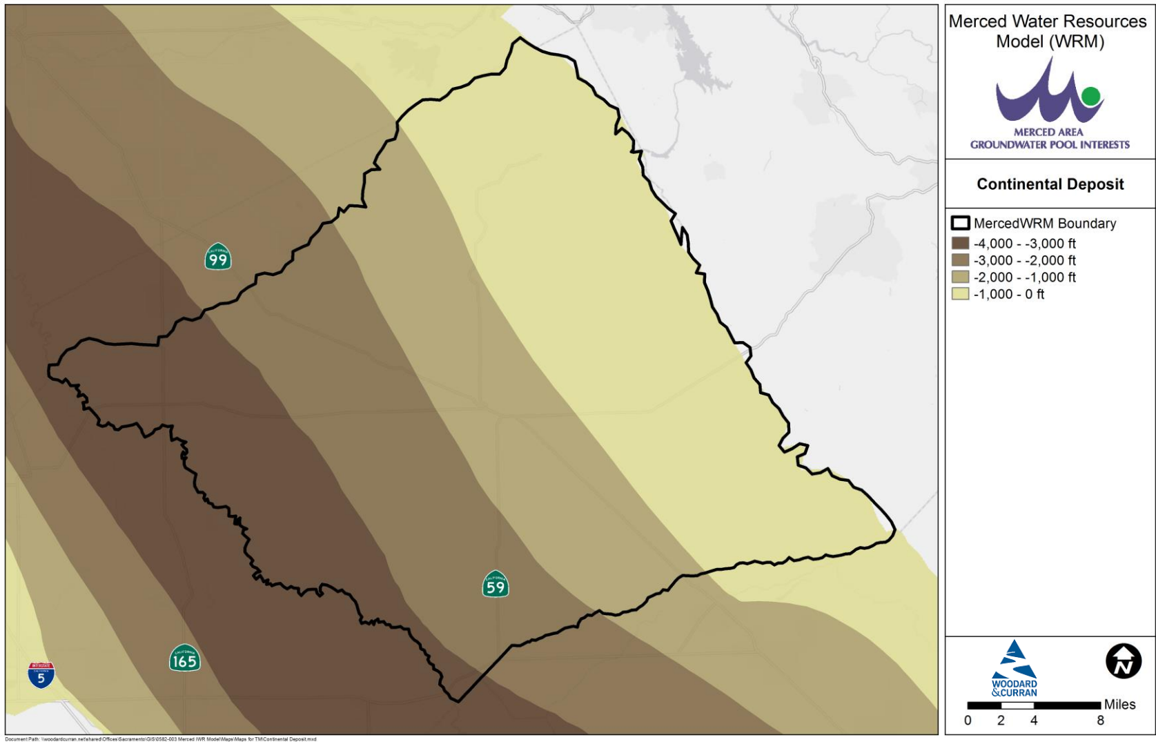
Figure 26: Continental Deposit
