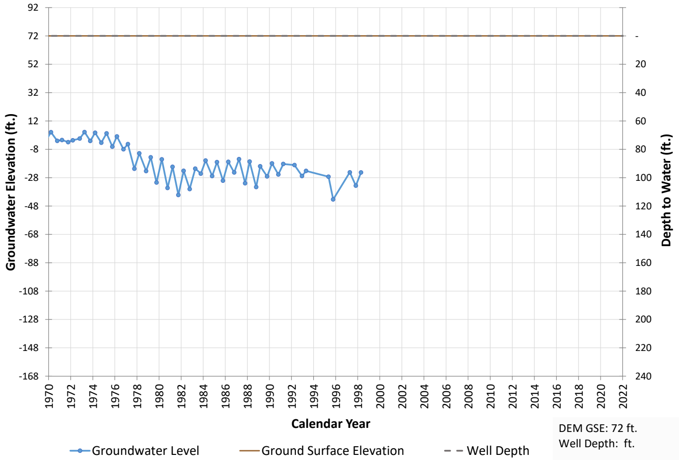
Well 593 Hydrograph
