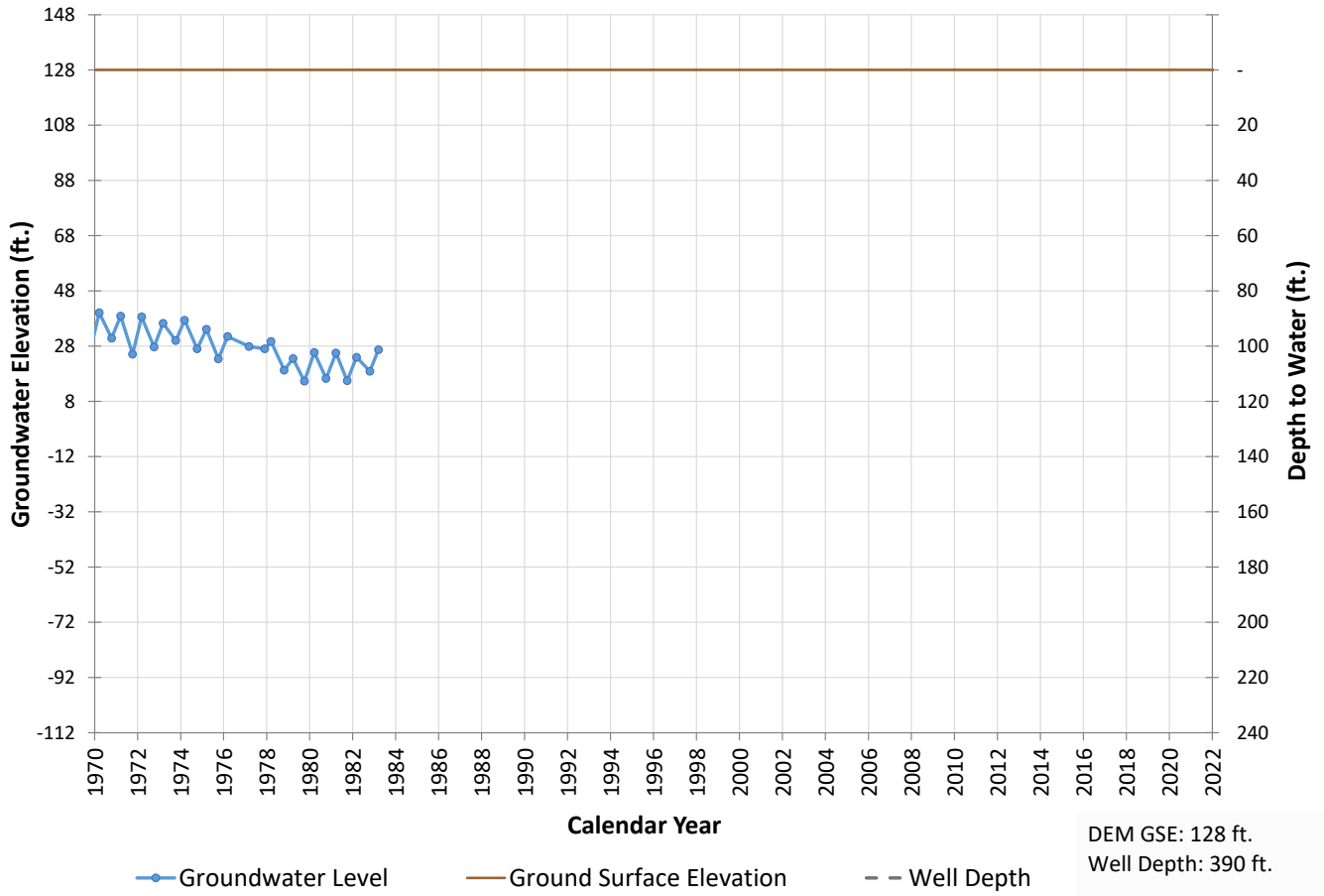
Well 287 Hydrograph
