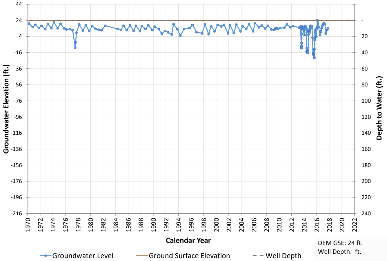
Well 696 Hydrograph
