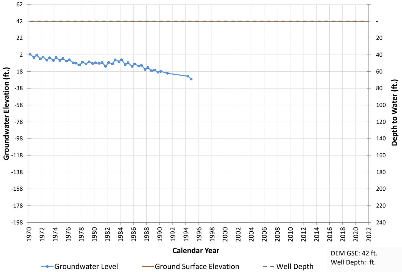
Well 455 Hydrograph
