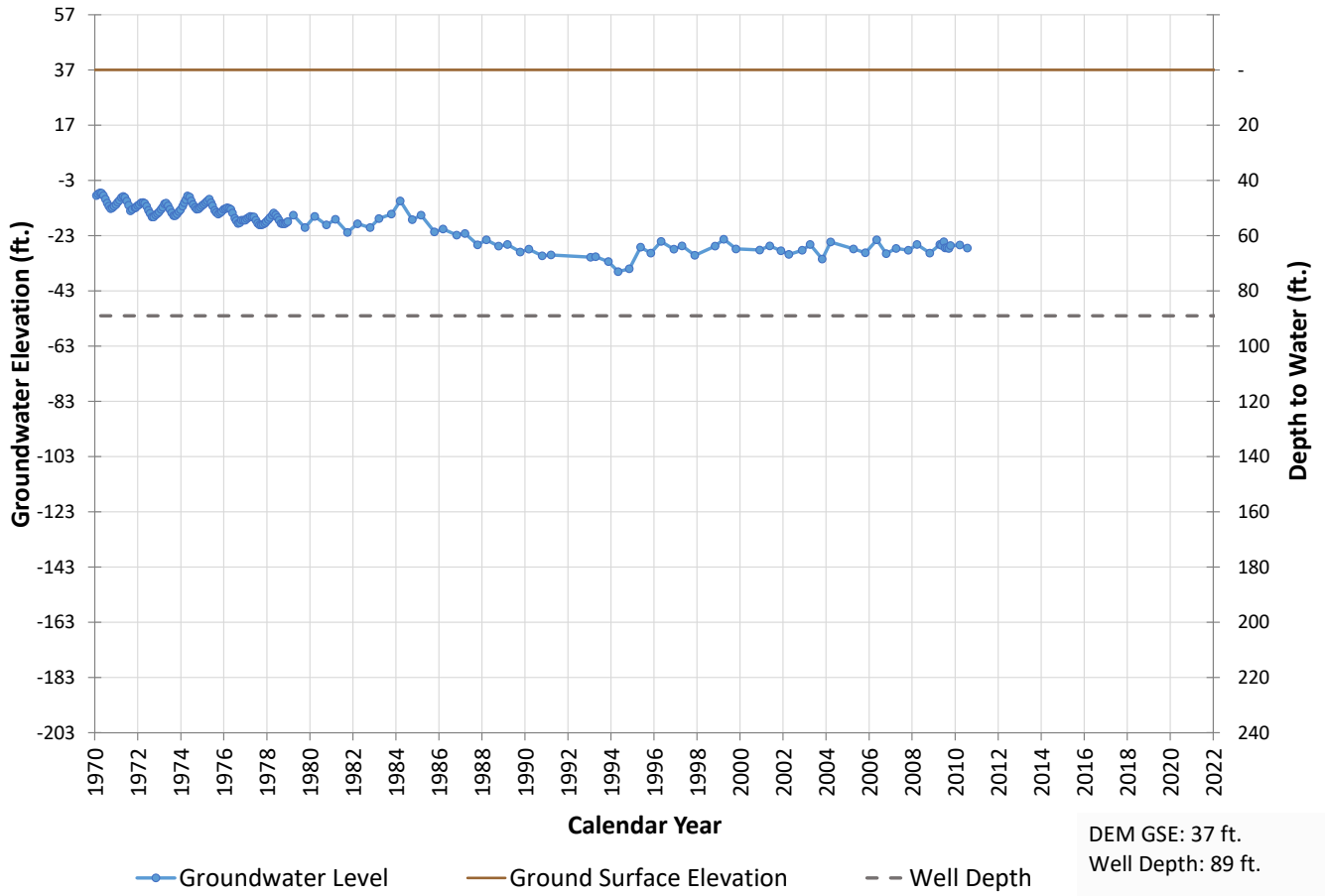
Well 367 Hydrograph
