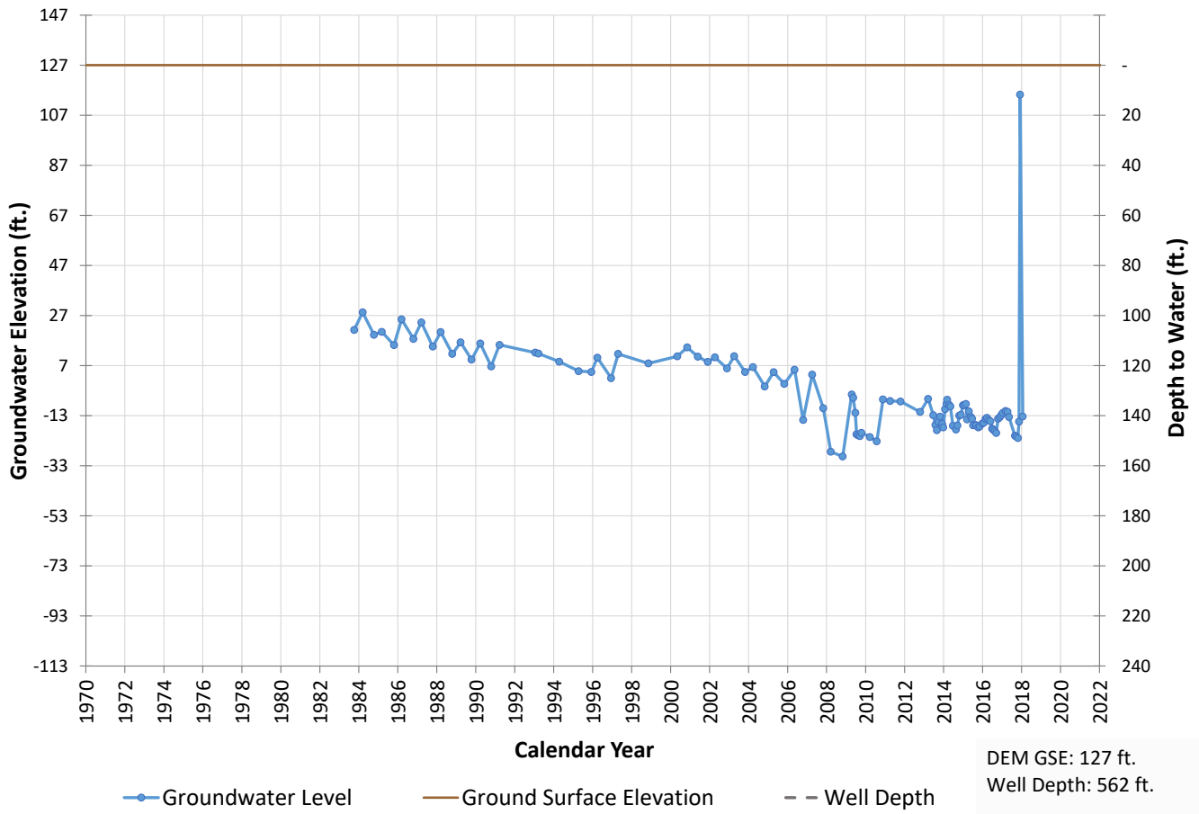
Well 289 Hydrograph
