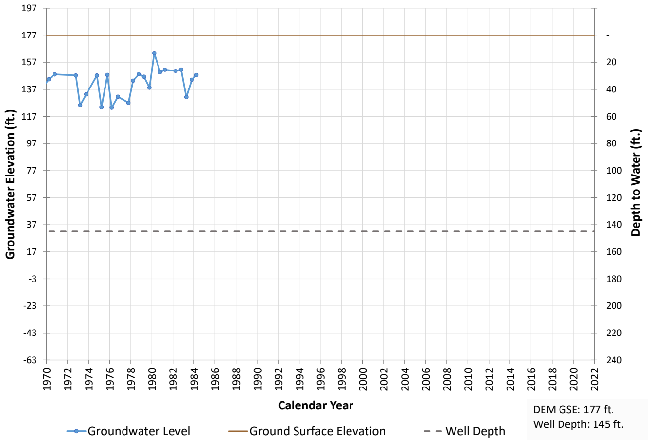
Well 774 Hydrograph
