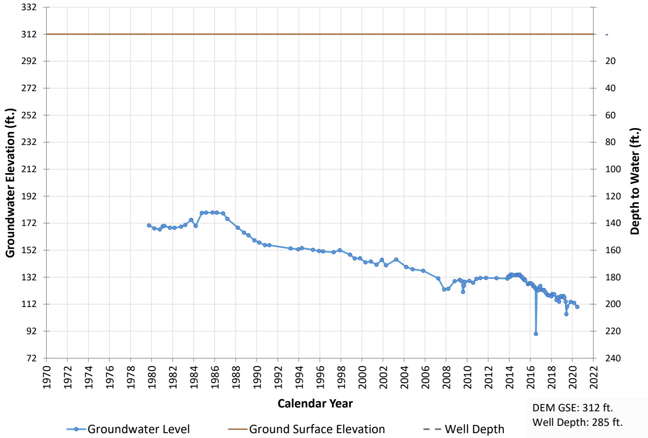
Well 319 Hydrograph
