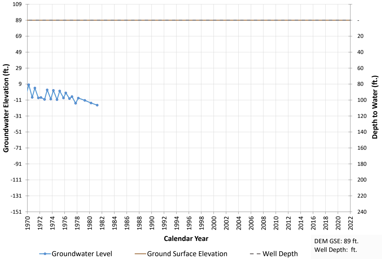
Well 533 Hydrograph
