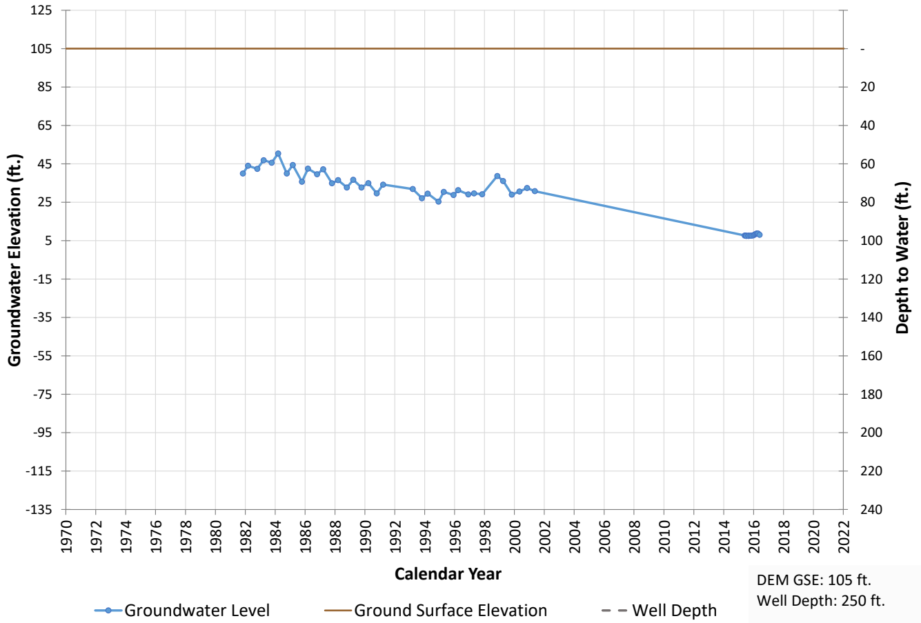
Well 357 Hydrograph
