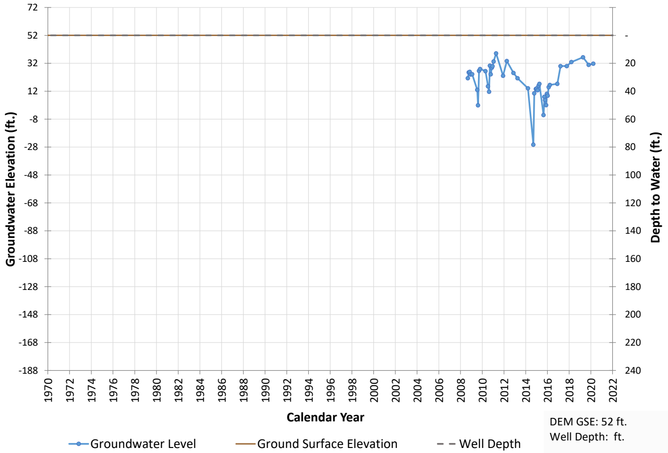
Well 805 Hydrograph
