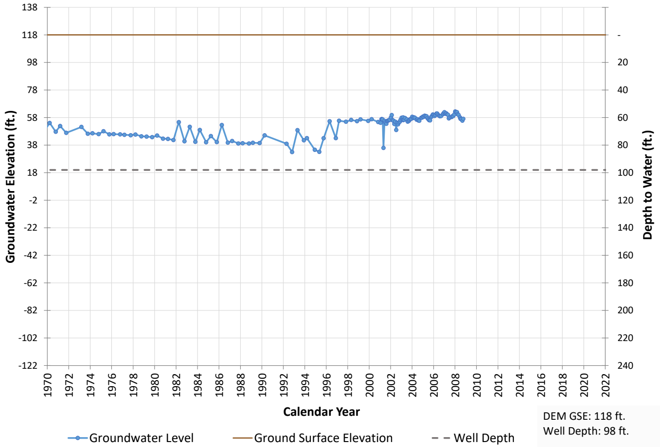
Well 650 Hydrograph
