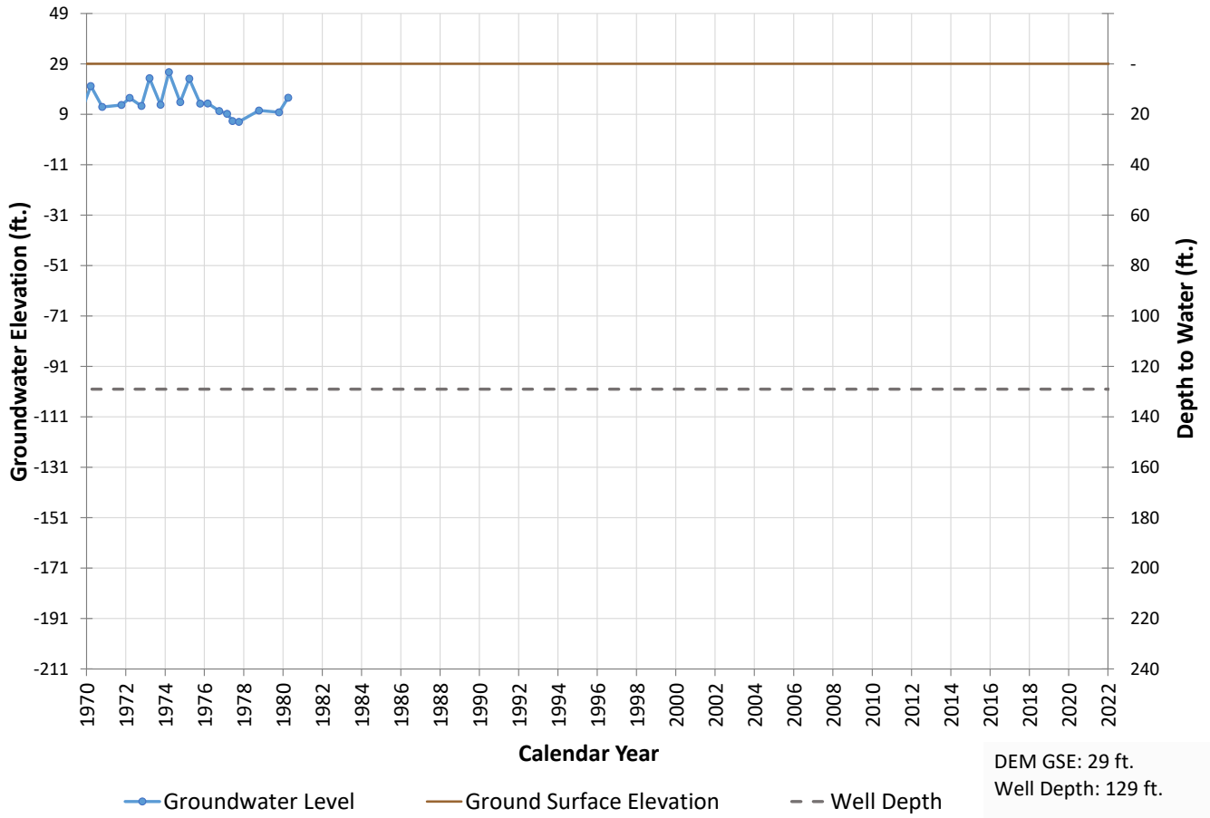
Well 607 Hydrograph
