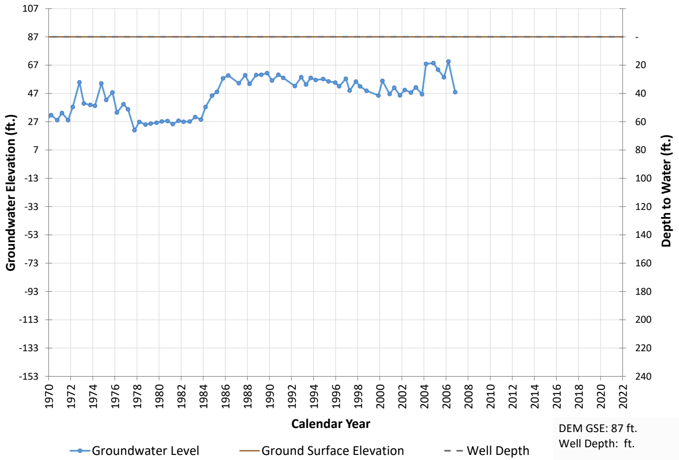
Well 628 Hydrograph
