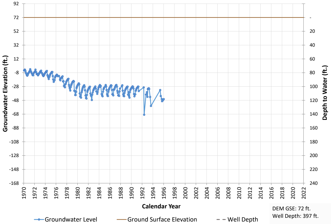
Well 568 Hydrograph
