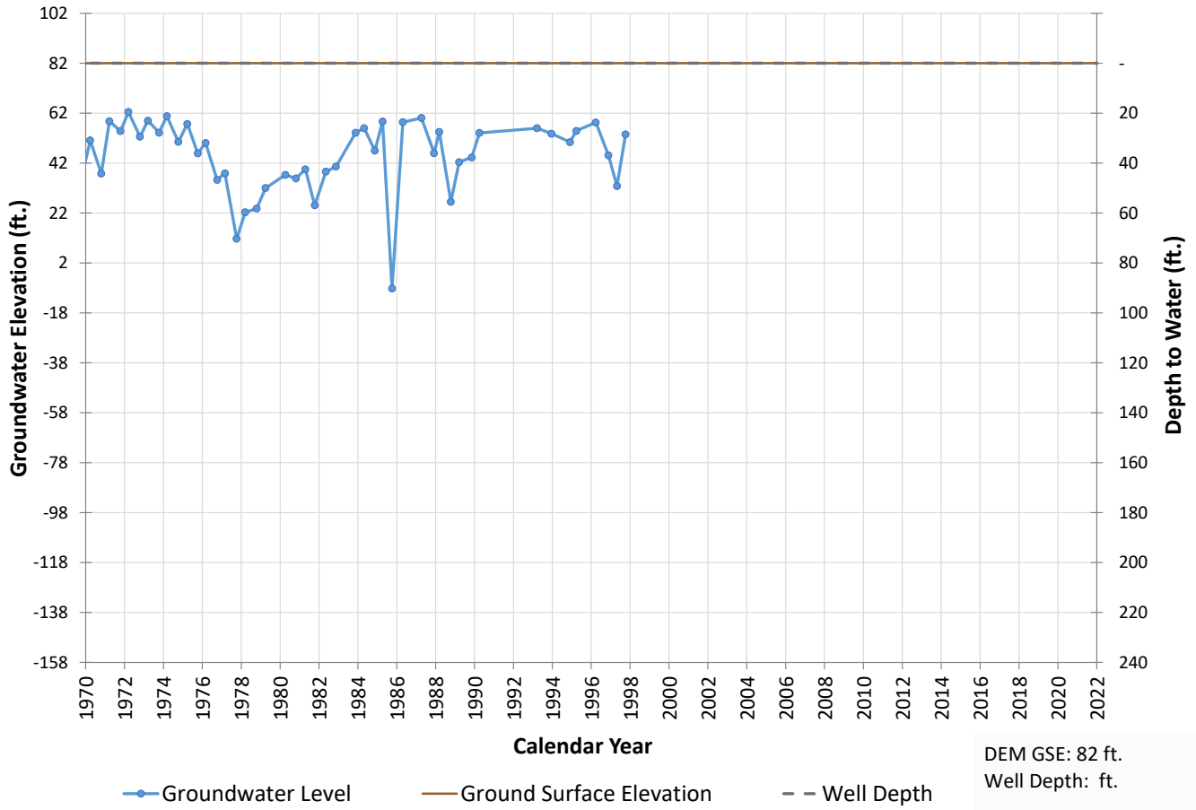
Well 813 Hydrograph
