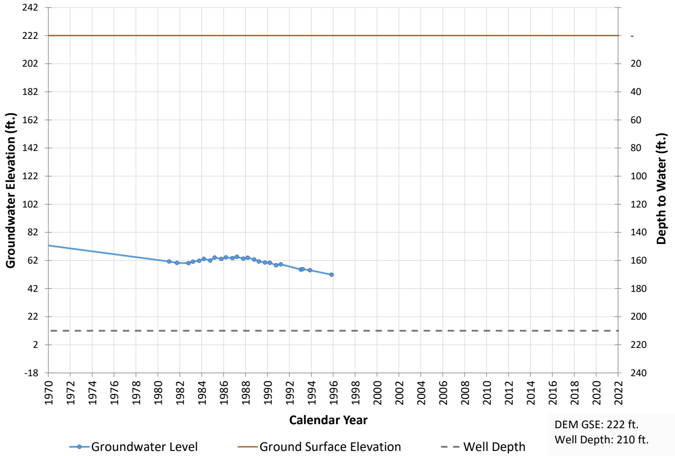
Well 278 Hydrograph
