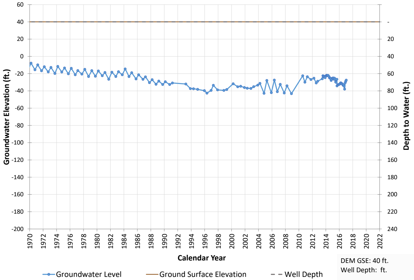
Well 356 Hydrograph
