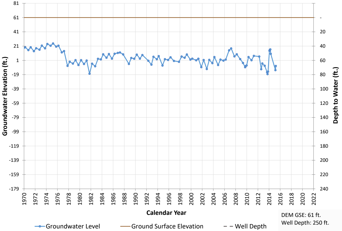
Well 694 Hydrograph
