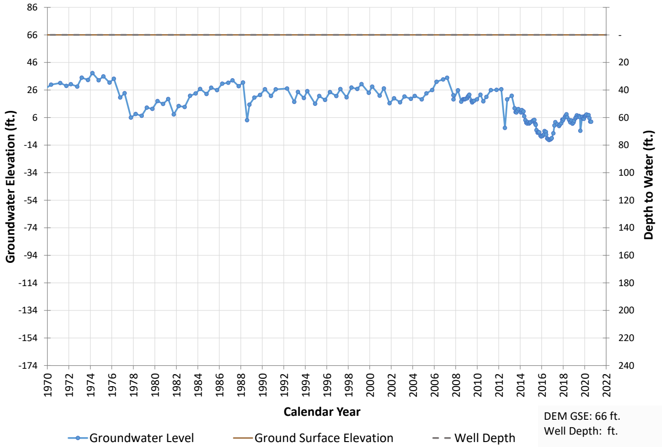
Well 735 Hydrograph
