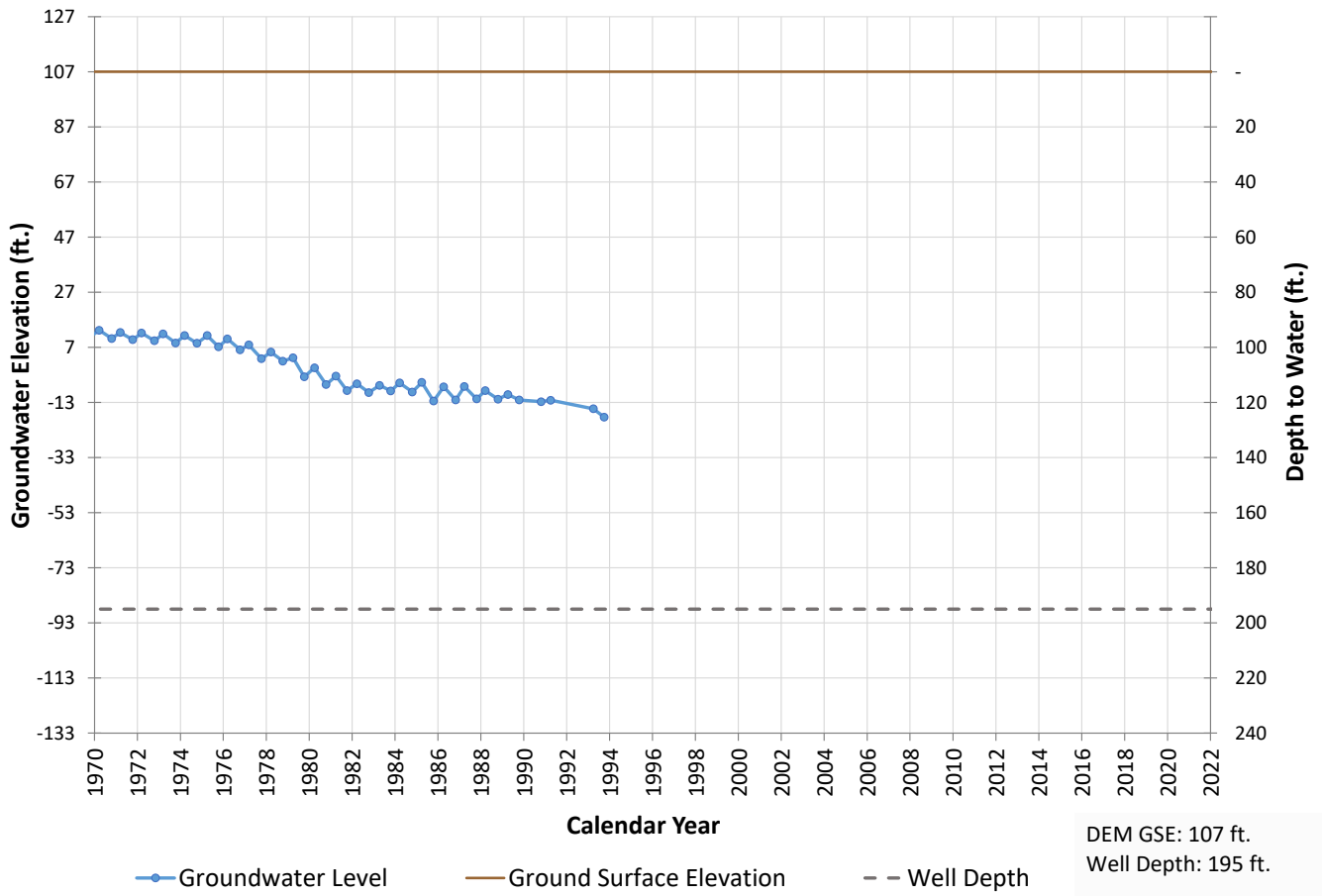
Well 587 Hydrograph
