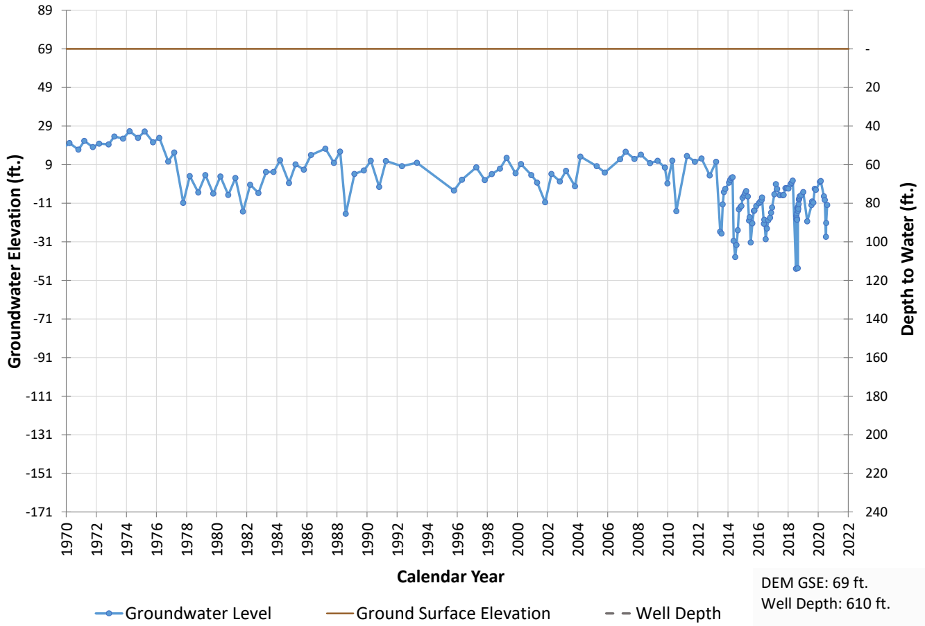
Well 717 Hydrograph
