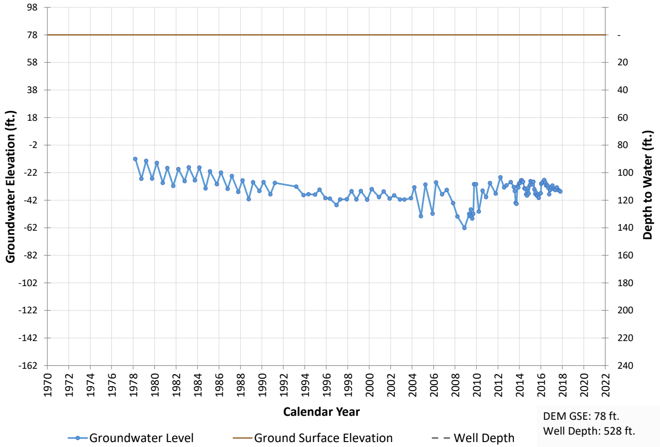
Well 431 Hydrograph
