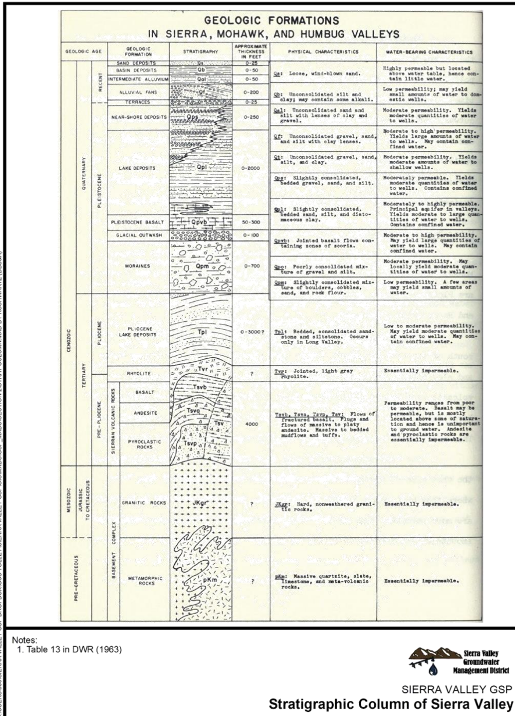
Figure 2.2.1-11: Stratigraphic Column of Sierra Valley
