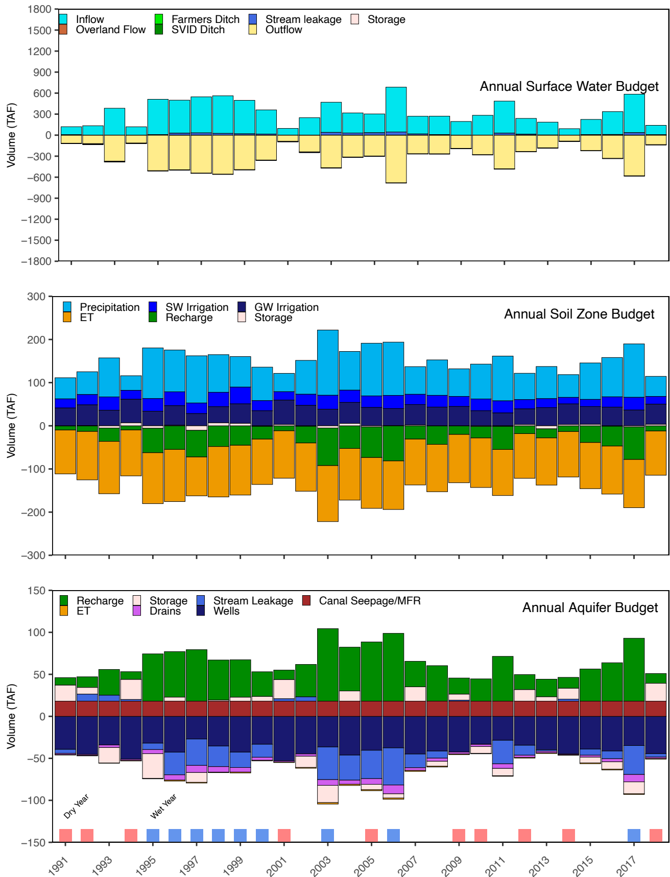
Figure 35: Annual water budgets for the three conceptual subsystems used to represent the hydrology of the Basin: the surface water system, the soil zone, and the aquifer.
