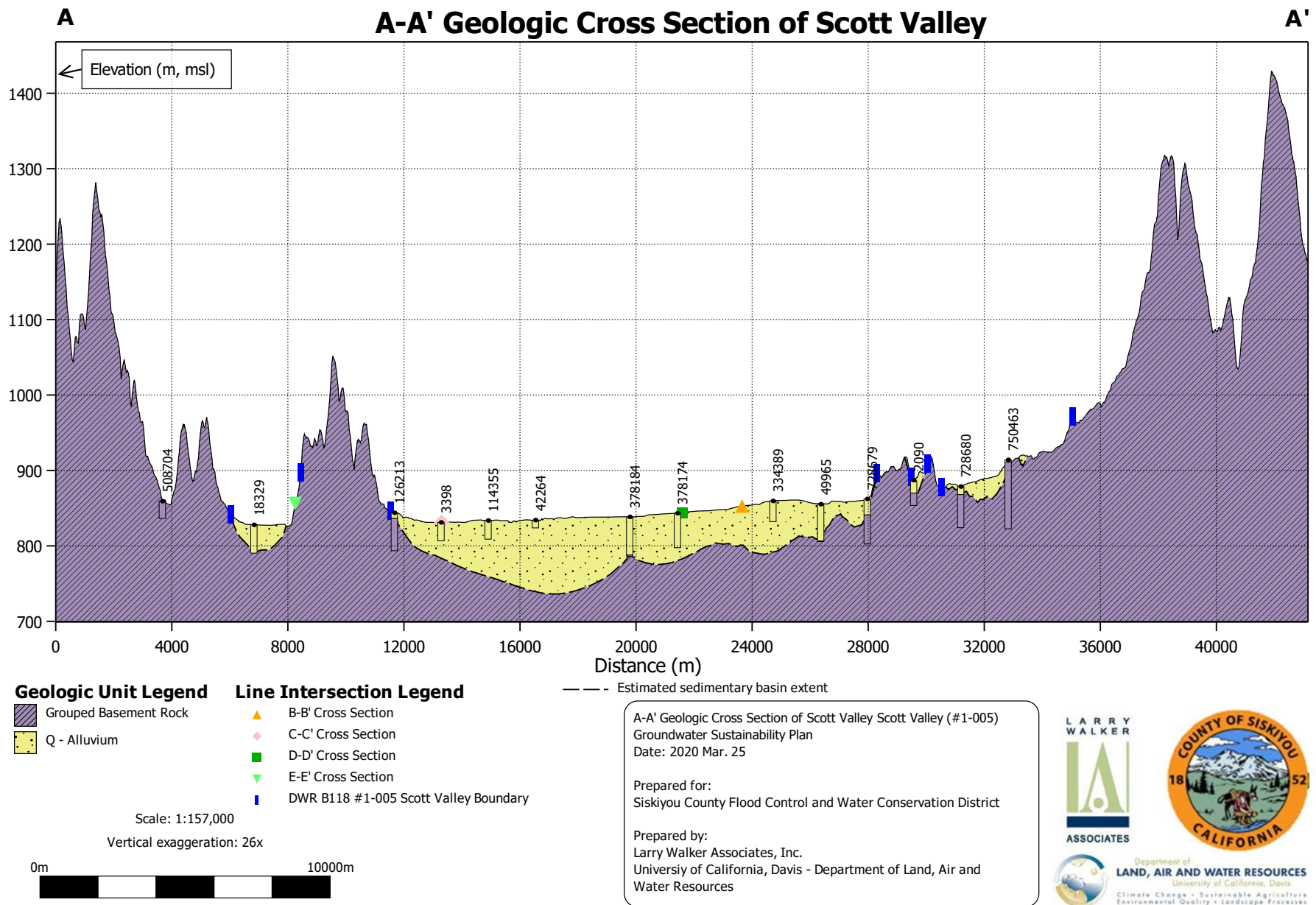
Figure 16: Scott Valley Groundwater Basin Cross Section A-A'
