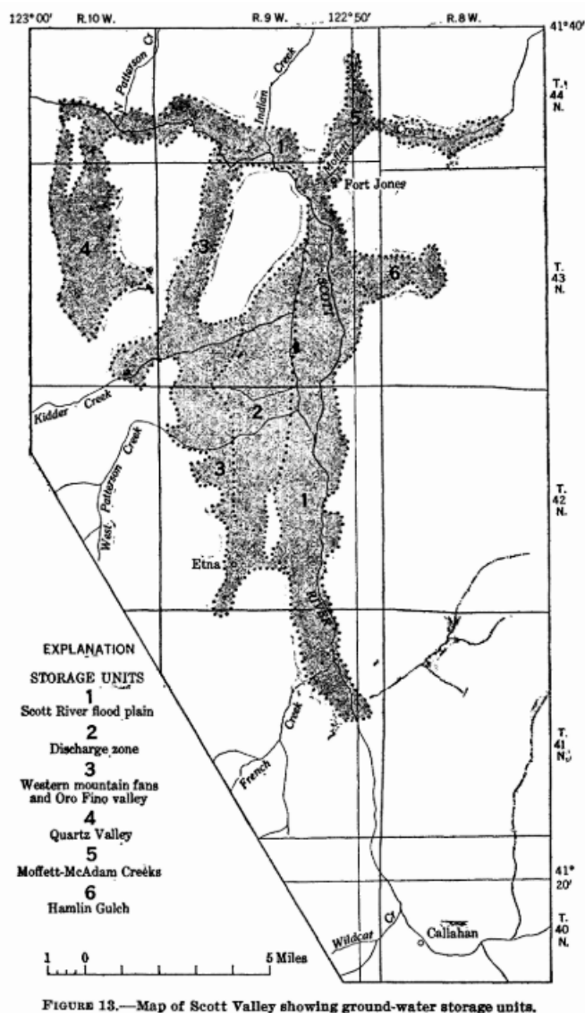
Figure 32: Scott Valley groundwater storage units, as published in Figure 13 in Mack 1958.
