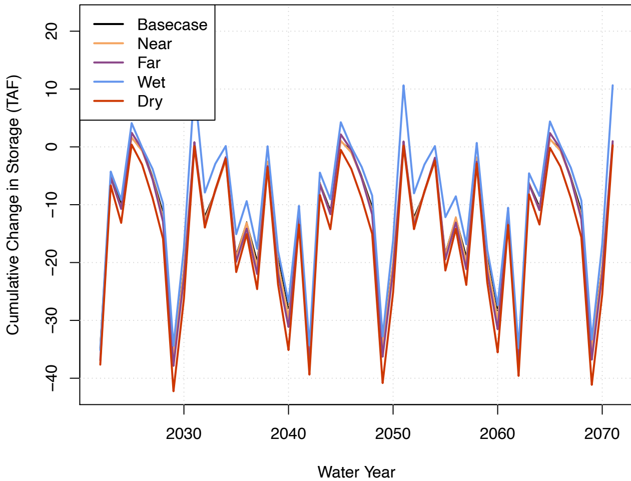
Figure 41: Cumulative groundwater storage for the future projected climate conditions, with base-case and four DWR climate scenarios.
