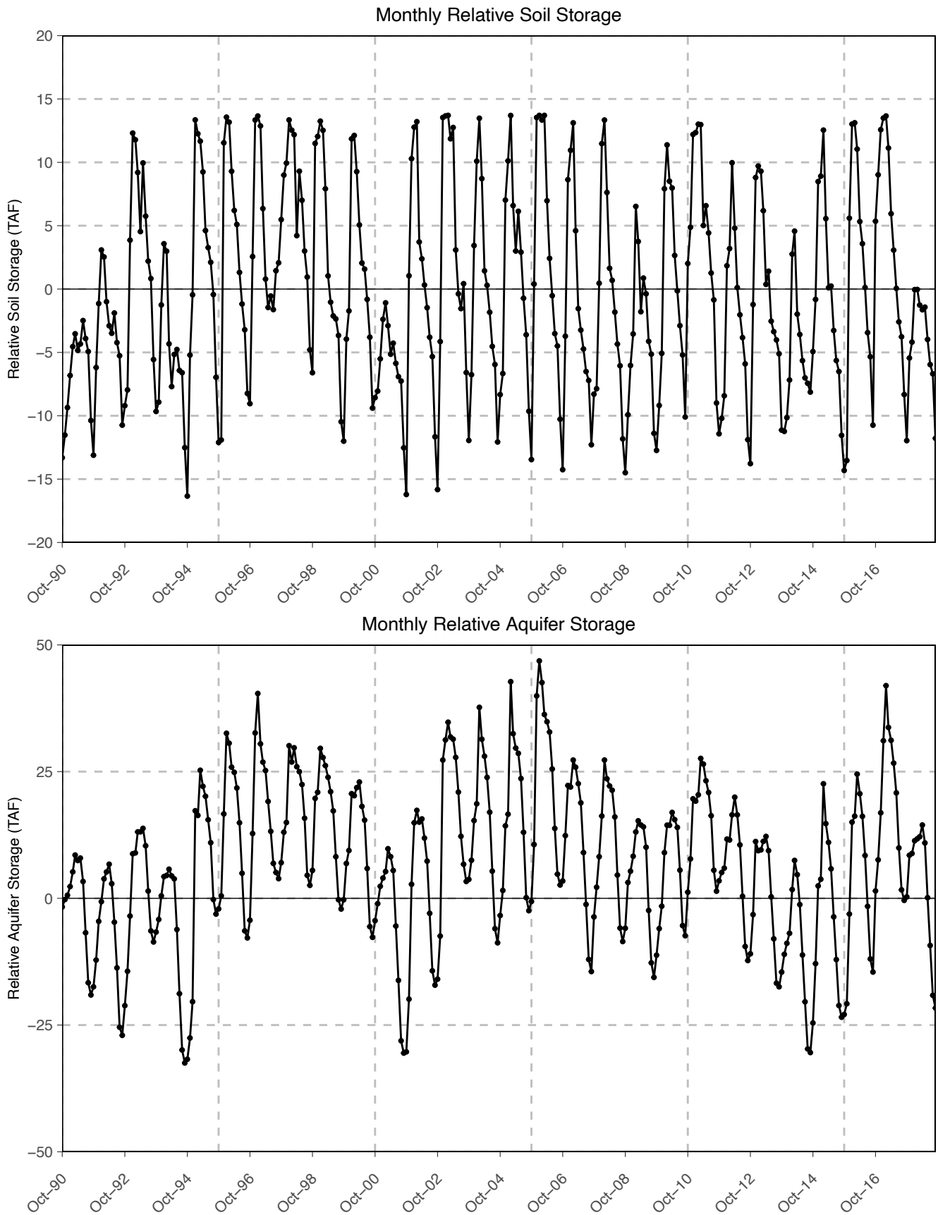
Figure 38: Monthly change in volume of water stored in the soil zone (top panel) and groundwater aquifer (bottom panel) Total storage volume and interannual variability are both greater for the aquifer than for the soil zone.
