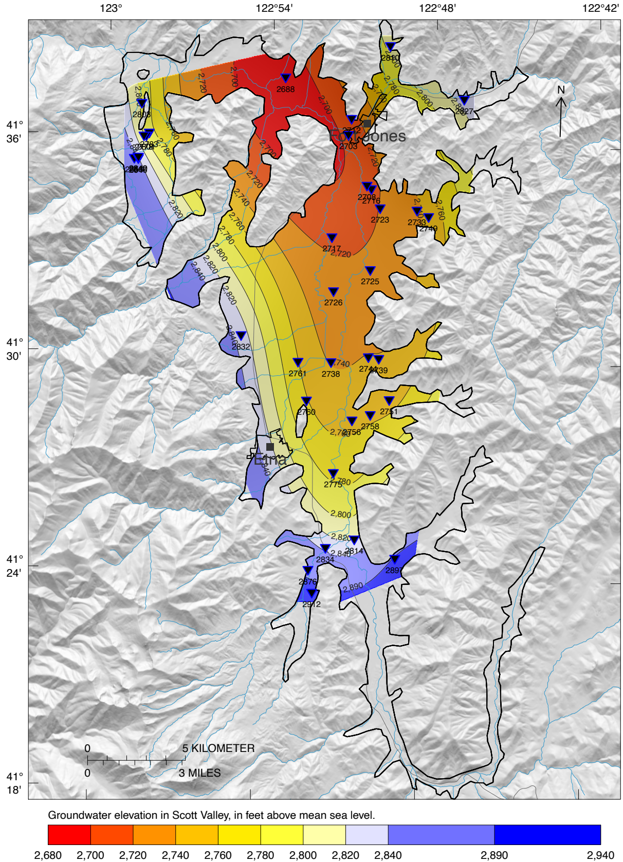
Figure 30: Scott Valley Groundwater Elevations, September 2015.
