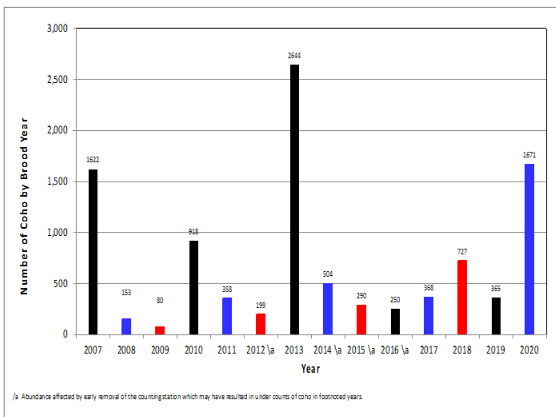
Figure 27: From Knechtle (2021), Figure 19. Estimated escapement by Brood Year of adult and grisle Coho Salmon salmon returning to the Scott River from 2007-2020. Individual Brood Years are represented by different colors.
