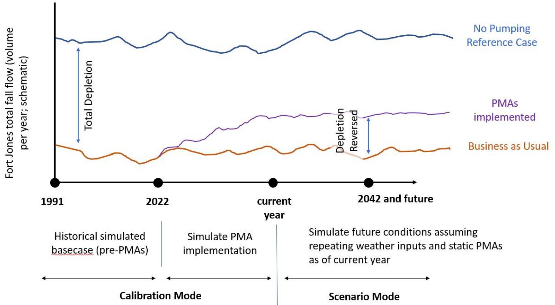
Figure 48: Visual schematic of simulations used to calculate Relative Depletion Reversal in future sustainable groundwater management reports.
