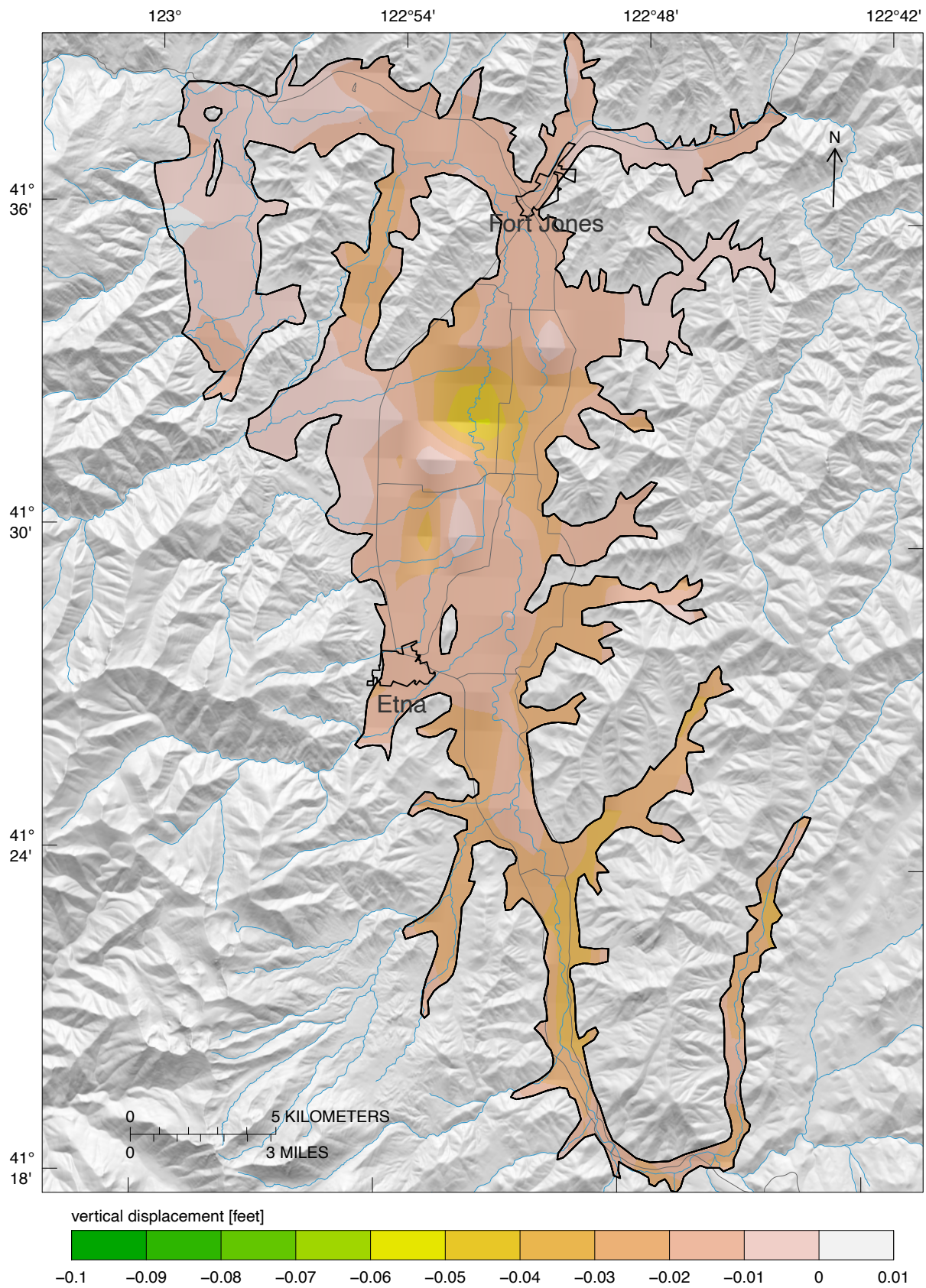
Figure 34: InSAR Total Subsidence in the SCott Valley Groundwater Basin Between June 2015 and September 2019.
