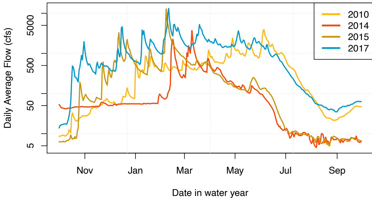
Figure 21: Streamflow record at the Fort Jones USGS Stream Gauge (11519500) from 1937 through 2019. Water years shown are examples of wet and dry years (2017 and 2014, respectively), and two years which received average total annual rainfall (2010 and 2015).
