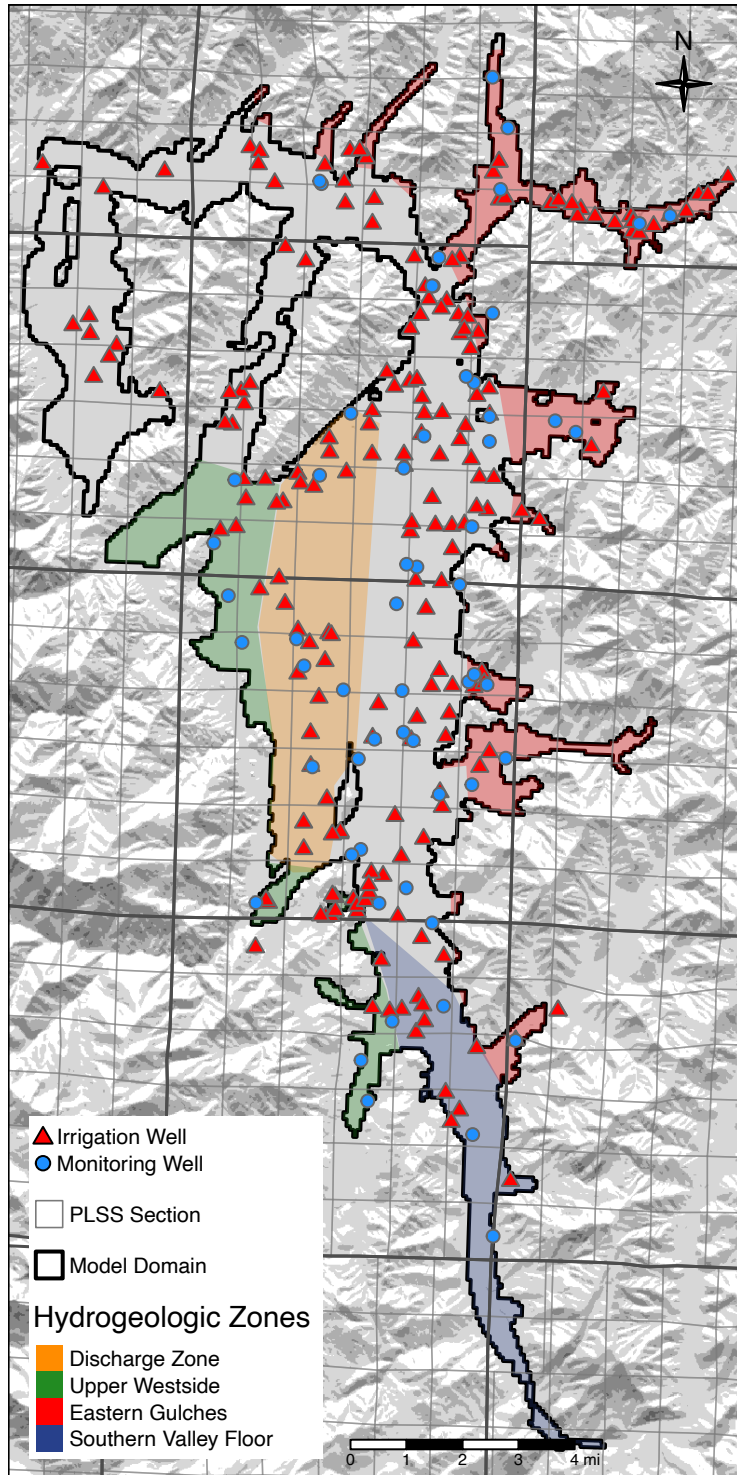
Figure 37: The model domain boundary and wells used in the SVIHM simulation of Basin hydrology. Additionally, generalized hydrogeologic zones (adapted from Mack, 1958) are shown. These areas represent general zones in which observed water level records tend to have similar characteristics (e.g., seasonal variability and overall depth to water). For more information see selected hydrographs in Section 2.2.2.1, the full hydrographs collection in Appendix 2-C, and Tolley et. al 2019.
