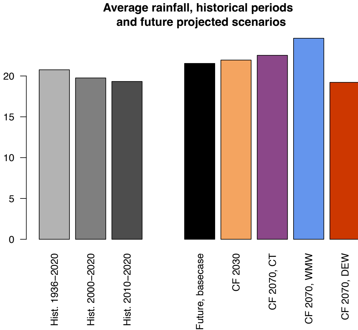
Figure 40: Historical rainfall for three selected periods (1936-2020, 2000-2020, and 2010-2020, with 20.8, 19.8 and 19.3 inches respectively) demonstrate that conditions in the last 10 years have been drier than the last 20, which have been drier than the full record period since 1936. The basecase and three of the four future scenarios exceed the historic averages, while the DEW (Dry) future scenario (19.2 inches) is on par with the average of the last 10 years (19.3 inches).
