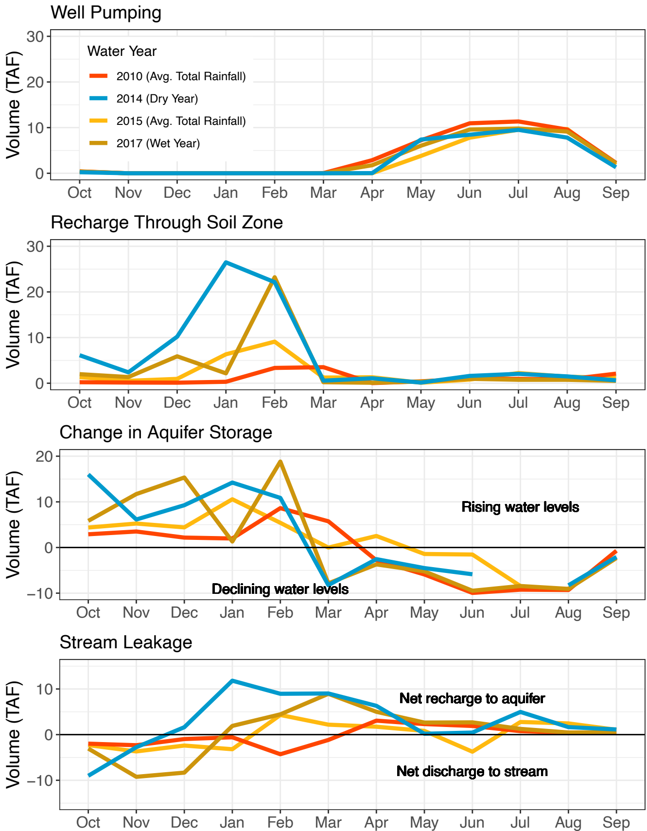
Figure 36: Monthly values of selected water budget components in 4 example water years.
