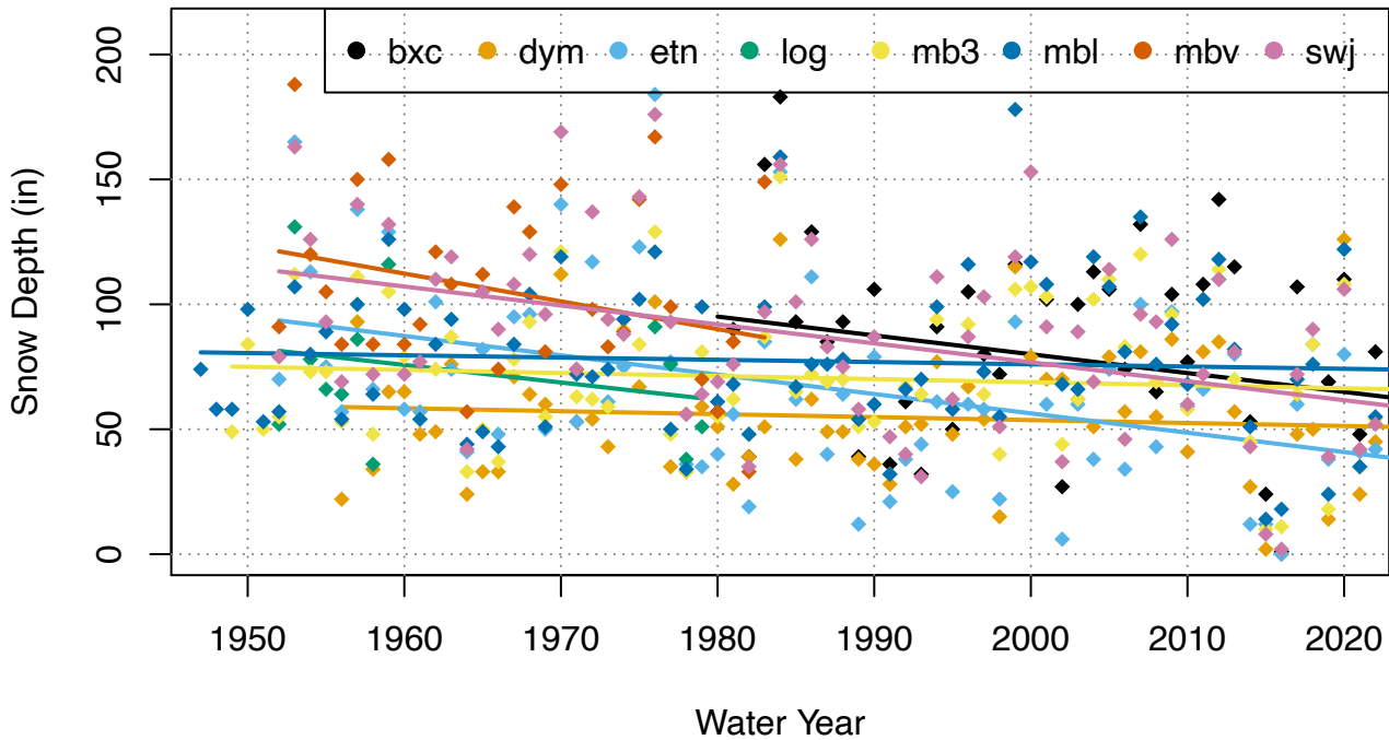
Figure 13: Annual maximum snow depth measured at eight California Data Exchange Center (CDEC) snow stations in the Scott Valley watershed. For more information see table below.
