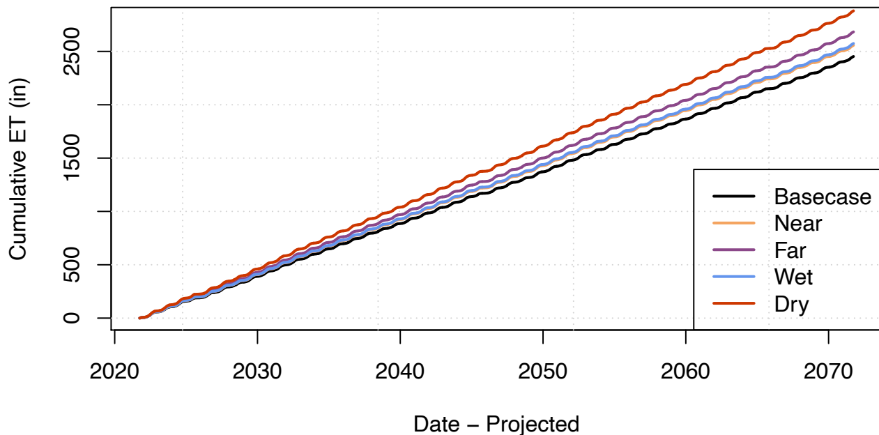
Figure 39: Cumulative precipitation and reference ET for the future projected climate conditions, with basecase and four DWR climate scenarios. The 2030 (Near) and 2070 central tendency (Far) scenarios predict similar rainfall conditions to the Basecase, while the 2070 DEW (Dry) and 2070 WMW (Wet) scenarios show less and more cumulative rain, respectively. Conversely, all scenarios predict higher future ET than the Basecase.
