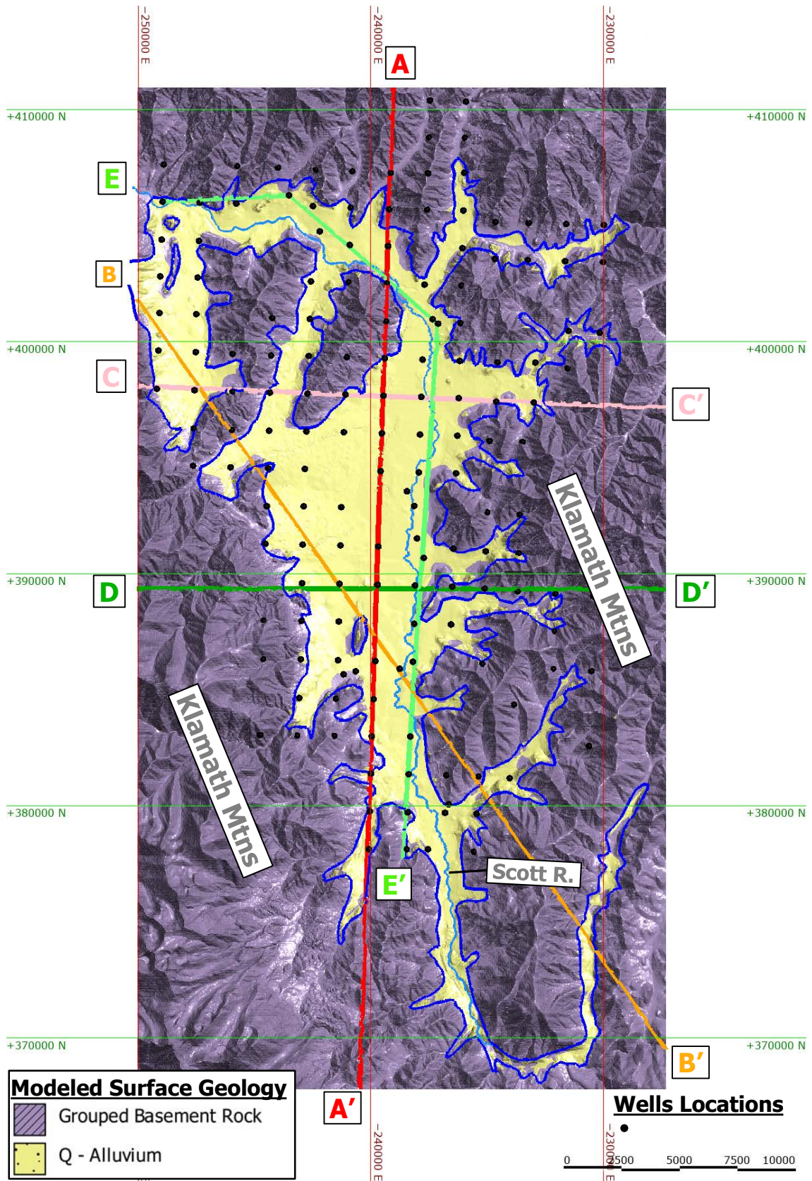
Figure 15: Scott Valley Groundwater Basin Map of Cross Section Locations'
