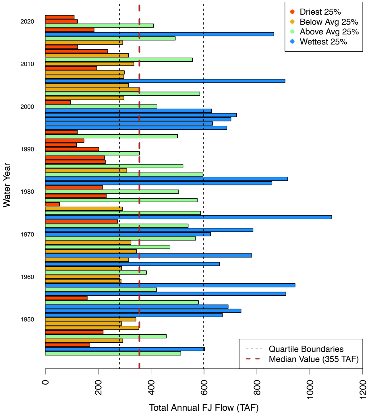
Figure 20: Total annual flow recorded at the Fort Jones USGS Stream Gauge (11519500) from water year 1942 through 2021. The median value for the record 1941-2021 is indicated as a dashed brown line at 355 TAF per year; the boundaries between the other quartiles are shown as dashed black lines at 280 and 598 TAF per year.
