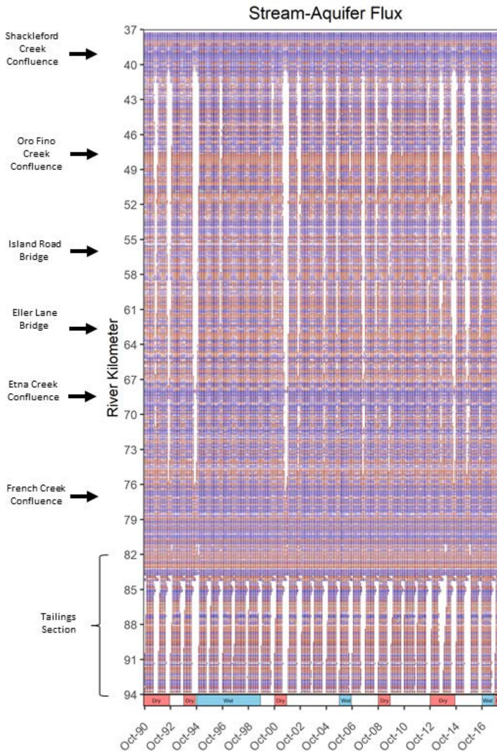
Figure 25: Spatiotemporal heat map of simulated flowrates between groundwater and surface water for the Scott River with geographic locations noted. After Tolley 2019.
