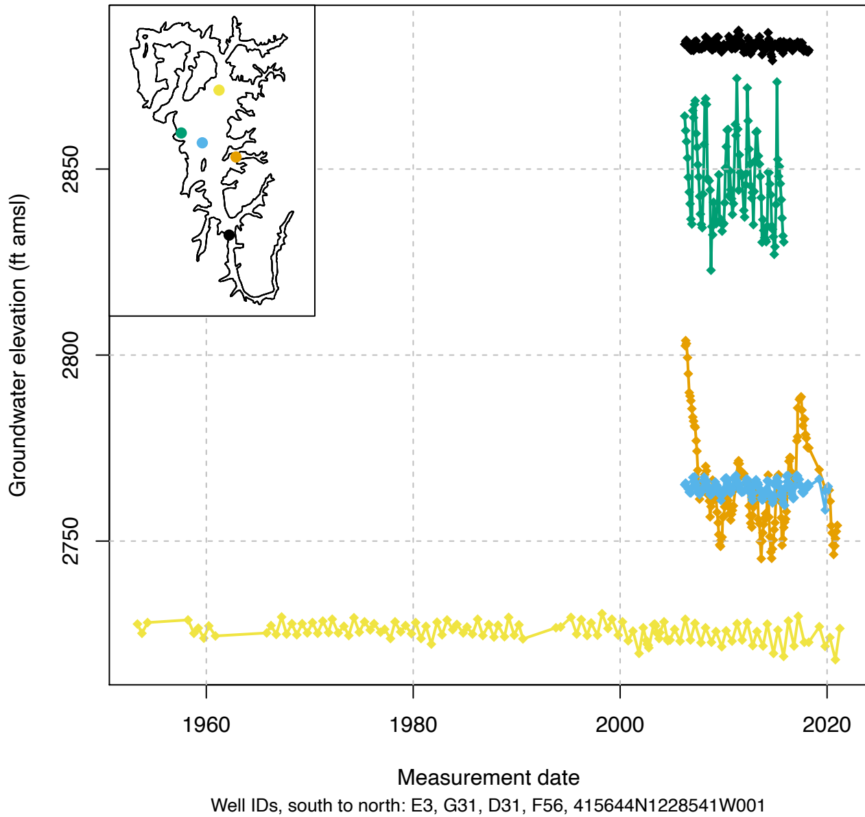
Figure 31: Selected long-term groundwater elevation measurements over time in five wells, one located in each hydrogeologic zone of the Scott Valley Groundwater Basin.
