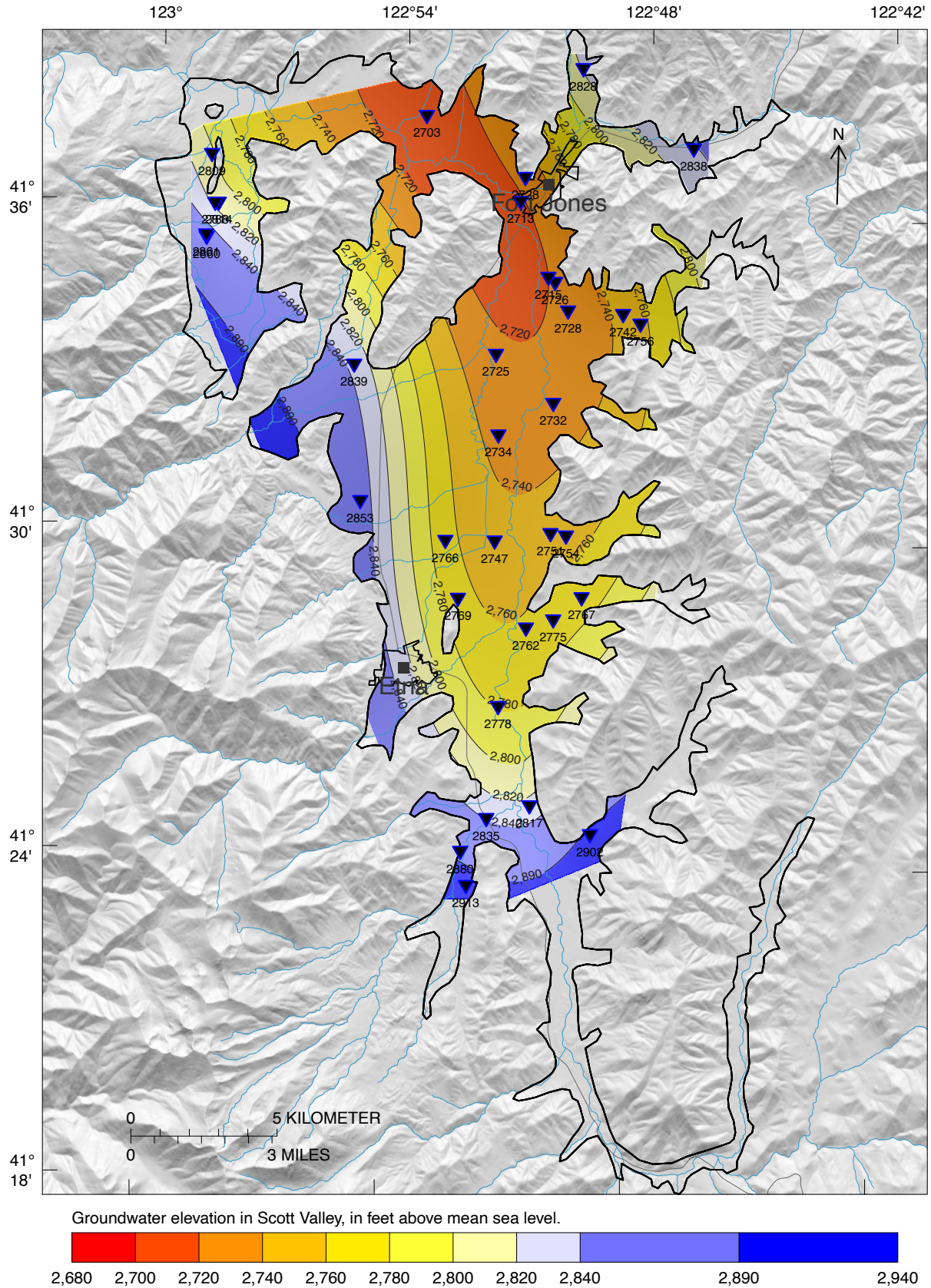
Figure 29: Scott Valley Groundwater Elevations, March 2015.
