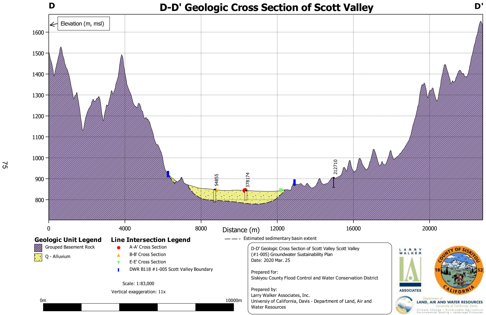
Figure 17: Scott Valley Groundwater Basin Cross Section D-D'
