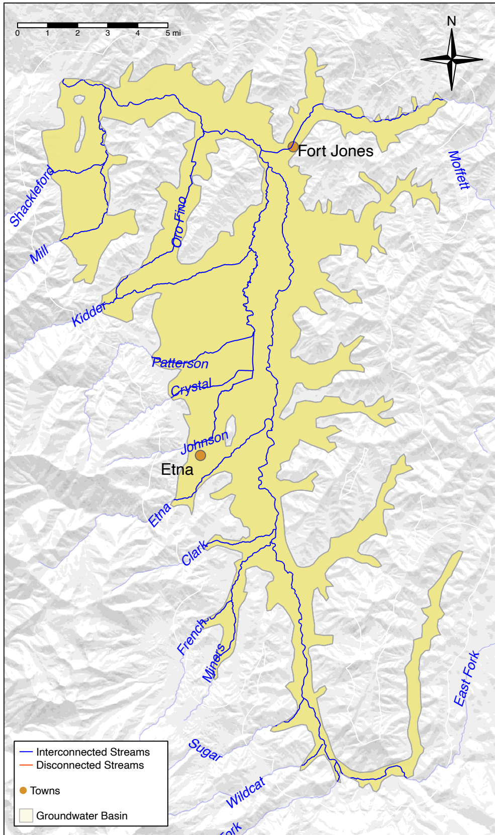
Figure 24: Interconnected Surface Waters (ISWs) in the Scott Valley. All surface water reaches overlying the Scott Valley groundwater basin have been designated as ISWs for purposes of this GSP.
