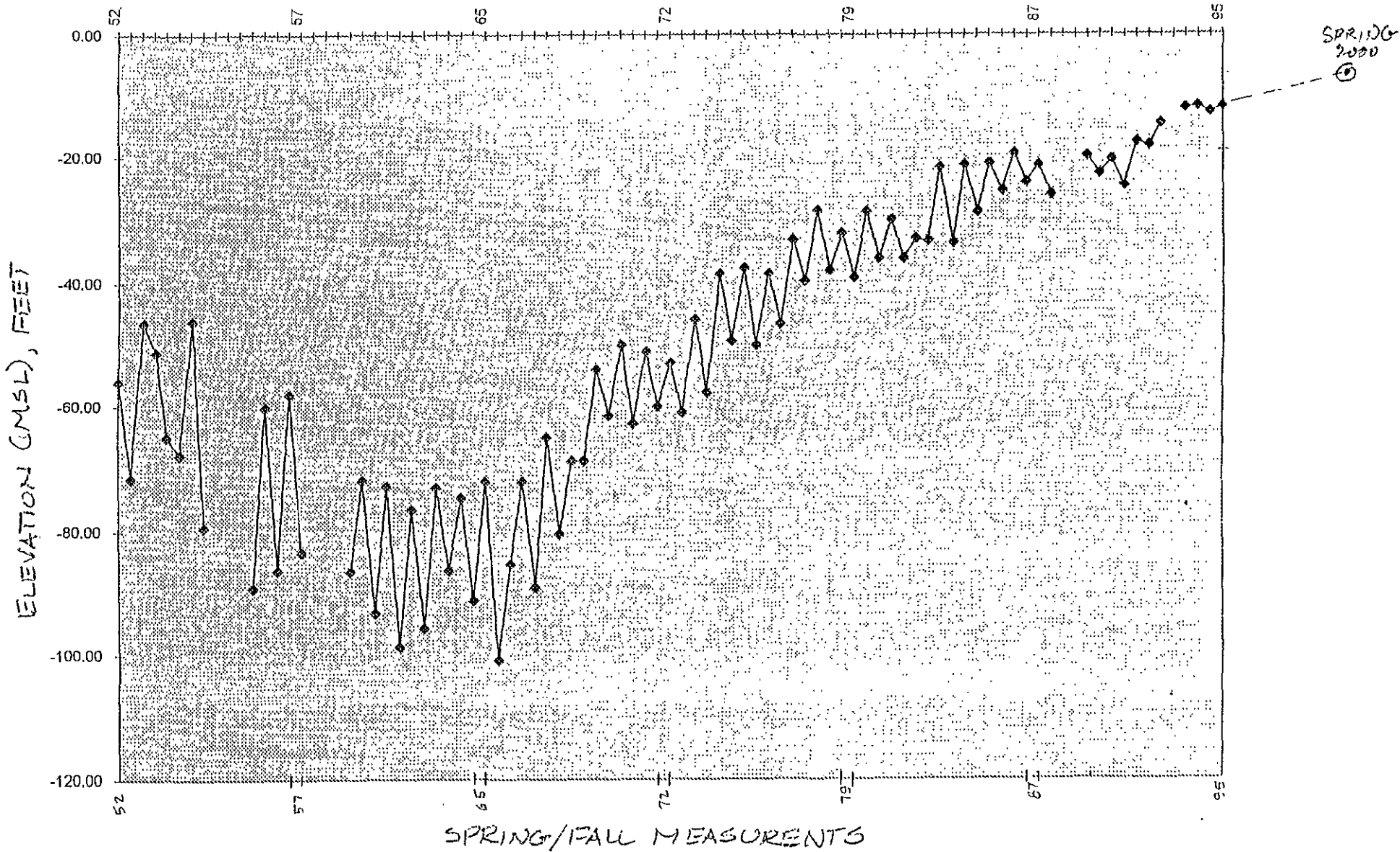
FIGURE 9. FLUCTUATIONS OF WATER LEVELS IN DEEP ZONE
