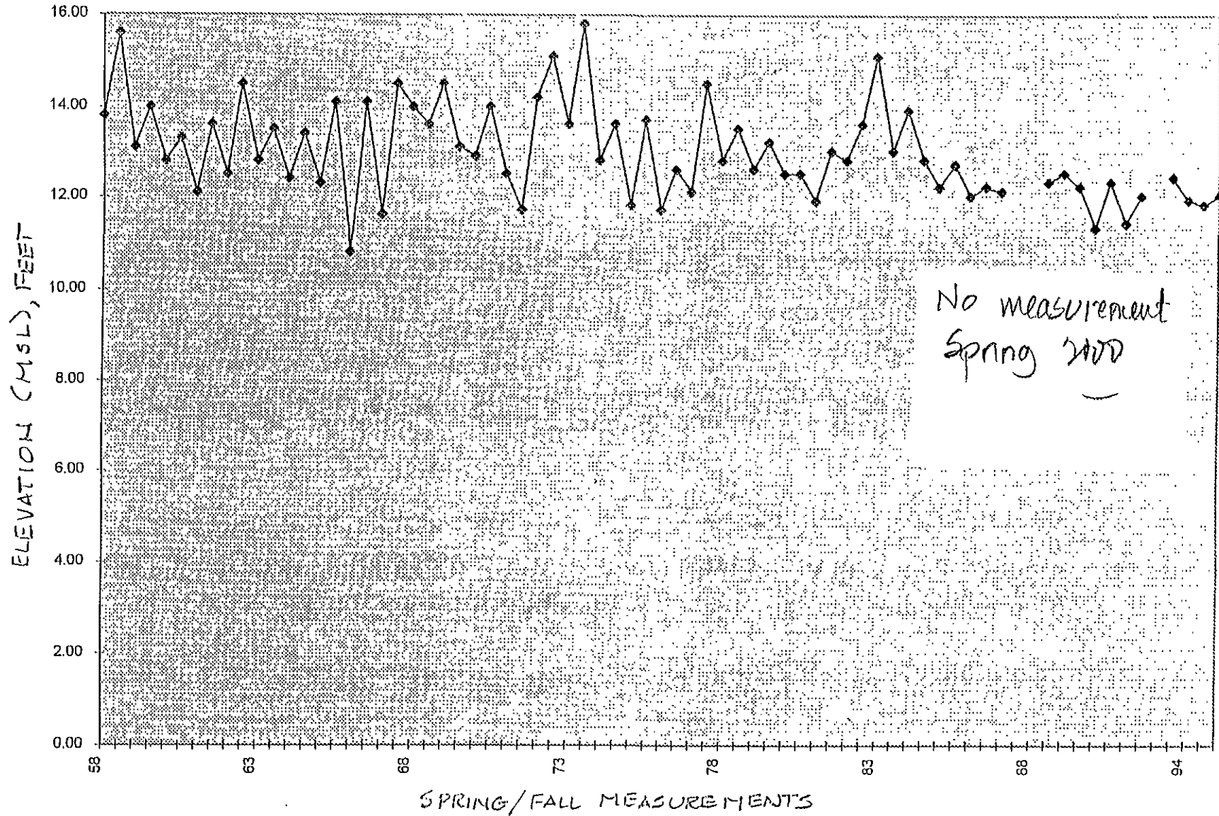
FIGURE 5. FLUCTUATIONS OF WATER LEVELS IN SHALLOW ZONE
