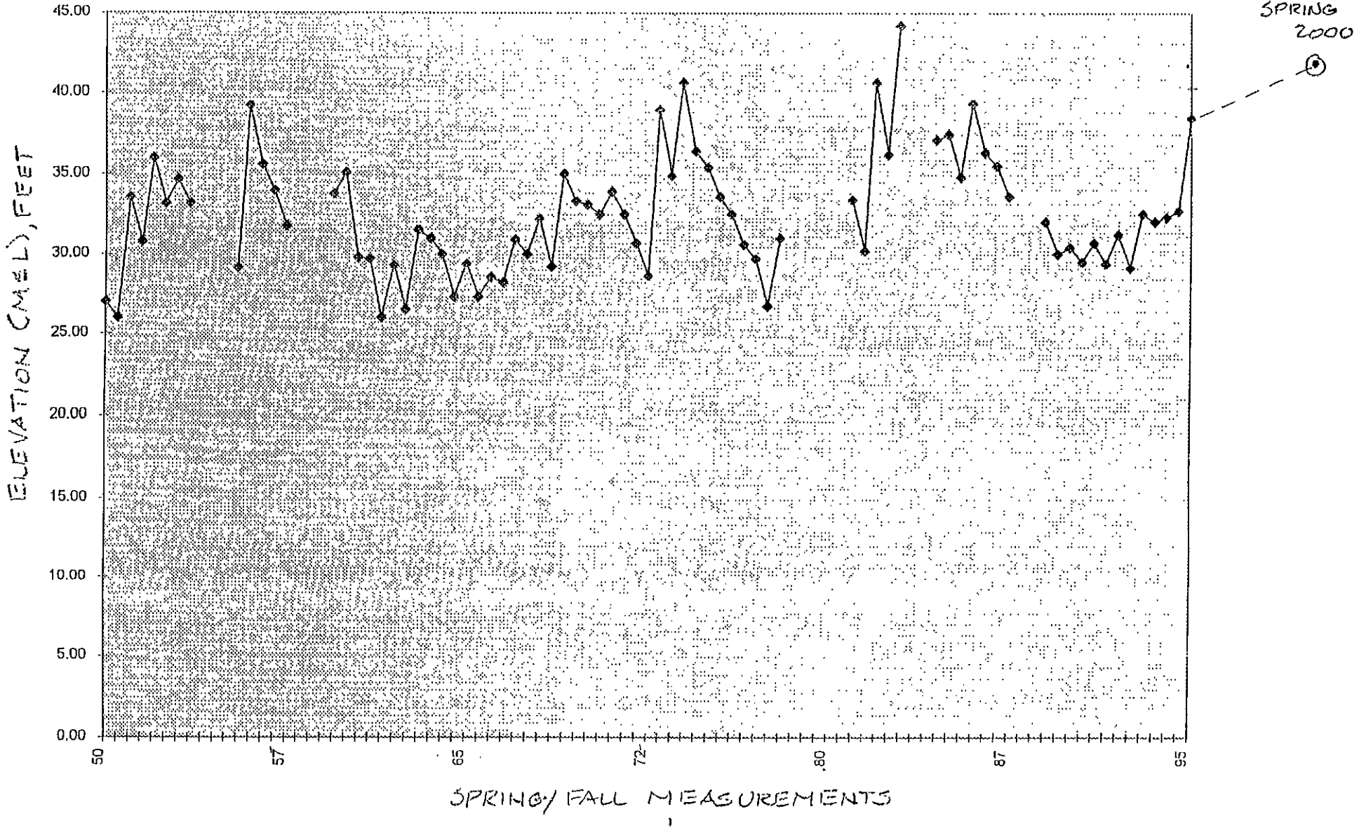
FIGURE 6. FLUCTUATIONS OF WATER LEVELS IN SHALLOW ZONE
