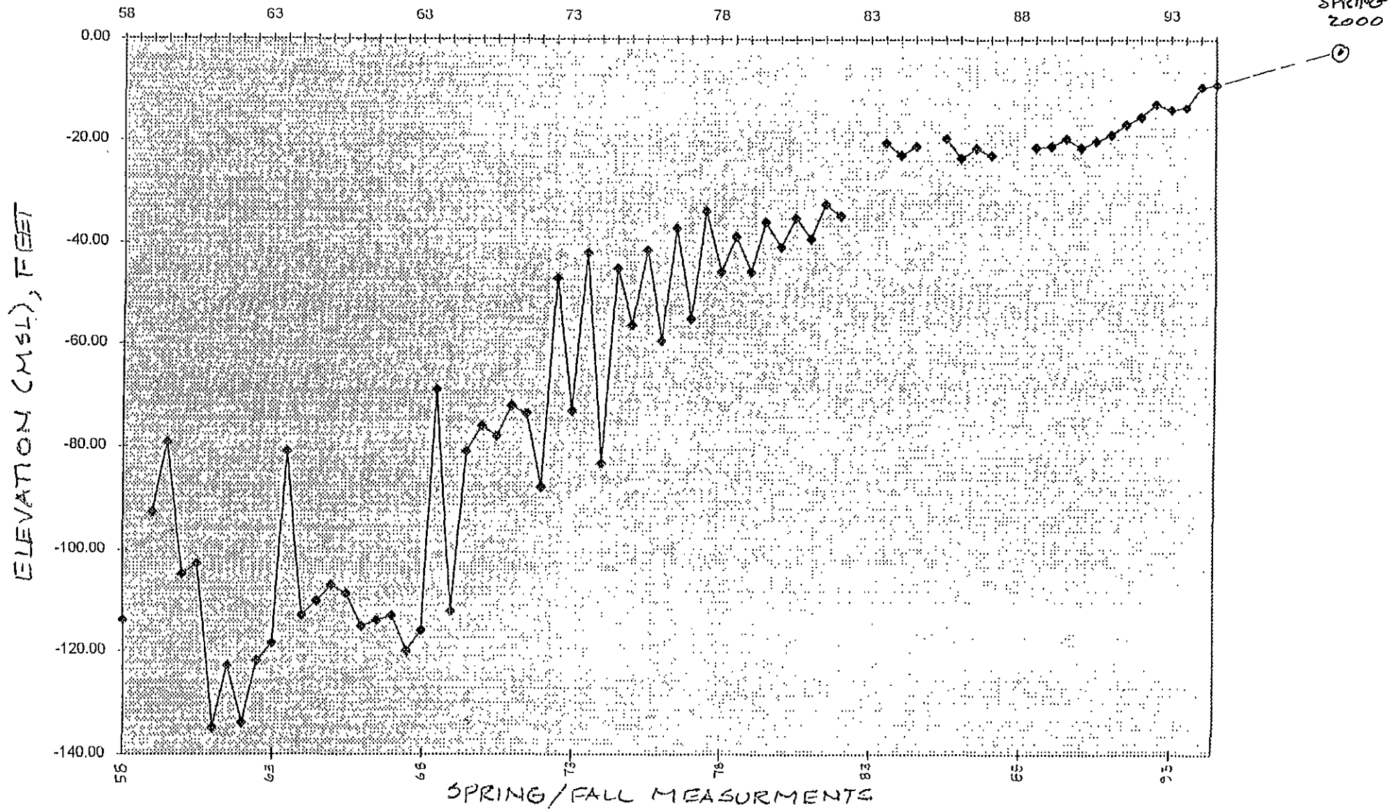
FIGURE 10. FLUCTUATIONS OF WATER LEVELS IN DEEP ZONE
