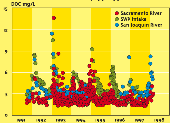
Time series showing similar timing and magnitude of peaks at SWP intake and major Central Valley rivers. Source: Data from DWR
