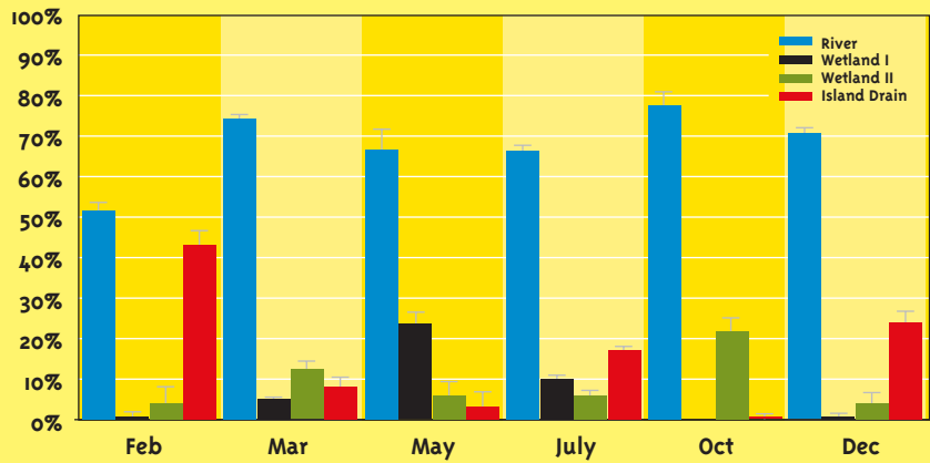
Samples taken from rivers, island drains and large, well-developed wetlands in the Delta. Source: Kraus, Bergamaschi, et al., USGS
