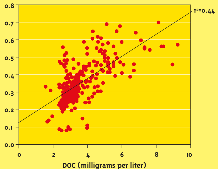
The variability in the quantity of DOC only explains 44% of the variability in THM formation — underscoring the differences in the quality of organic carbon. Source: Data from DWR
