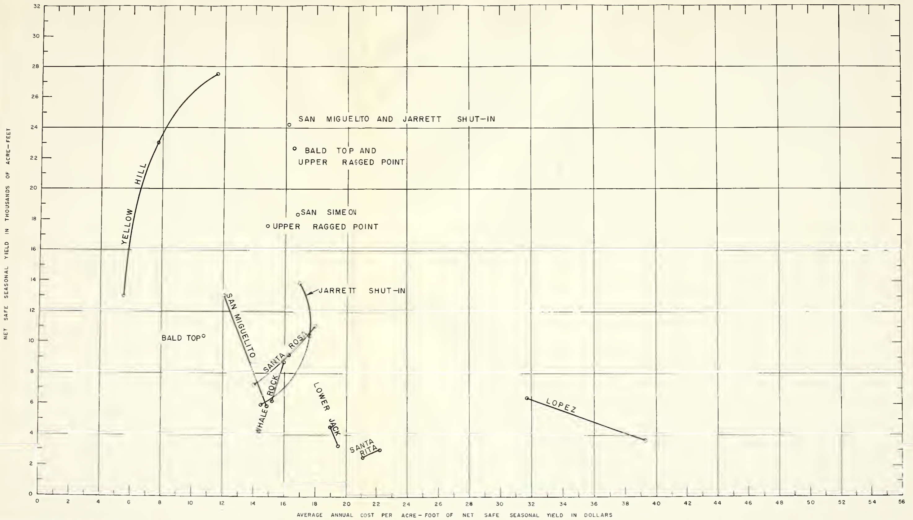
RELATIONSHIP BETWEEN NET SAFE SEASONAL YIELD OF RESERVOIRS AND ANNUAL UNIT COST
