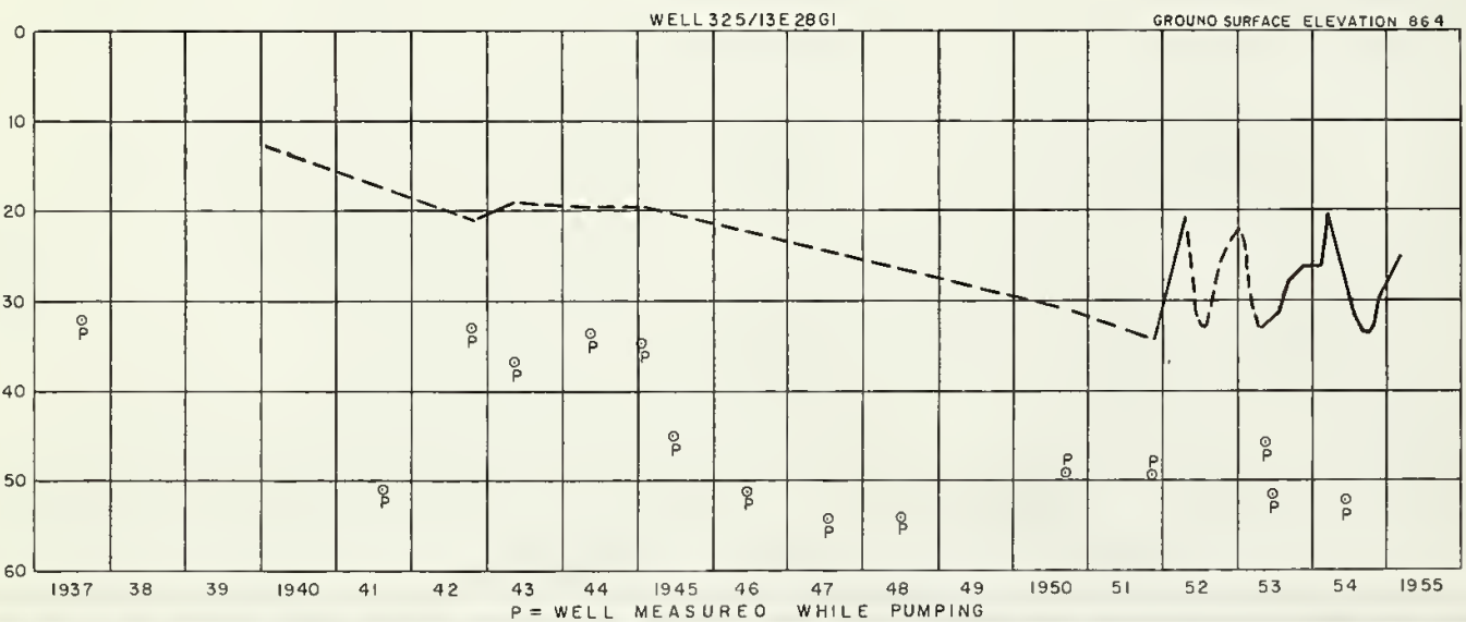
FLUCTUATION OF WATER LEVELS AT SELECTED WELLS
