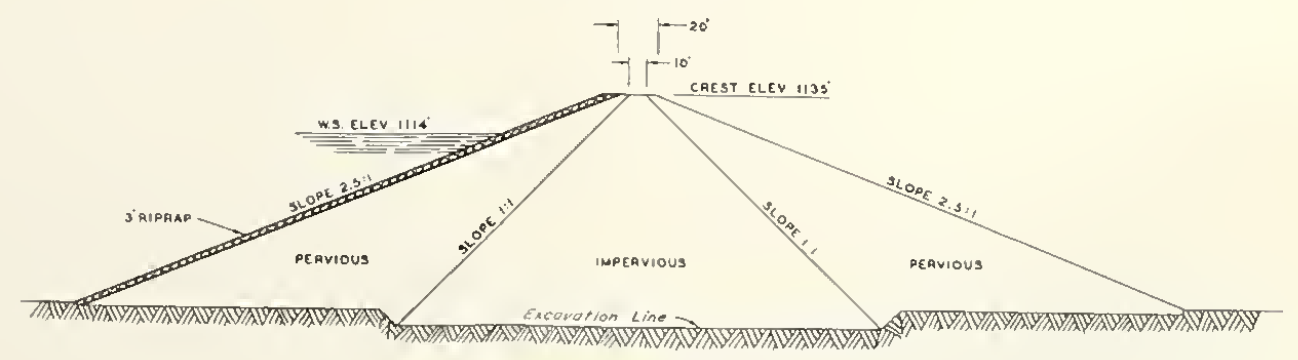
SECTION OF DAM SCALE OF FEET 0 50 100 SADDLE DAM
