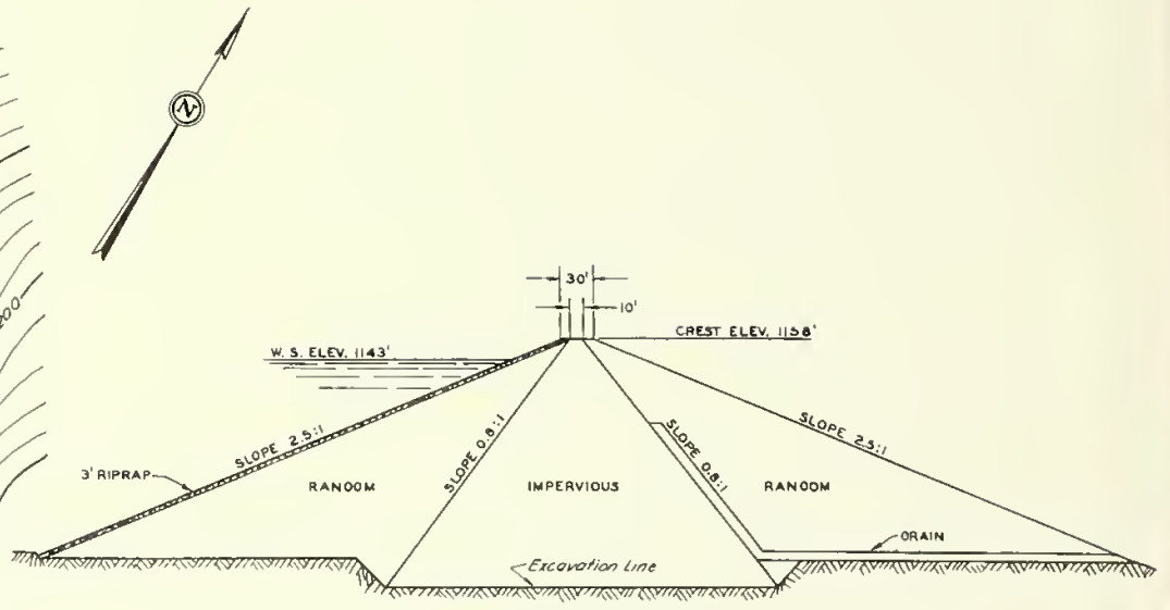
SECTION OF DAM SCALE OF FEET 0 100 200
