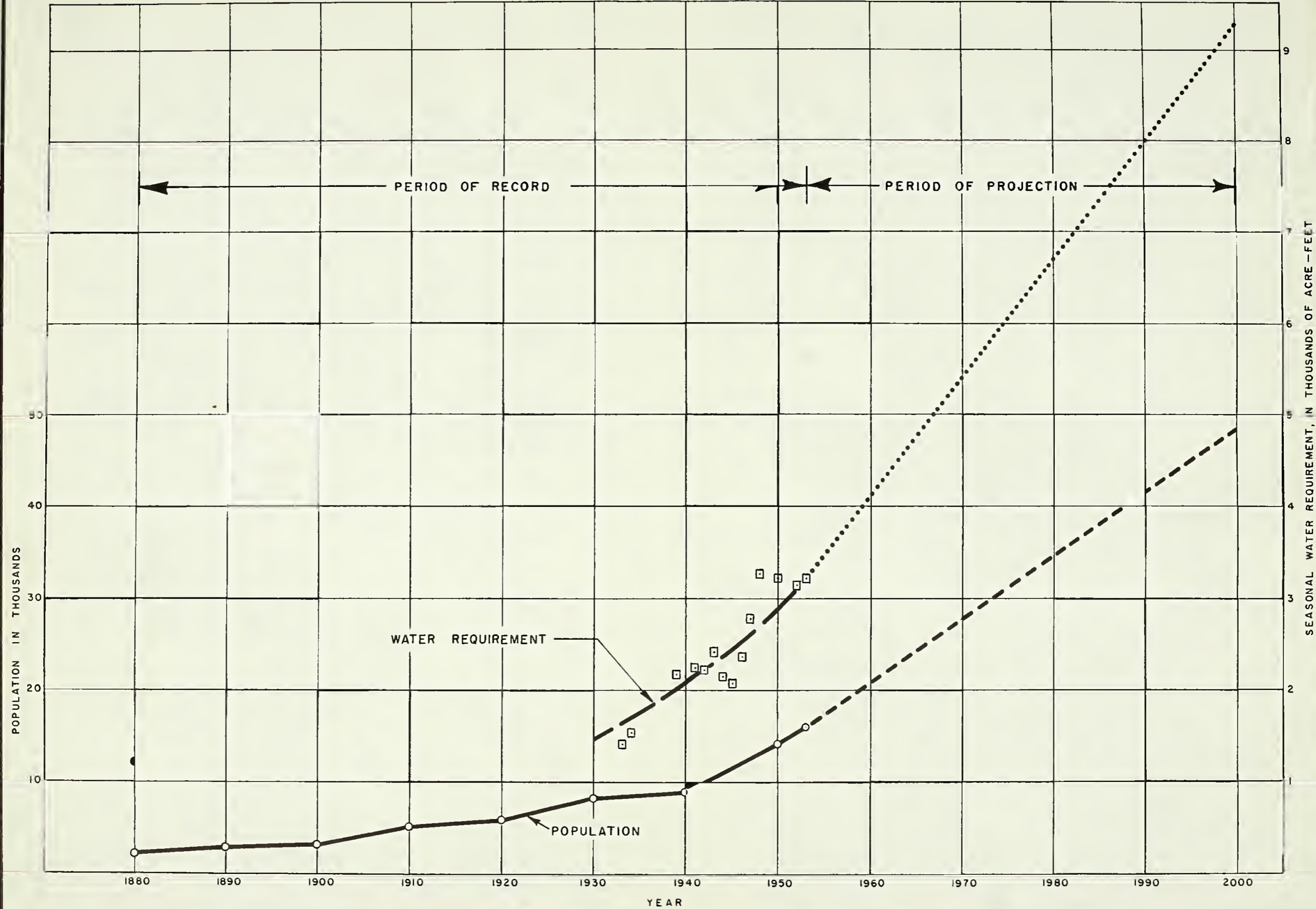
PROJECTION OF POPULATION AND WATER REQUIREMENT OF CITY OF SAN LUIS OBISPO
