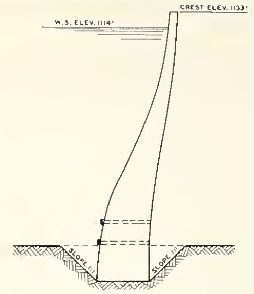
SECTION OF DAM SCALE OF FEET 0 50 100
