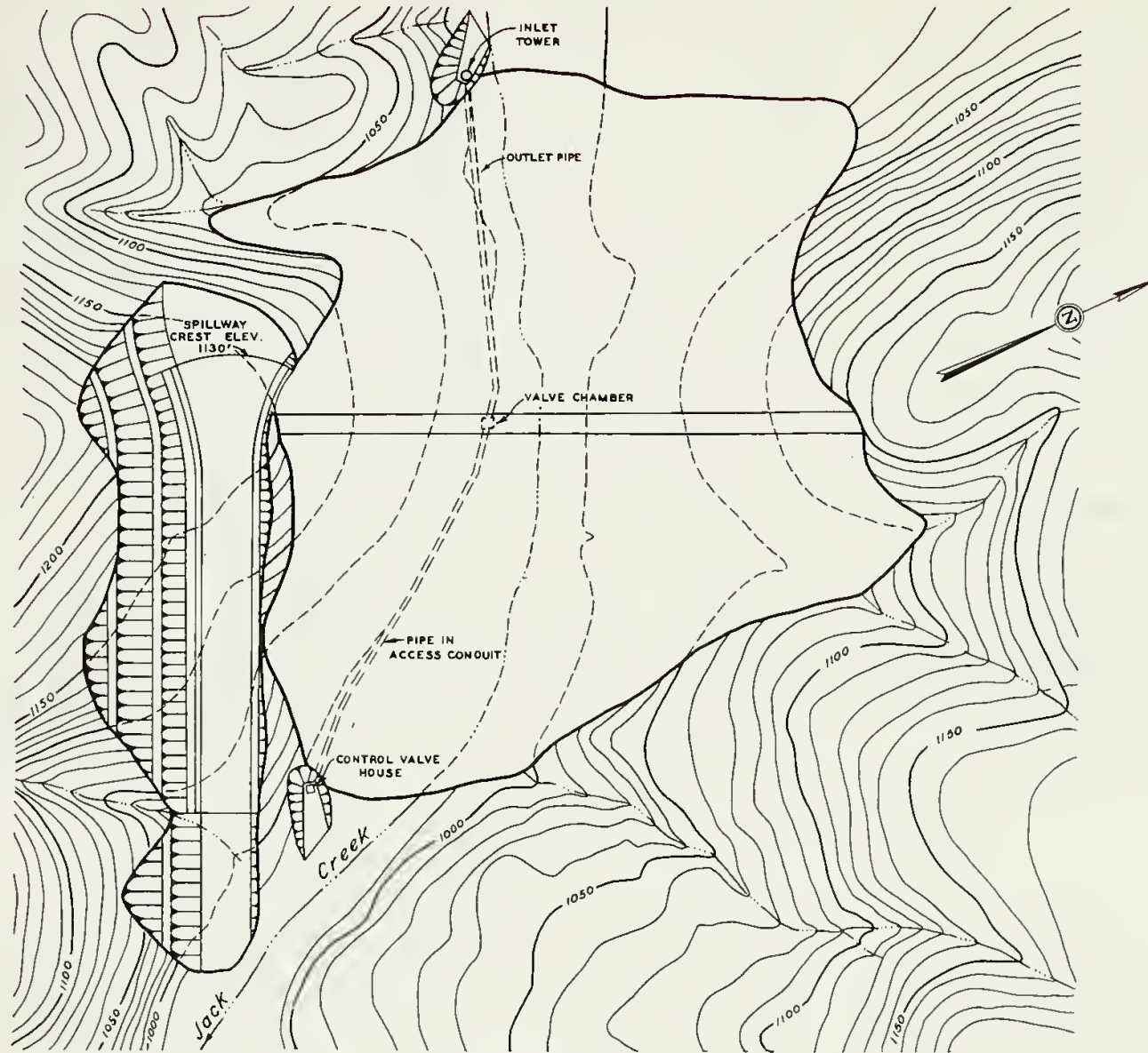
GENERAL PLAN SCALE OF FEET 0 100 200
