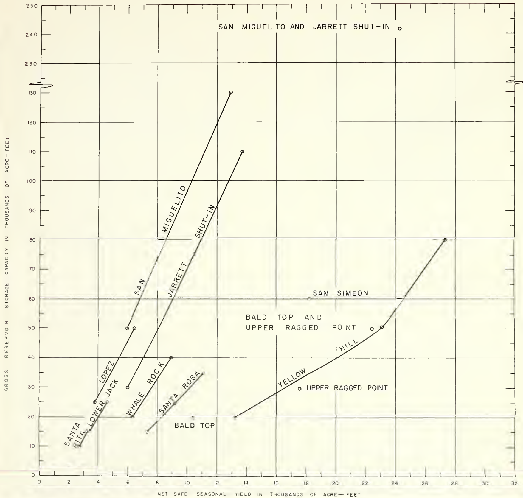
RELATIONSHIP BETWEEN STORAGE CAPACITY OF RESERVOIRS AND NET SAFE SEASONAL YIELD
