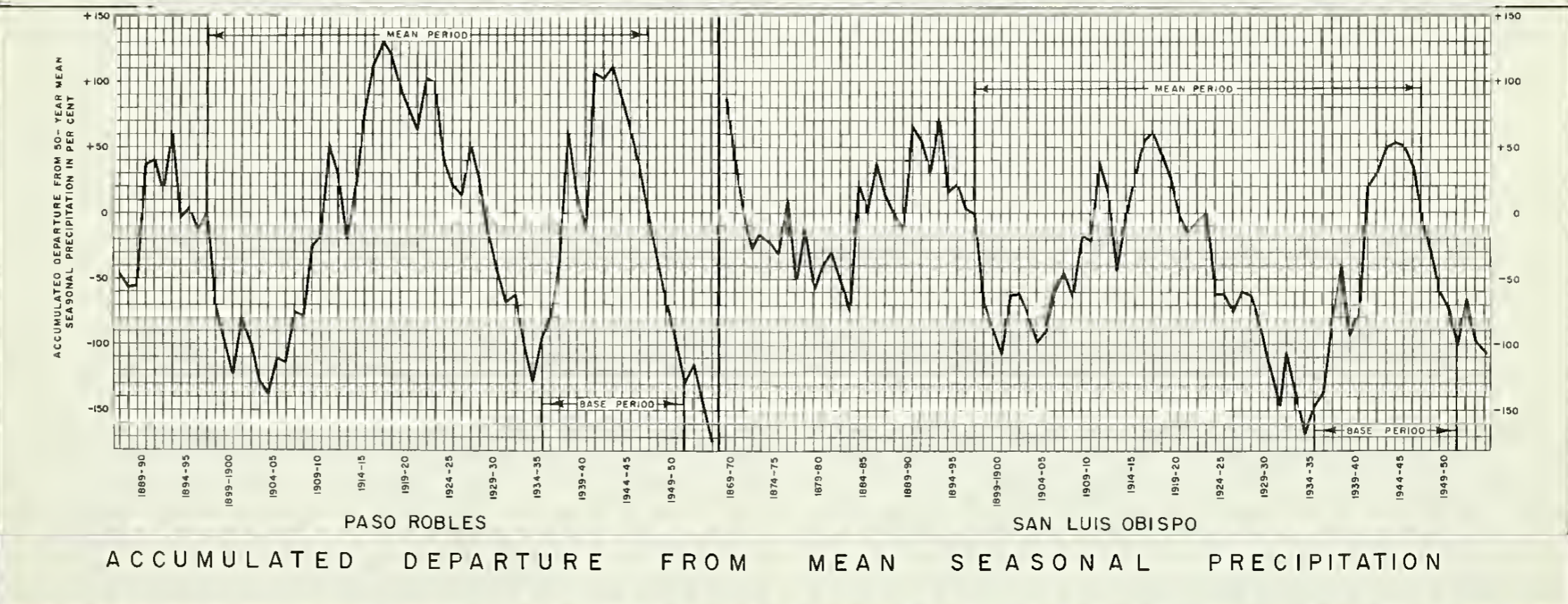
REPRESENTATIVE PRECIPITATION CHARACTERISTICS IN SAN LUIS OBISPO COUNTY
