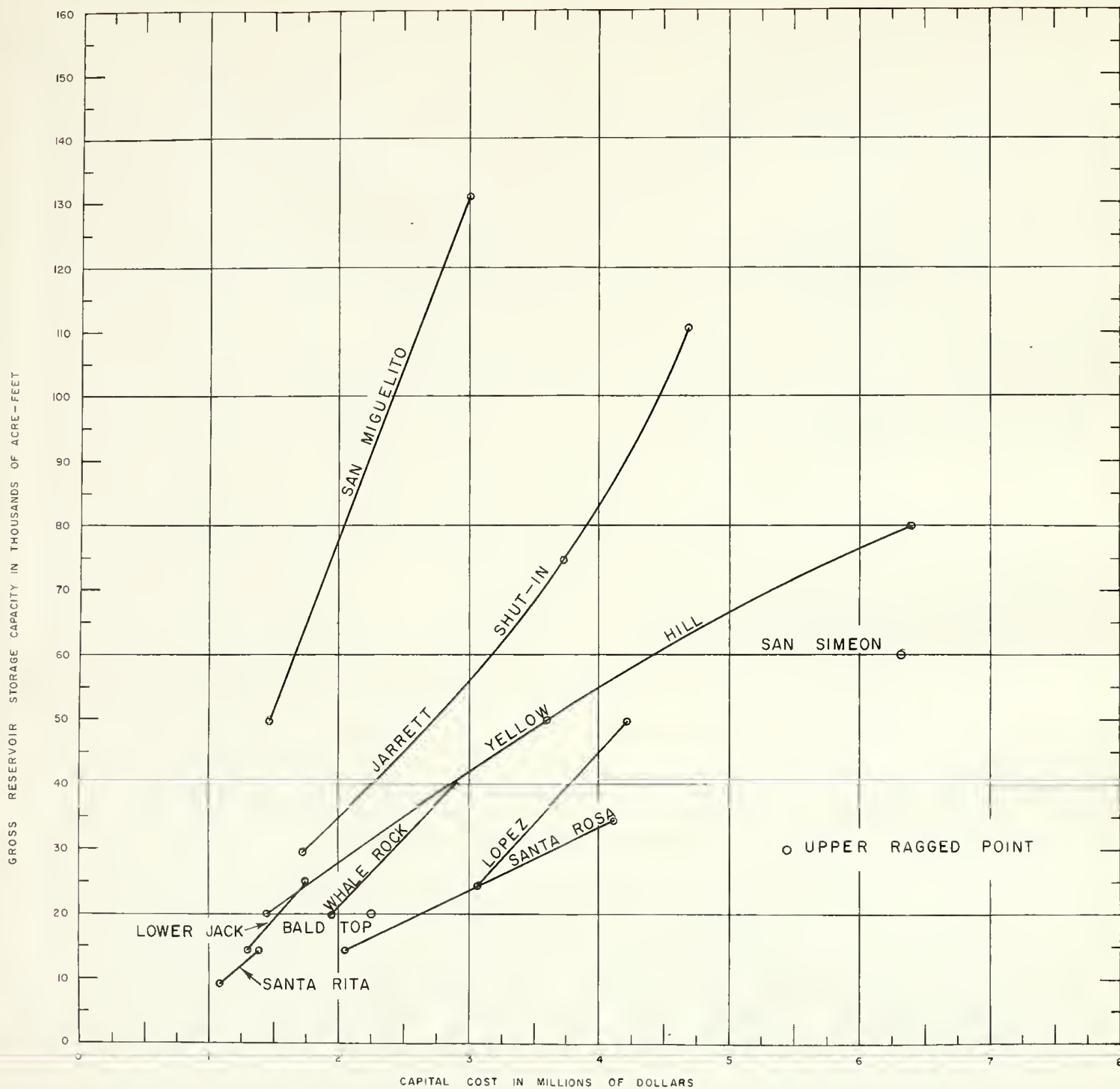
RELATIONSHIP BETWEEN STORAGE CAPACITY OF RESERVOIRS AND CAPITAL COST
