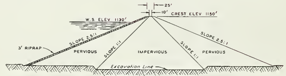
SECTION OF DAM SCALE OF FEET 0 100 200
