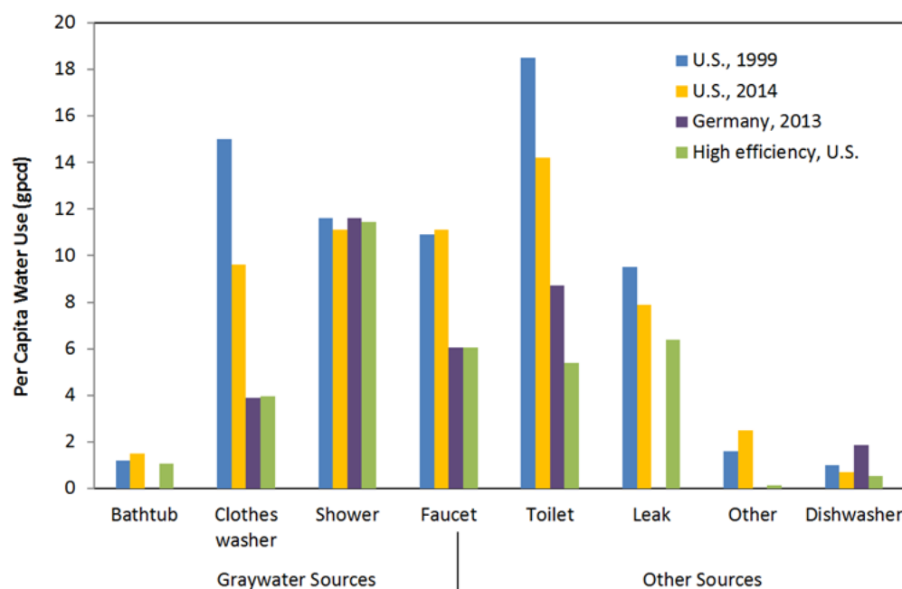
FIGURE 3-4 Average indoor water use in the United States in 1999 (69 gpcd) and 2014 (59 gpcd), Germany in 2013 (32 gpcd), and efficient new homes (36 gpcd). NOTES: Data collected in Germany do not include leaks, bathtubs, or other sources; thus, total water use figures are not comparable. Fixture data for high efficiency homes based on average household data and 3 persons per household. SOURCES: Data from Mayer et al. (1999); DeOreo et al. (2011; 2016); http://de.statista.com/statistik/daten/studie/224682/umfrage/trinkwasserverbrauch-in-deutschen-haushalten .
