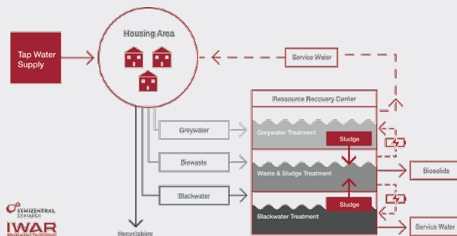
FIGURE 2-1-1 Flow schematic of the semicentralized Resource Recovery Center in Qingdao, China. SOURCE: J. Tolktsdorf, S. Bieker, P. Cornel, Technische Universität Darmstadt, Germany, http://www.semizentral.de .
