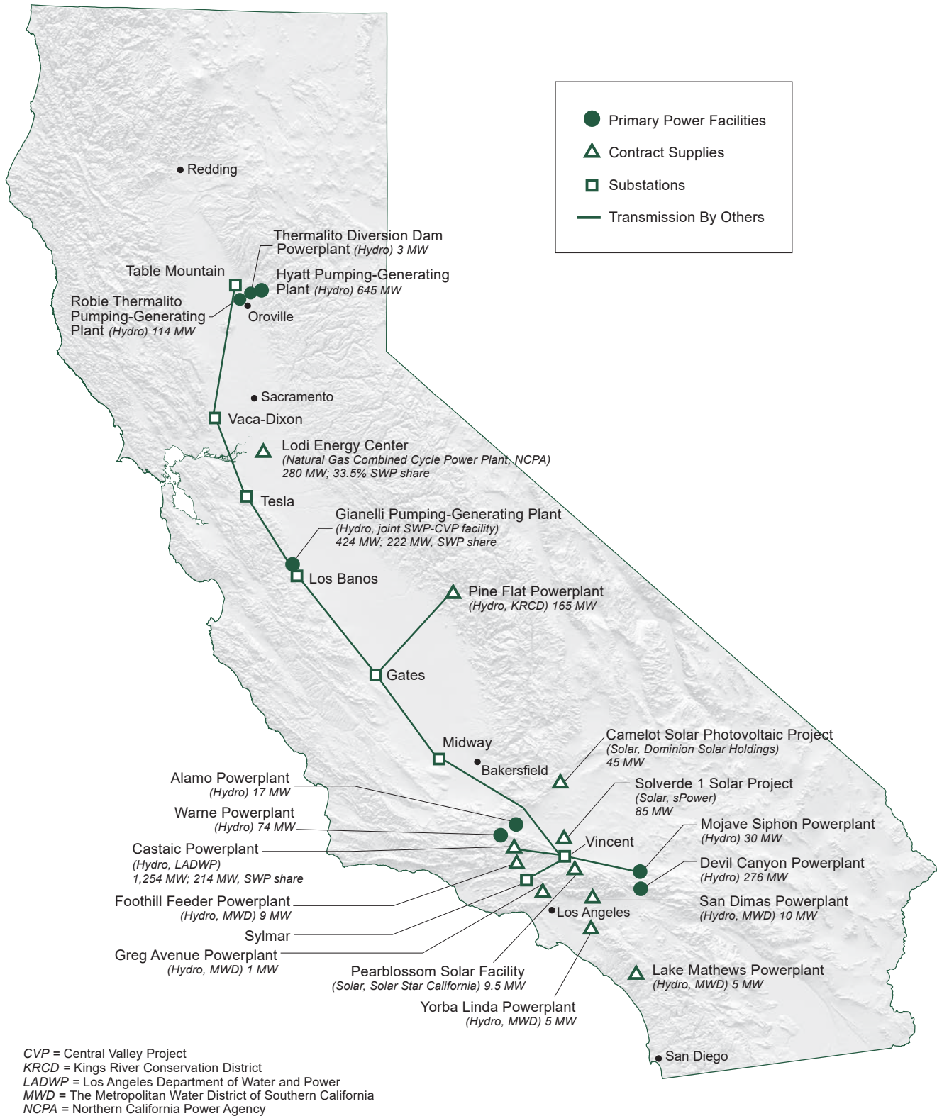
Figure 10-1 Names, Locations, and Nameplate Capacities of Primary Long-term Power Facilities
