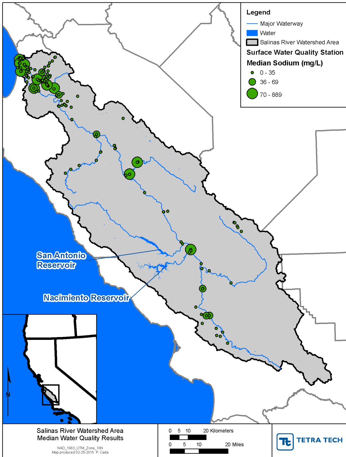
Figure 35. Median sodium results for the entire Salinas River Watershed area
