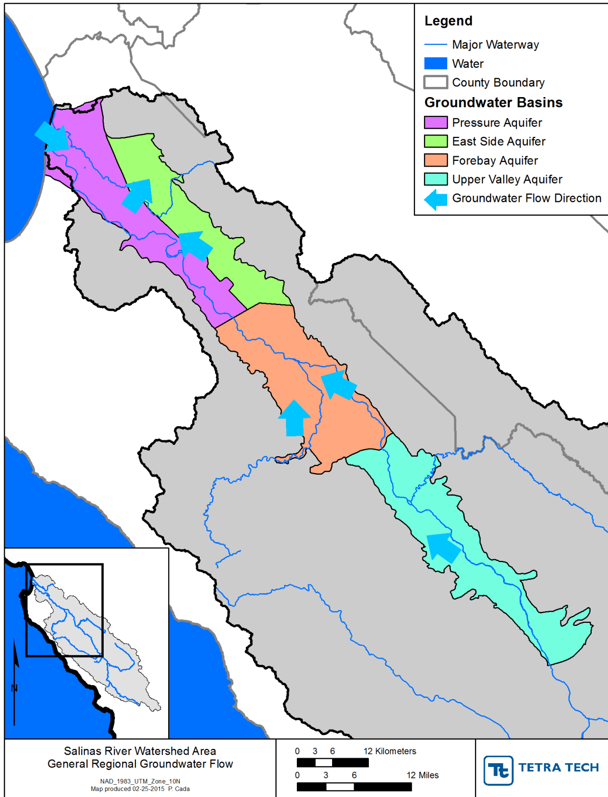
Figure 15. Regional groundwater flow direction in the Salinas Valley (based on information from Brown and Caldwell, 2015)
