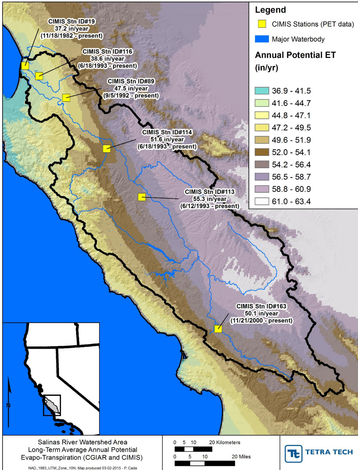
Figure 6. Long-term average annual evapotranspiration for the Salinas River Watershed area (data sources: CIMIS stations and CGIAR)
