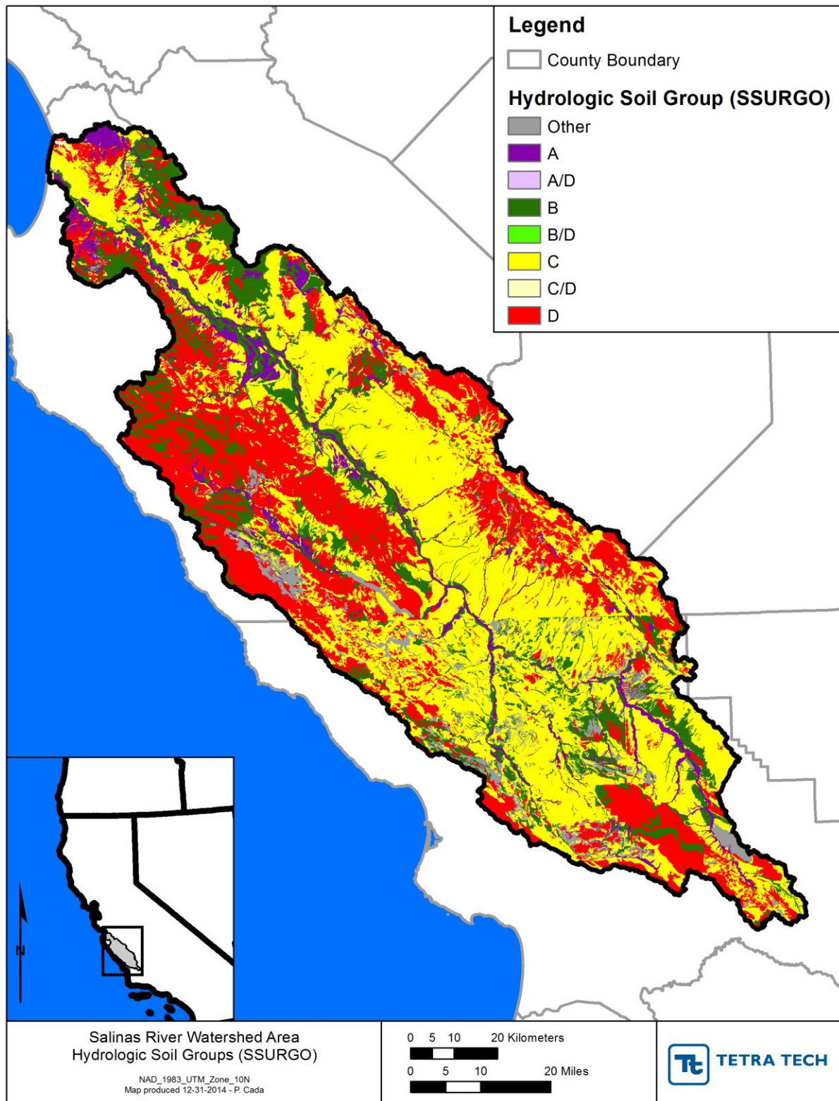
Figure 10. Hydrologic soil groups for the Salinas River Watershed area (SSURGO)
