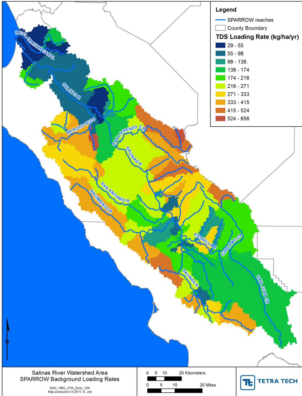
Figure 88. SPARROW Background TDS Loading Rates to Water Bodies
