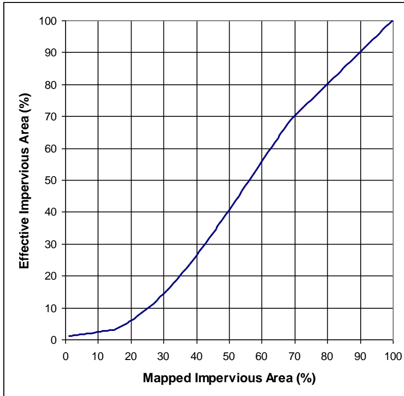
Figure 89. Effective impervious area to mapped impervious area relationship
