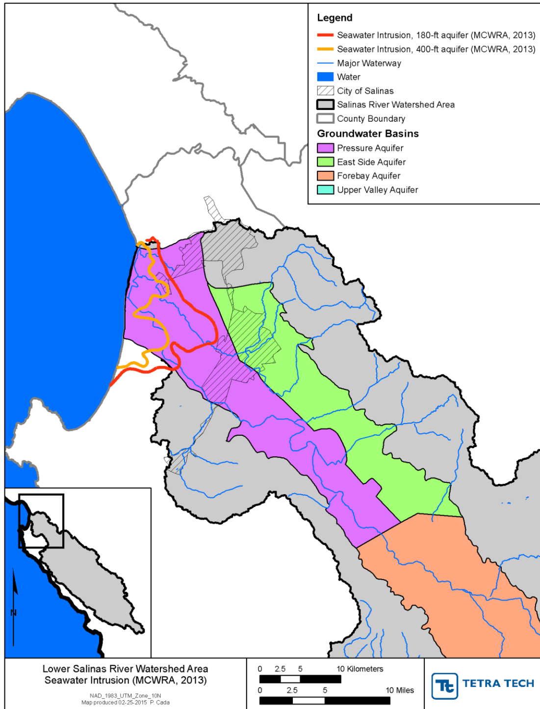
Figure 78. Salt water intrusion in the Salinas Valley Pressure Area (MCWRA, 2013)
