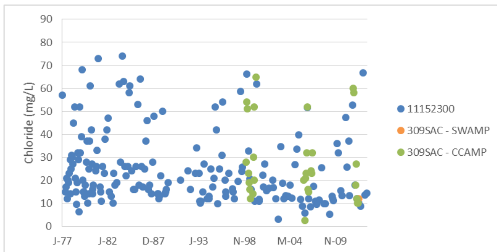
Figure 47. Time series of chloride at Salinas River at Chualar Bridge
