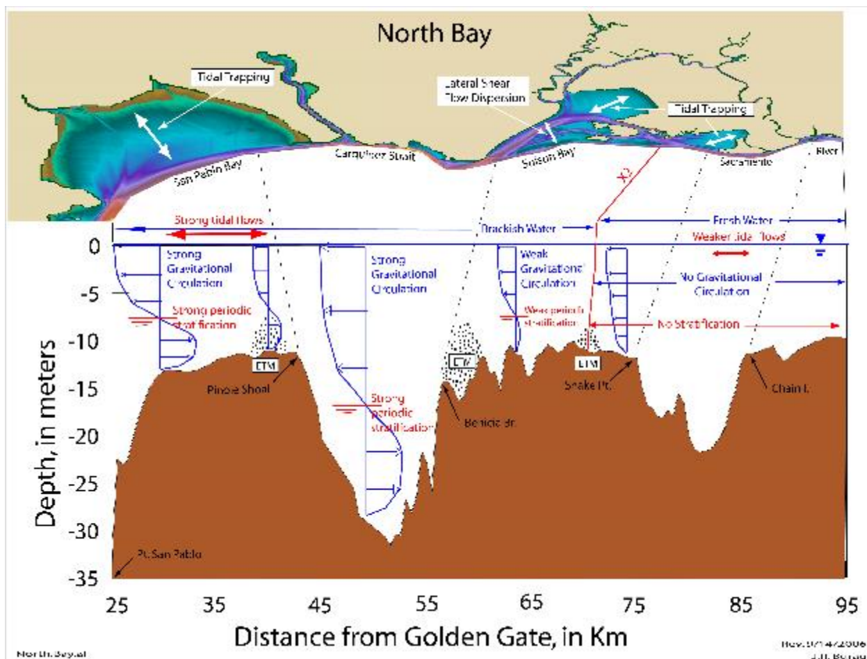
Figure 2-1 A Conceptual Model of Gravitational Circulation, Estuarine Turbidity Maximum (ETM) Formation, Salinity Stratification and Intrusion in the North Bay and Western Delta.
