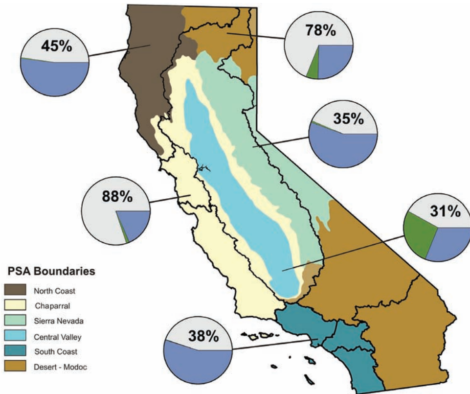
Figure D-1. Map of major Perennial Streams Assessment (PSA) regions with pie charts showing the relative proportion of perennial-wadeable (blue), perennial-non-wadeable (green) and non-perennial (gray) streams in each region. Thick black lines indicate Regional Water Board boundaries.
