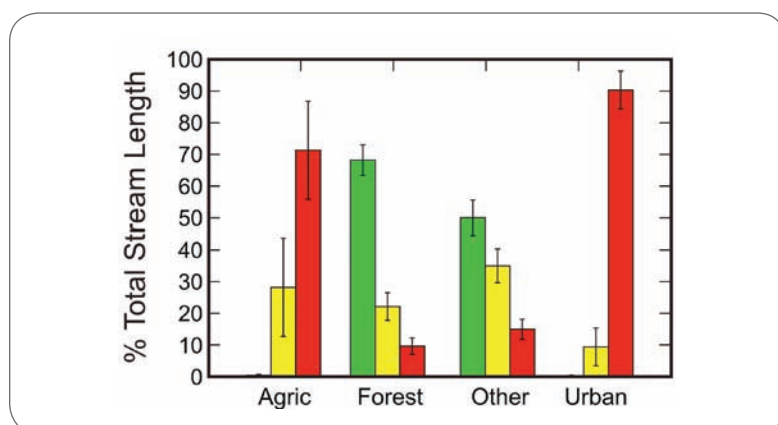
Figure 13. The biological condition of California's wadeable perennial stream length broken out by land cover (use) class. Green = good, yellow = degraded, red = very degraded, biological condition.
