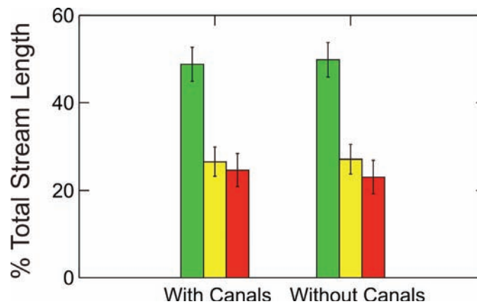
Figure B-1 Overall (eight-year) condition estimates produced with data from canal design included or excluded. Green = good biological condition, yellow = degraded biological condition, red = very degraded biological condition (see text for additional explanation).
