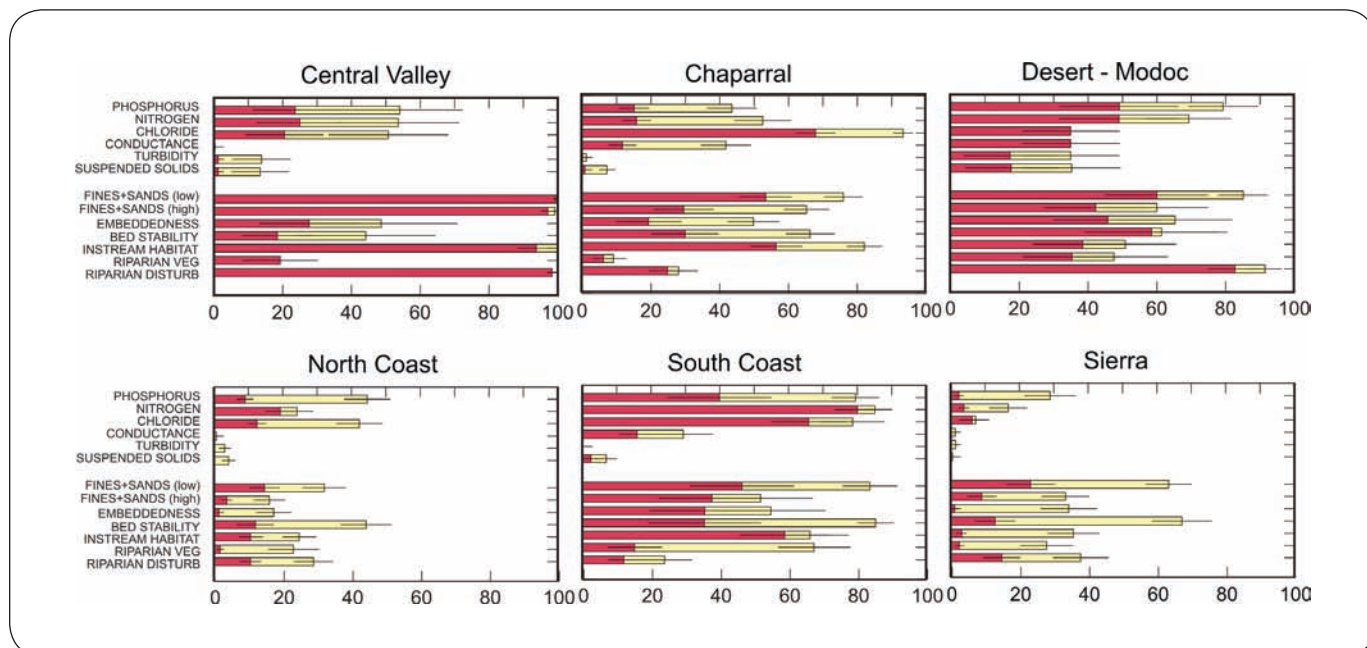
Figure 8a. Percentage of stream length within each Perennial Streams Assessment (PSA) region with chemical contamination or habitat alteration values greater than moderate (yellow) or severe (red) degradation thresholds. Stressor thresholds are listed in Appendix A-Table A-3.
