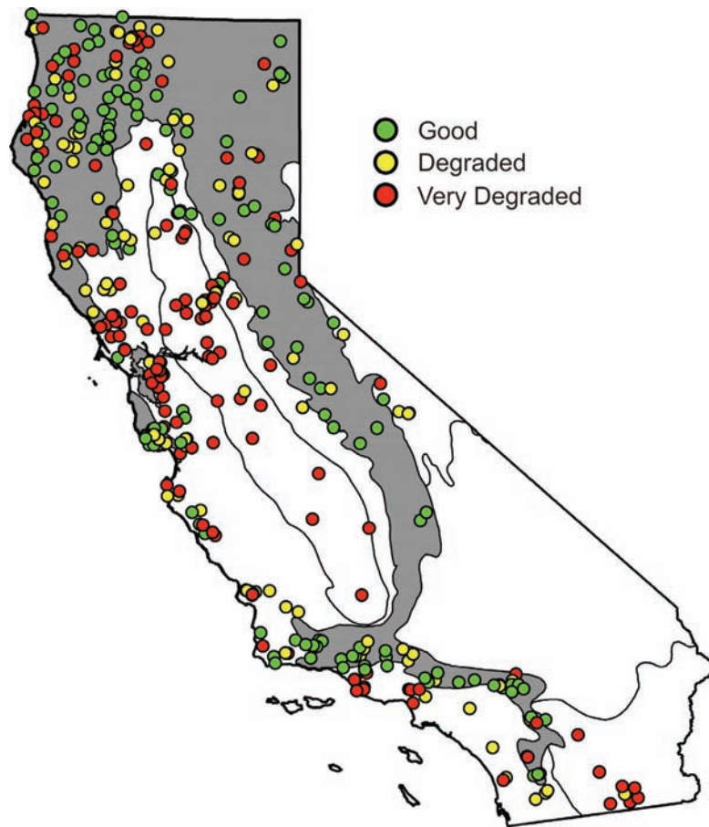
Figure 4. Distribution of survey sites coded by biological condition (green = good, yellow = degraded biology, red = very degraded biology).
