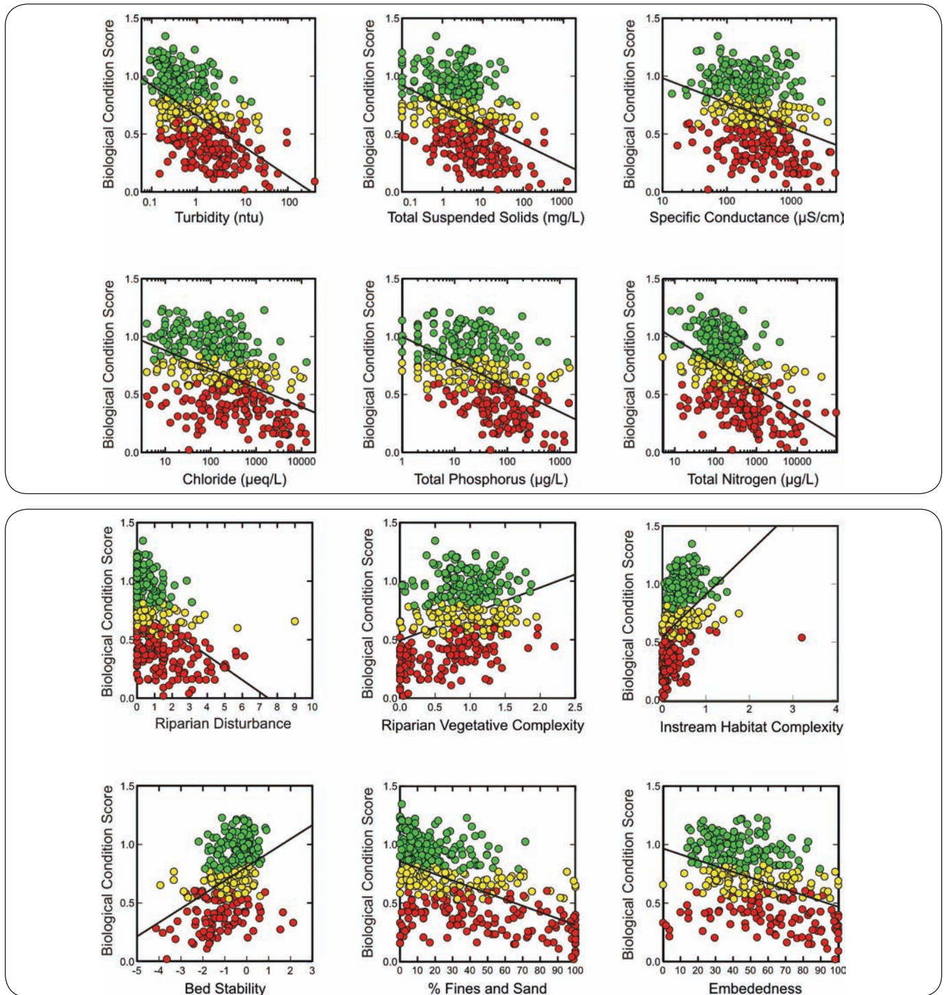
Figure E-8. Relationships between chemical and physical stressor intensity, habitat characteristics, and biological condition scores. Green dots represent sites in good biological condition and yellow and red dots represent sites with degraded and very degraded biological condition, respectively. Chemical stressors: chloride, total phosphorous, and total nitrogen. Physical stressors: turbidity, total suspended solids, specific conductance. Habitat characteristics: riparian disturbance, riparian vegetation, habitat complexity, bed stability, percent fines and sand, mean embeddedness. See Appendix Table A-3 for additional information.
