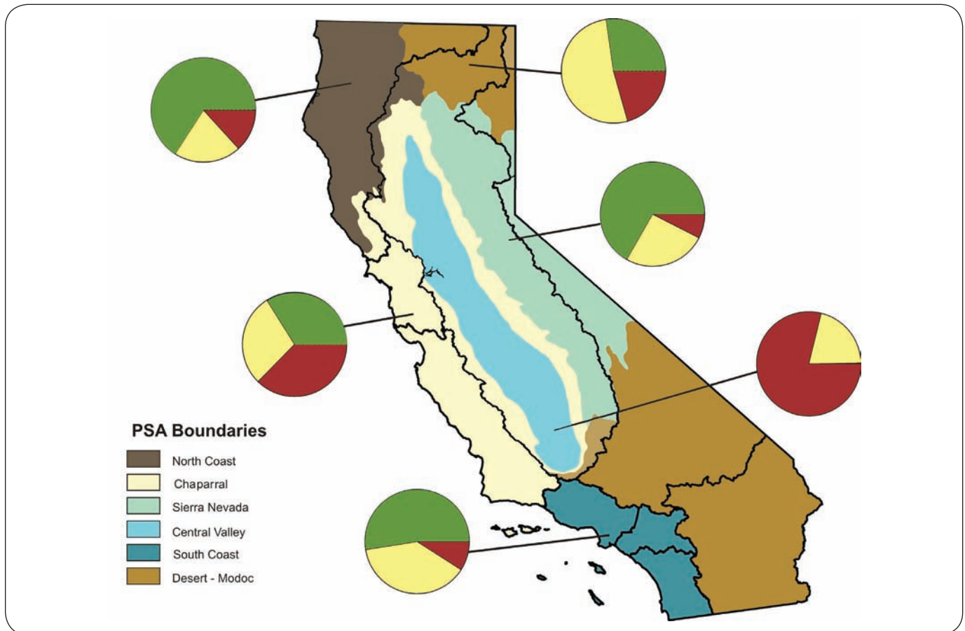
Figure 6b. The biological condition of wadeable perennial streams (pie charts: green = good, yellow = degraded, red = very degraded) in each of the six major Perennial Streams Assessment (PSA) regions in California.
