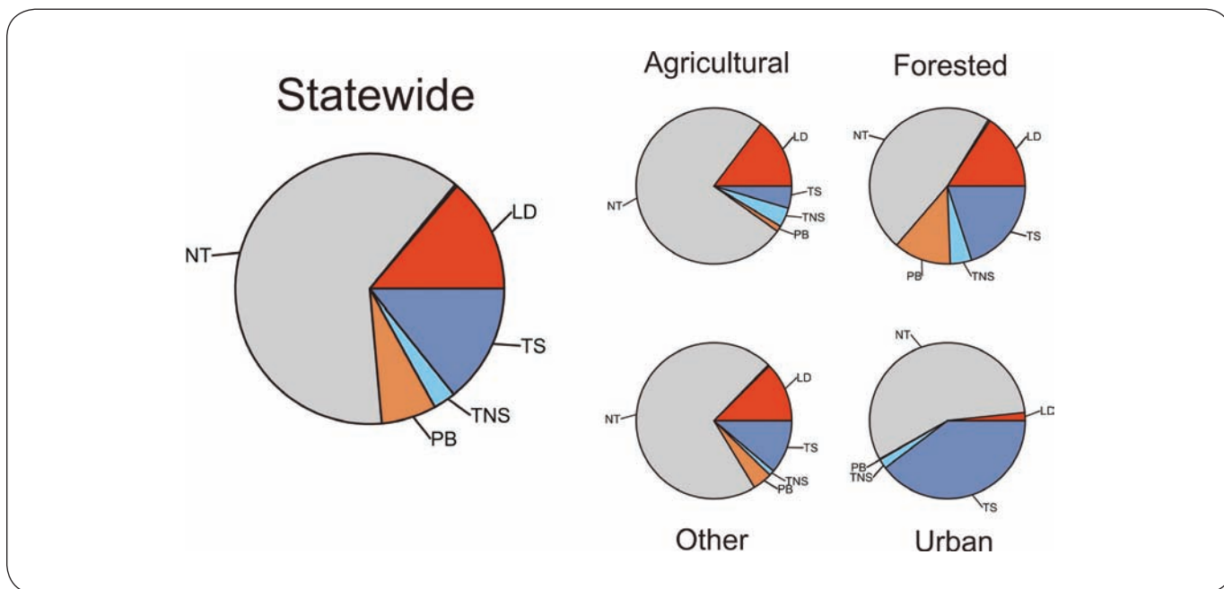
Figure D-2. Estimates (All Years: 2000-2007) of the percentage of total stream length falling into one of five reconnaissance fate classes: LD = landowner denial, NT = non-target, PB = physical barrier, TNS = target, not sampled, TS = target sampled. Results are shown for all sites for each of the four land cover/ land use classes. (Percentages and total stream length estimates are listed in Appendix E, Table E-1.)
