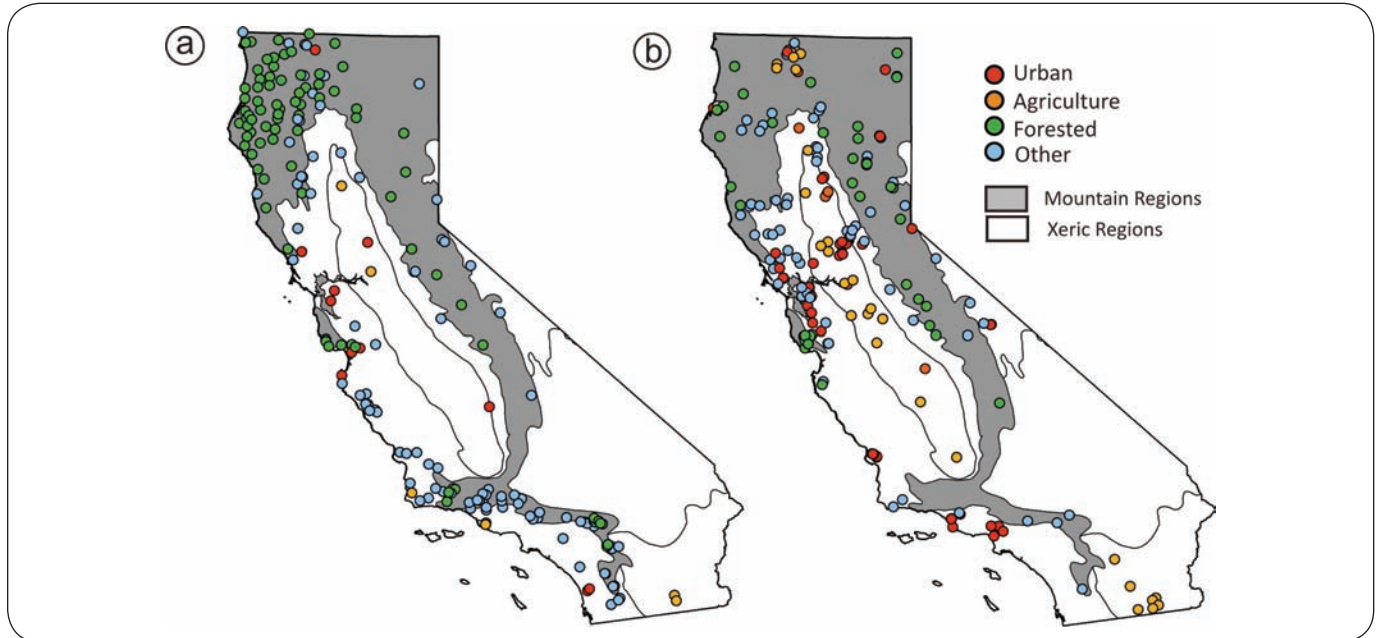
Figure E-1. Distribution of sites used in condition assessments coded by final land use designation: a) Environmental Monitoring Assessment Program (EMAP) sites and b) California Monitoring Assessment Program (CMAP) sites.
