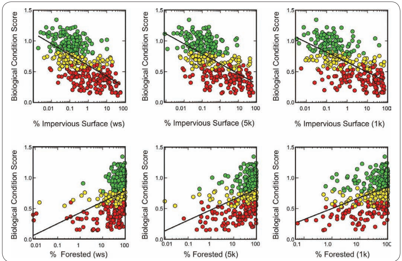
Figure E-9a. Relationship between development impact intensity at three spatial scales (watershed, 5 kilometers, and 1 kilometer) and biological condition scores. Green dots represent sites in good biological condition and yellow and red dots represent sites with degraded and very degraded biological condition, respectively. Condition analysis is presented for agricultural, urban, agricultural + urban, forest, and impervious surface development categories. See Appendix Table A-3 for additional information.
