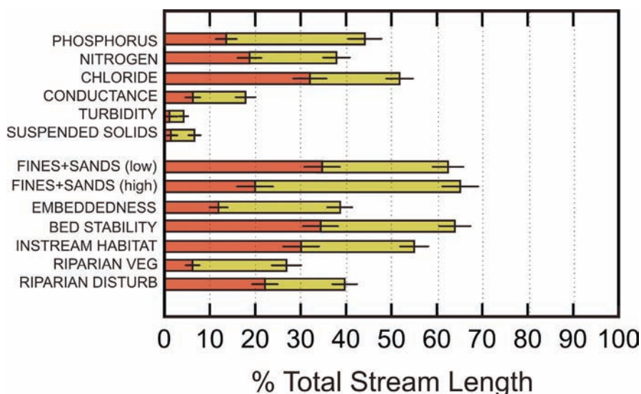
Figure 7a. Percentage of statewide stream length with chemical and habitat assessment values above moderate (yellow) and severe (red) degradation thresholds. Stressors and thresholds are listed in Appendix A, Table A-3. Bars for severe thresholds are plotted on top of bars for moderate thresholds.
