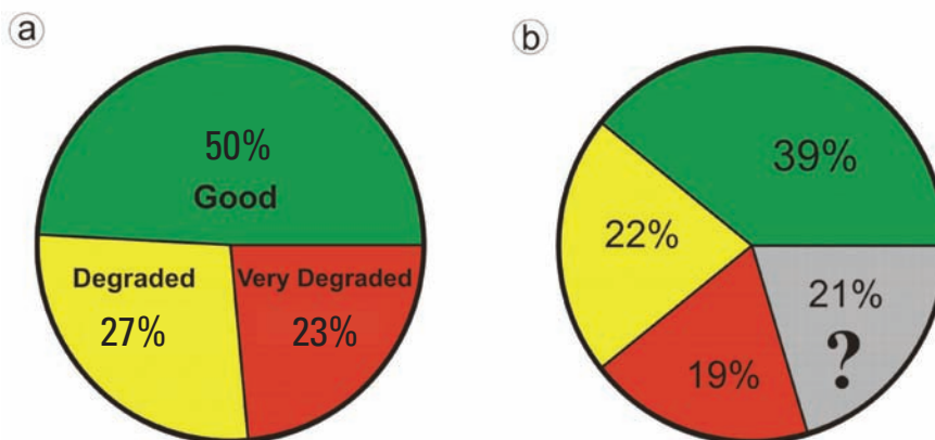
Figure 5. The percent of total stream length in different biological condition classes. Two presentation alternatives: a) with the proportion of unassessed stream length (reconnaissance fate codes LD, PB and NS) extrapolated from the sampled target site data (TS + TNS), b) with unassessed stream length left as a distinct category (adjusted for non-perennial stream length and represented here by a question mark).
