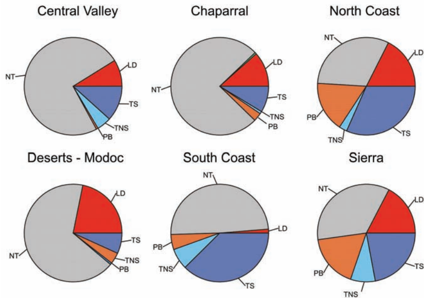
Figure D-3. Estimates of the percentage of total stream length falling into one of five reconnaissance fate classes: LD = landowner denial, NT = non-target, PB = physical barrier, TNS = target, not sampled, TS = target sampled. Results are shown for the six Perennial Streams Assessment (PSA) regions of California. (Percentages and total stream length estimates are listed in Appendix E, Table E-2.)
