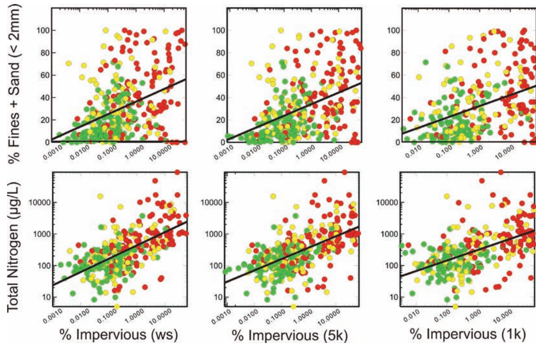
Figure 22. Bi-plots of relationships between two stressors (nitrogen concentration and proportion of fine sediments) and impervious surface at three spatial scales. Codes in parentheses refer to the spatial scale for analysis: ws = entire upstream watershed, 5k = 5 kilometer area upstream of site, 1k = 1 kilometer area upstream of site. Colored dots represent sites in good biological condition (green), degraded condition (yellow) or very degraded condition (red).
