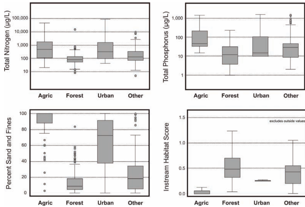
Figure 15. Distribution of chemical and physical habitat variables in each of the four Non-Point Source (NPS) land cover classes for total nitrogen, total phosphorous, percent sand and fines, and instream habitat score. Note the use of a log scale on some of the plots and that outside values (dots) were removed from the instream habitat plot for clarity.
