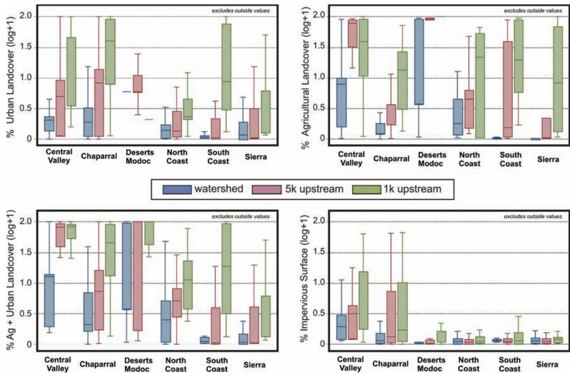
Figure E-5. Stressor distribution boxplots in three distinct spatial scales (ws = watershed, 5k = 5 kilometers, 1k = 1 kilometer), for the land cover variables urban, agricultural, urban + agricultural, and impervious surface, by Perennial Streams Assessment (PSA) region.
