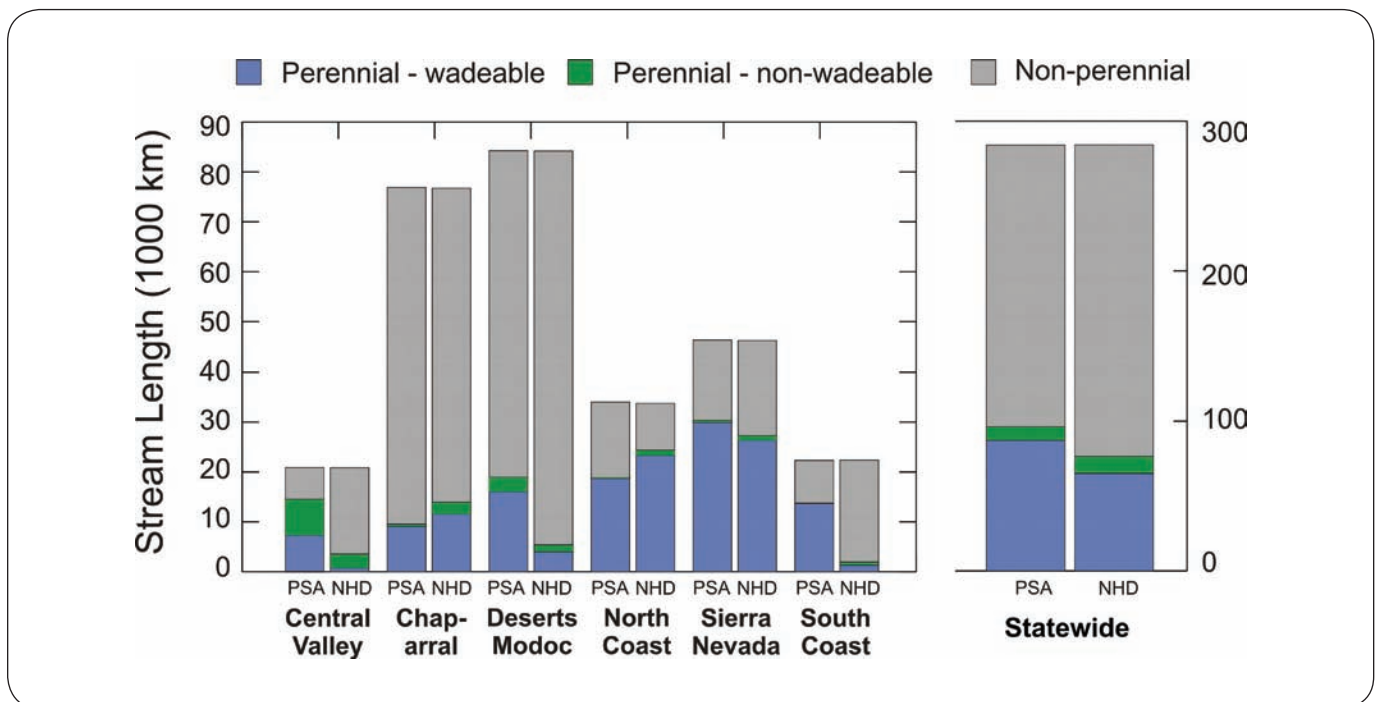
Figure 3. The length and relative proportion of perennial wadeable, perennial non-wadeable and non-perennial streams, in each of the six major Perennial Streams Assessment (PSA) regions. The first bar in each pair represents estimates generated from PSA (this study) and the other bar represents data derived from National Hydrology Database (NHD+). The heights of PSA bars were rescaled to match NHD totals for easier comparisons of flow classes.
