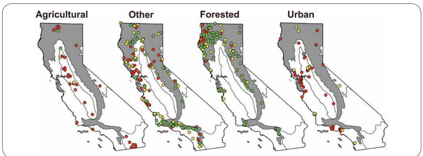
Figure E-2. Distribution of site scores in each of four Non-Point Source (NPS) categories. Green = good, yellow = degraded, red = very degraded.
