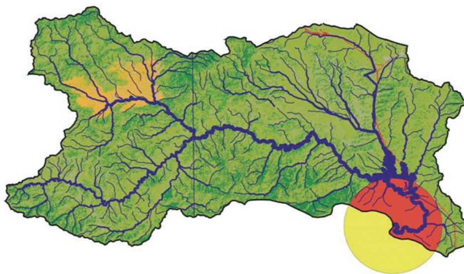
Figure A-1. Example watershed showing a 1 km surrounding a survey point. The percent of land used for agriculture, urban and other uses was calculated upstream of each survey point (area in red) for three spatial scales: 1 km, 5 km and watershed scale.
