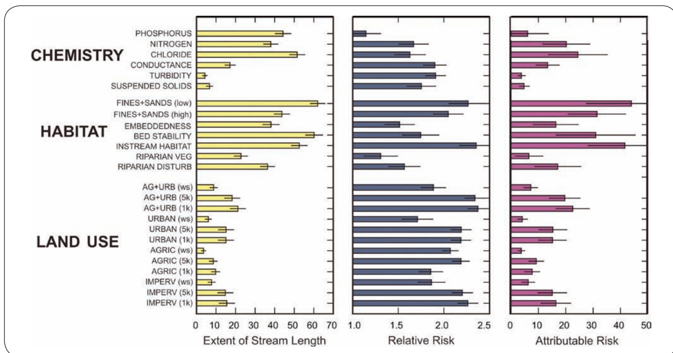
Figure 16. Stressor extent, relative risk and attributable risk estimates for chemical, habitat and land use variables. All three variables are based on the moderate threshold levels presented in Appendix A, Table A-3. Variable codes: AG + URB = combination of agricultural and urban land use, URBAN = % urban land use, AGRIC = % agricultural land use, IMPERV = % impervious surface. Codes in parentheses refer to the spatial scale at which the land cover was calculated: ws = entire upstream watershed, 5k = 5 kilometer area upstream of site, 1k = 1 kilometer area upstream of site.
