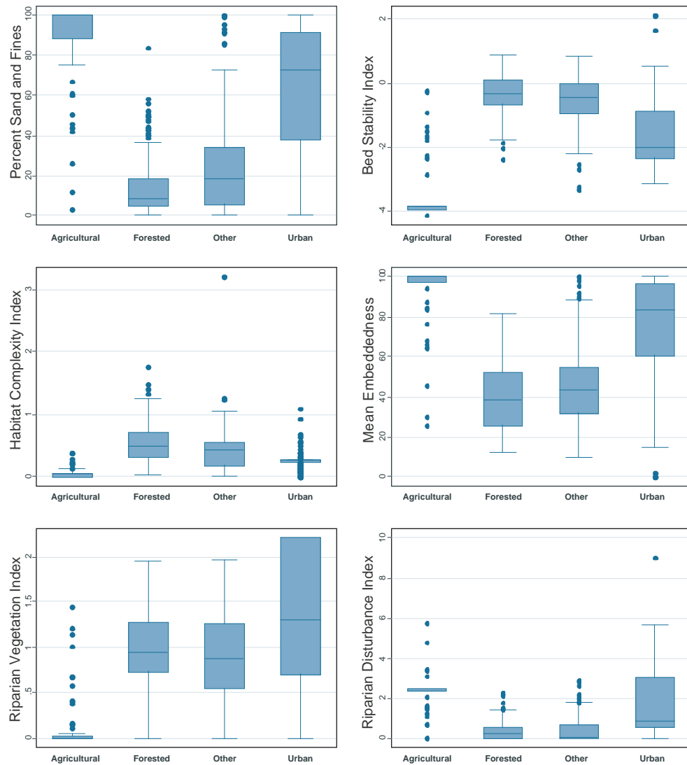
Figure E-7. Stressor distribution boxplots by Non-Point Source (NPS) land cover class for habitat variables: percent fines and sands, bed stability, habitat complexity index (EMAP composite), mean embeddedness, riparian vegetation index (EMPA composite), riparian disturbance index (EMAP composite).
