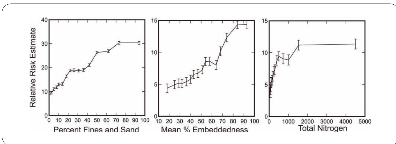
Figure 17. Continuous risk threshold plots showing the relationship between relative risk and stressor intensity for three example stressors.
