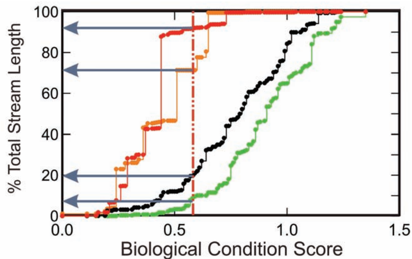
Figure C-2. Overall cumulative distribution of biological condition scores for each of four land cover classes, derived from eight years of stream surveys. Each point on the lines, represents a biological condition score for a stream running through a particular land use area: Red = urban sites, Orange = agricultural sites, Green = forested sites, and Black = other sites. The red line indicates a biological condition score threshold demarcating the point below which sites are in very degraded condition. The corresponding percent of stream length falling below this threshold is indicated on the y-axis (see gray arrows).
