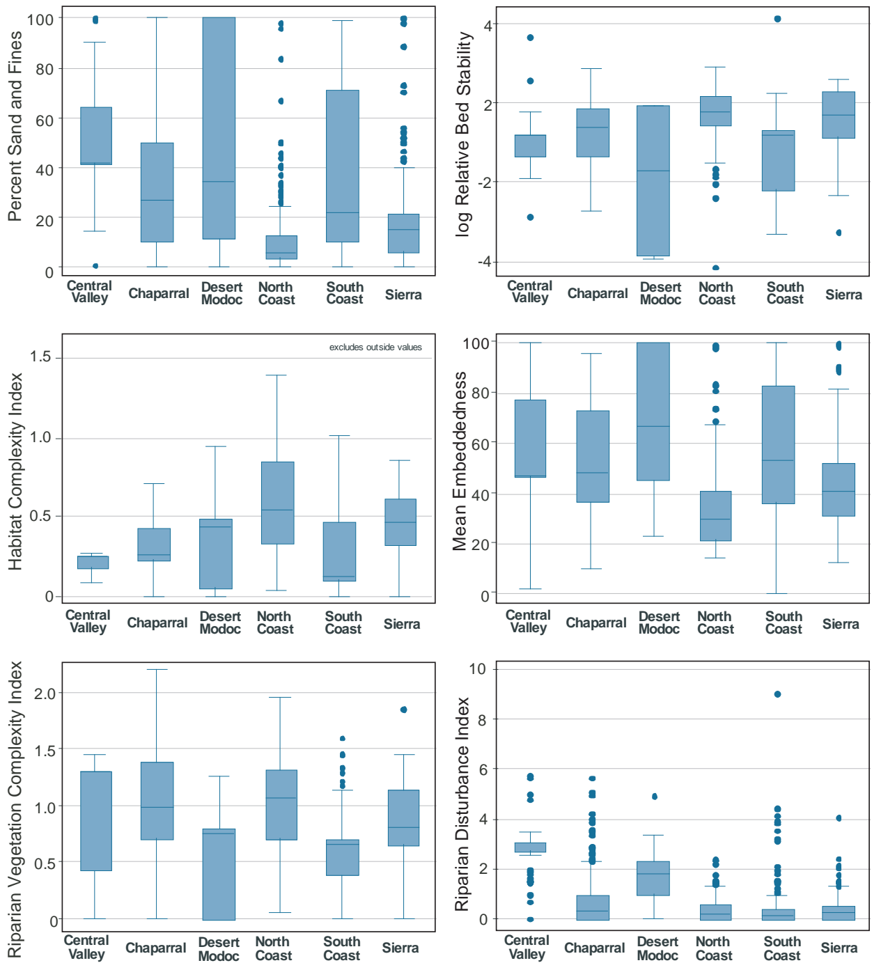
Figure E-4. Stressor distribution boxplots by Perennial Streams Assessment (PSA) region for habitat variables: percent fines plus sand, streambed stability, habitat complexity (EMAP composite), mean embeddedness, riparian vegetation complexity (EMAP composite) and riparian disturbance index (EMAP composite). Definition codes are also listed in Appendix A, Table A-3.
