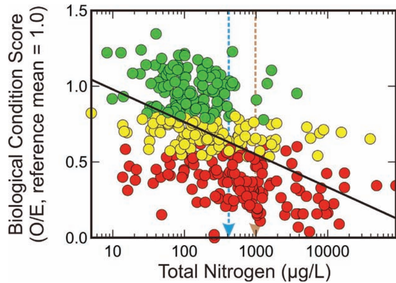
Figure 18. Statewide relationship between total nitrogen concentration and biological condition scores. Green dots represent sites in good condition and yellow and red dots represent sites with degraded and very degraded biological condition, respectively. The blue dotted line represents a 90th percentile threshold (see text) and the brown line indicates a common nitrogen impairment threshold.
