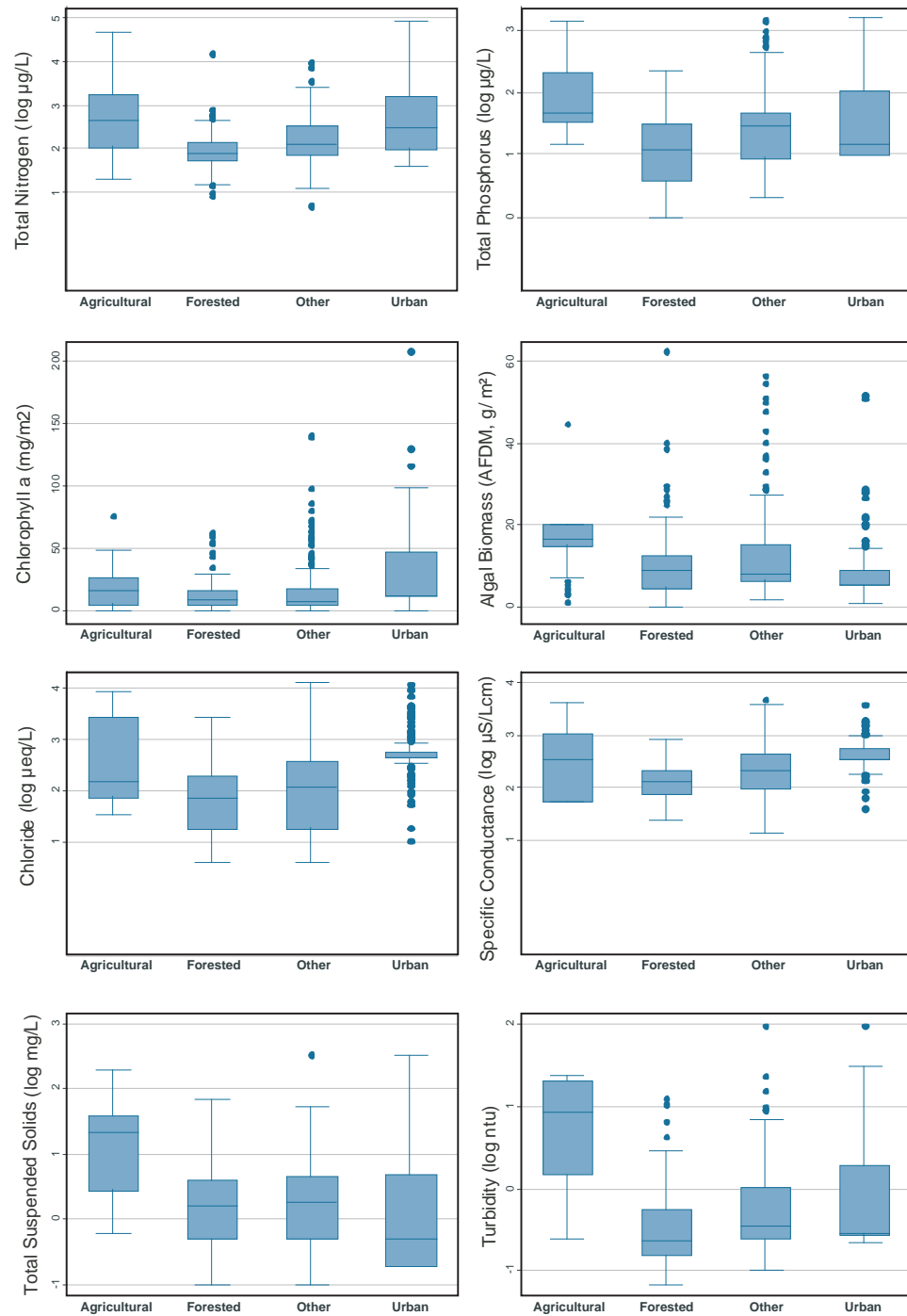
Figure E-6. Stressor distribution boxplots by Non-Point Source (NPS) land cover class for chemical variables: total nitrogen, total phosphorus, chlorophyll a, algal biomass (ash free dry ), chloride, specific conductance, total suspended solids, and turbidity. See Table A-3 for additional information.
