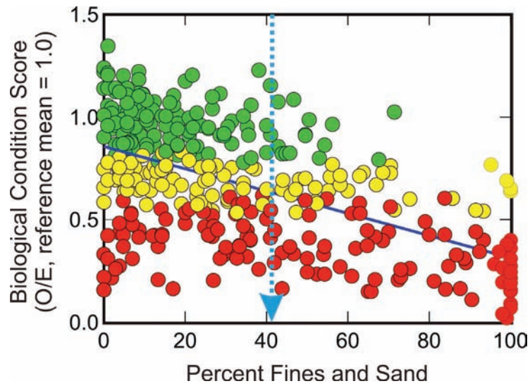
Figure 20. Statewide relationship between the percentage of fine sediments in sampling reaches and biological condition scores. Green dots represent sites in good biological condition and yellow and red dots represent sites with degraded and very degraded biological condition, respectively. The blue dotted line represents a 90th percentile threshold (see text).
