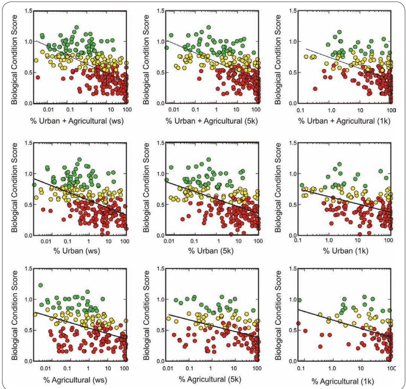
Figure E-9b. Relationship between development impact intensity at three spatial scales (watershed, 5 kilometers, and 1 kilometer) and biological condition scores. Green dots represent sites in good biological condition and yellow and red dots represent sites with degraded and very degraded biological condition, respectively. Condition analysis is presented for agricultural, urban, agricultural + urban, forest, and impervious surface development categories. See Appendix Table A-3 for additional information.
