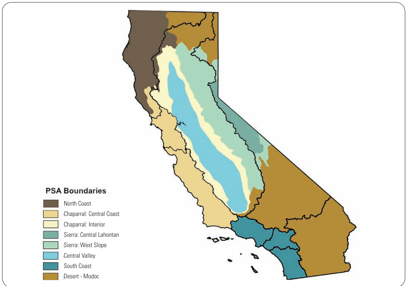
Figure 2. Boundaries of the eight major Perennial Streams Assessment (PSA) subdivisions used in surveys. Black lines correspond to regional water board boundaries. The sub-regions of the Chaparral and Sierra regions were combined for summary analyses in this report.
