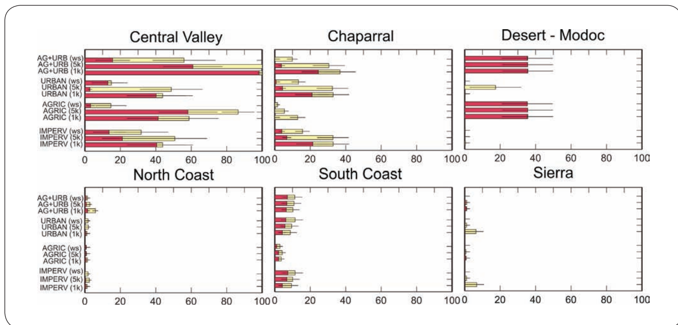
Figure 8b. Percent of stream length in each Perennial Streams Assessment (PSA) region with land use coverage that exceed moderate (yellow) or severe (red) degradation thresholds. Variable codes: AG + URB = combination of agricultural and urban land use, URBAN = % urban land use, AGRIC = % agricultural land use, IMPERV = % impervious surface. Codes in parentheses refer to the spatial scale at which the land cover was calculated: ws = entire upstream watershed, 5k = 5 kilometer area upstream of site, 1k = 1 kilometer area upstream of site. Stressors code definitions and thresholds are also listed in Appendix A-Table A-3.
