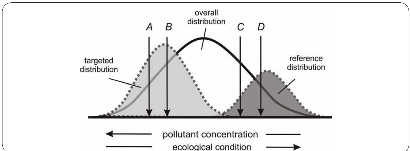
Figure 10. Theoretical distributions of monitoring variables across all sites (e.g., from PSA probability surveys) and across reference sites (e.g., from SWAMP's RCMP). Letters (A-D) refer to hypothetical site values discussed in the text.
