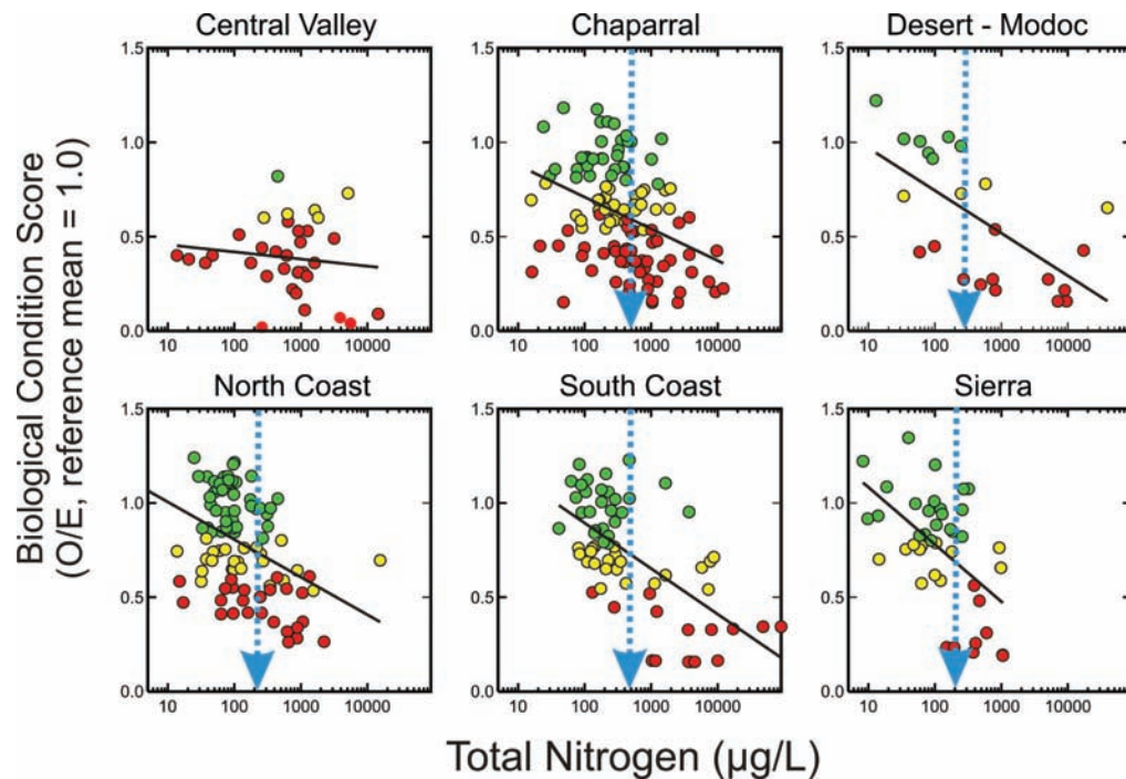
Figure 19. Relationship between biological condition scores and total nitrogen concentration in each Perennial Streams Assessment (PSA) Region. Green dots represent sites in good biological condition and yellow and red dots represent sites with degraded and very degraded biological condition, respectively.
