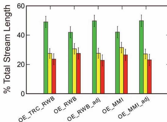
Figure B-2. Overall (eight-year) condition assessments based on five different versions of the biological scoring index. Green = good, yellow = degraded, red = very degraded, biological condition. O/E = observed/expected; TRC = Targeted Riffle Composite; RWB = Reachwide Benthos; MMI = Multi-metric Index; such as Biological Condition Score.
