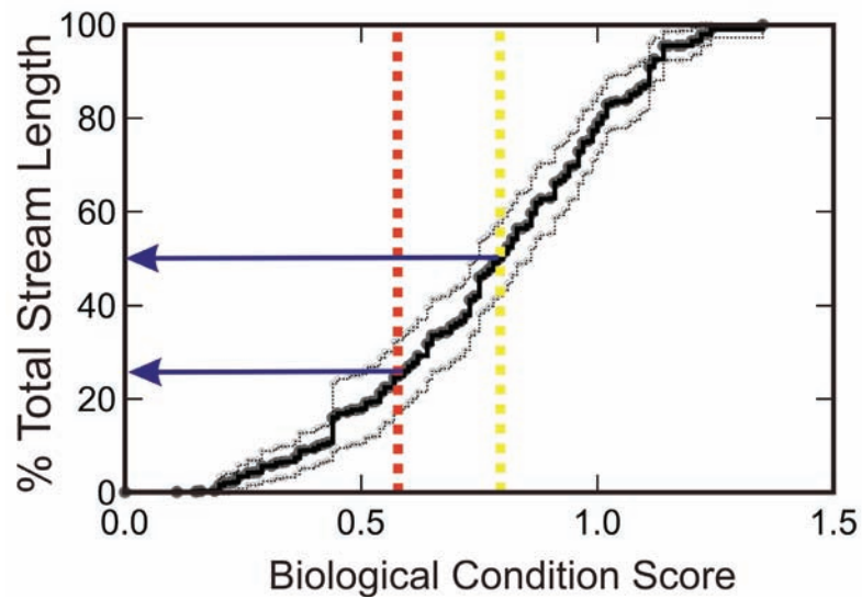
Figure C-1. Cumulative distribution graph of biological condition scores with upper and lower 95% confidence limits, and biological condition thresholds, representing eight-years of stream surveys. The heavy black line composed of points indicates the biological condition score from each site. The dotted gray lines represent the upper and lower 95% confidence limits of the scores. The yellow line indicates a threshold point, below which biological condition scores are degraded. The red line indicates the threshold point below which biological condition scores are very degraded. Each threshold corresponds to a specific percent of stream length (indicated by the blue arrows).
