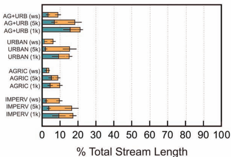
Figure 7b. Percent of total stream length statewide that exceed moderate (orange) and high (blue) land use coverage thresholds. Land use thresholds and variable codes are described in Appendix A, Table A-3. Codes in parentheses refer to the spatial scale at which the land cover was calculated: ws = entire upstream watershed, 5k = 5 kilometer area upstream of site, 1k = 1 kilometer area upstream of site. Variable codes: AG + URB = combination of agricultural and urban land use, URBAN = % urban land use, AGRIC = % agricultural land use, IMPERV = % impervious surface.
