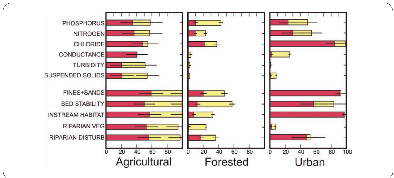
Figure 14. Percentage of California's stream length in each of three major land cover classes that exceeded degradation thresholds for chemical and physical habitat stressors. Red bars represent severe degradation thresholds and yellow bars represent moderate degradation thresholds. Threshold values are presented in Appendix A, Table A-3.
