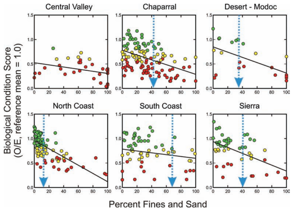
Figure 21. Scatterplots of biological condition scores in each of the six Perennial Streams Assessment (PSA) regions, as a function of the percent of fine sediments in the sampling reach. Green dots represent sites in good biological condition and yellow and red dots represent sites with degraded and very degraded biological condition, respectively. The blue dotted lines represents the 90th percentile threshold (see text).
