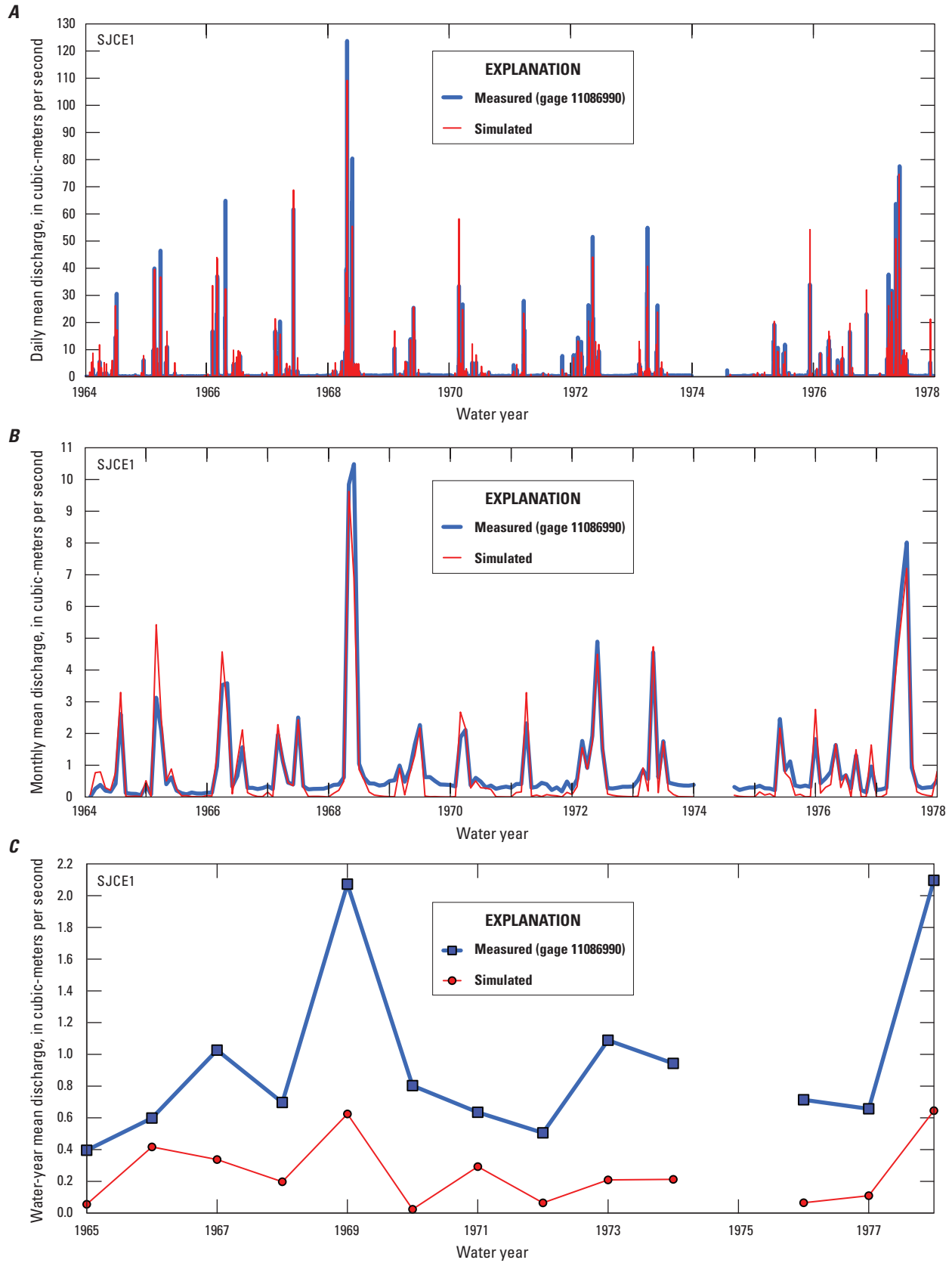
Figure 31. Comparison of simulated and measured streamflow at gage SJCE1, Los Angeles Basin watershed model (LABWM), California: A, daily; B, monthly; C, annually.
