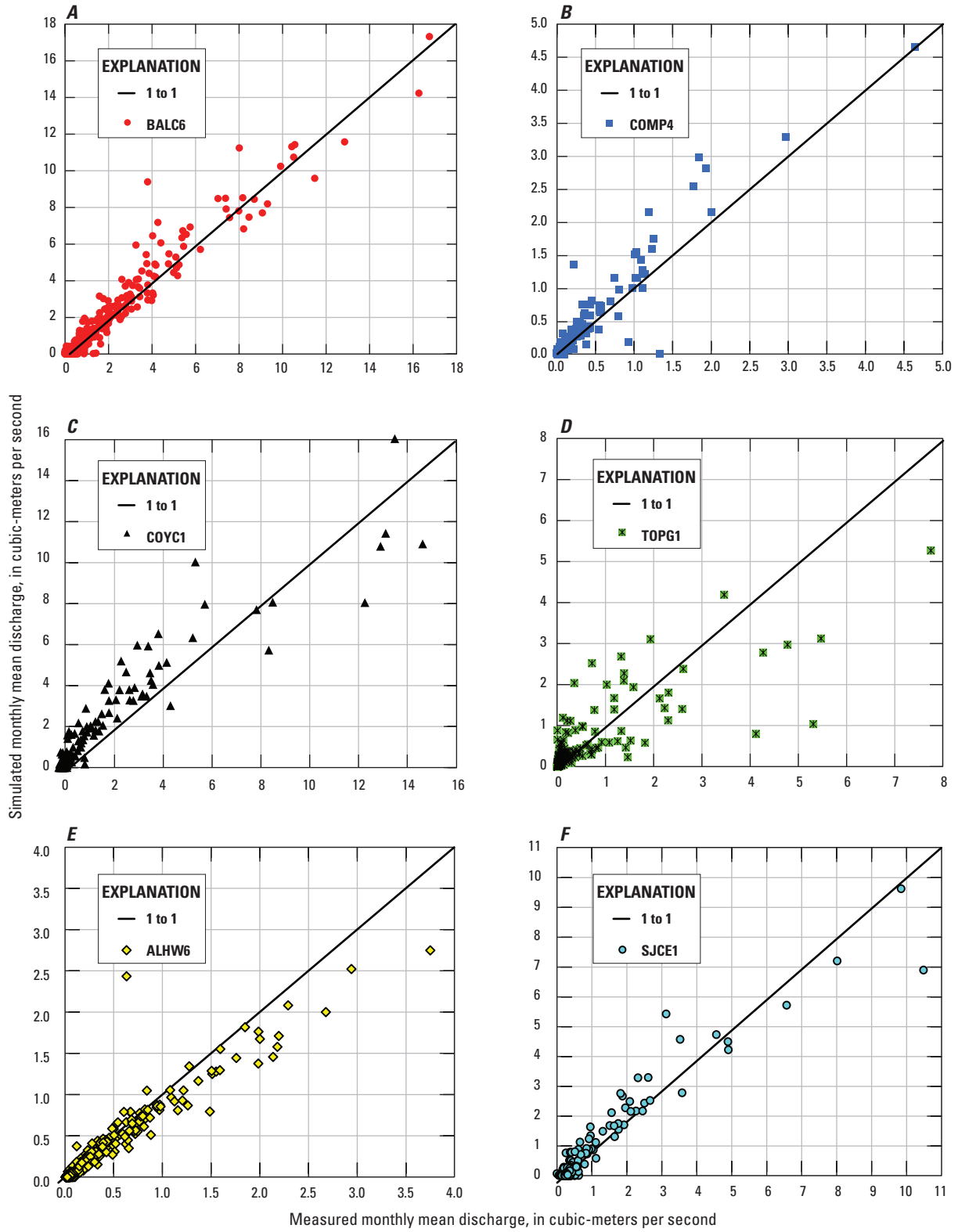
Figure 32. Simulated against measured monthly streamflow, Los Angeles Basin watershed model (LABWM), California, at gage A, BALC6; B, COMP4; C, COYC1; D, TOPG1; E, ALHW6; F, SJCE1.
