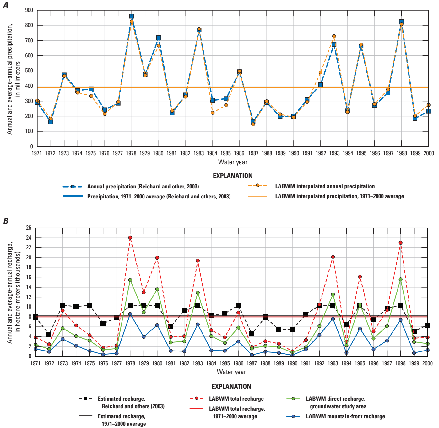
Figure 51. Comparison of annual results from a previous study and results from using the Los Angeles Basin watershed model (LABWM), California, for A , precipitation; and B , recharge.
