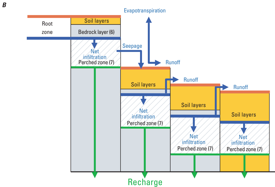
Figure 6. Grid, water storage components, and flow processes used by the INFILv3 code to simulate the spatial distribution of flows by the Los Angeles Basin watershed model (LABWM), California: A , the multi-layered root zone; B , the perched zone.
