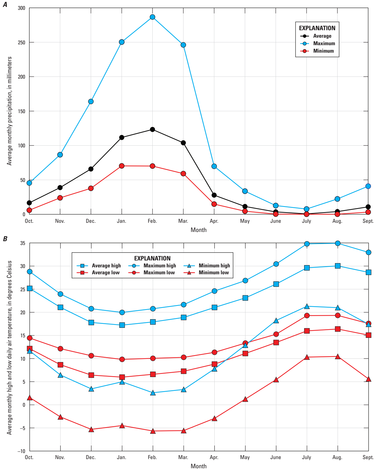
Figure 3. Average monthly values estimated for water years 1915–2014 for the Los Angeles Basin watershed model (LABWM) area, California, for A , precipitation; and B , maximum and minimum daily air temperature.
