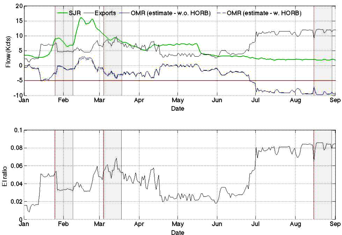
Figure 1: Flow data for WY 1999 – The three shaded areas represent the 3 two-week-long periods represented in Smith’s calculations.
