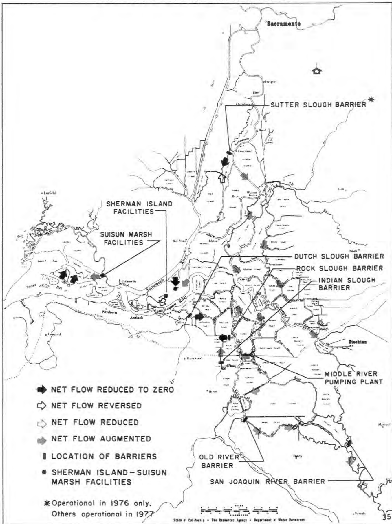
Figure 18. INFLUENCE OF BARRIERS AND OTHER FACILITIES ON DELTA FLOW PATTERNS 1976 and 1977
