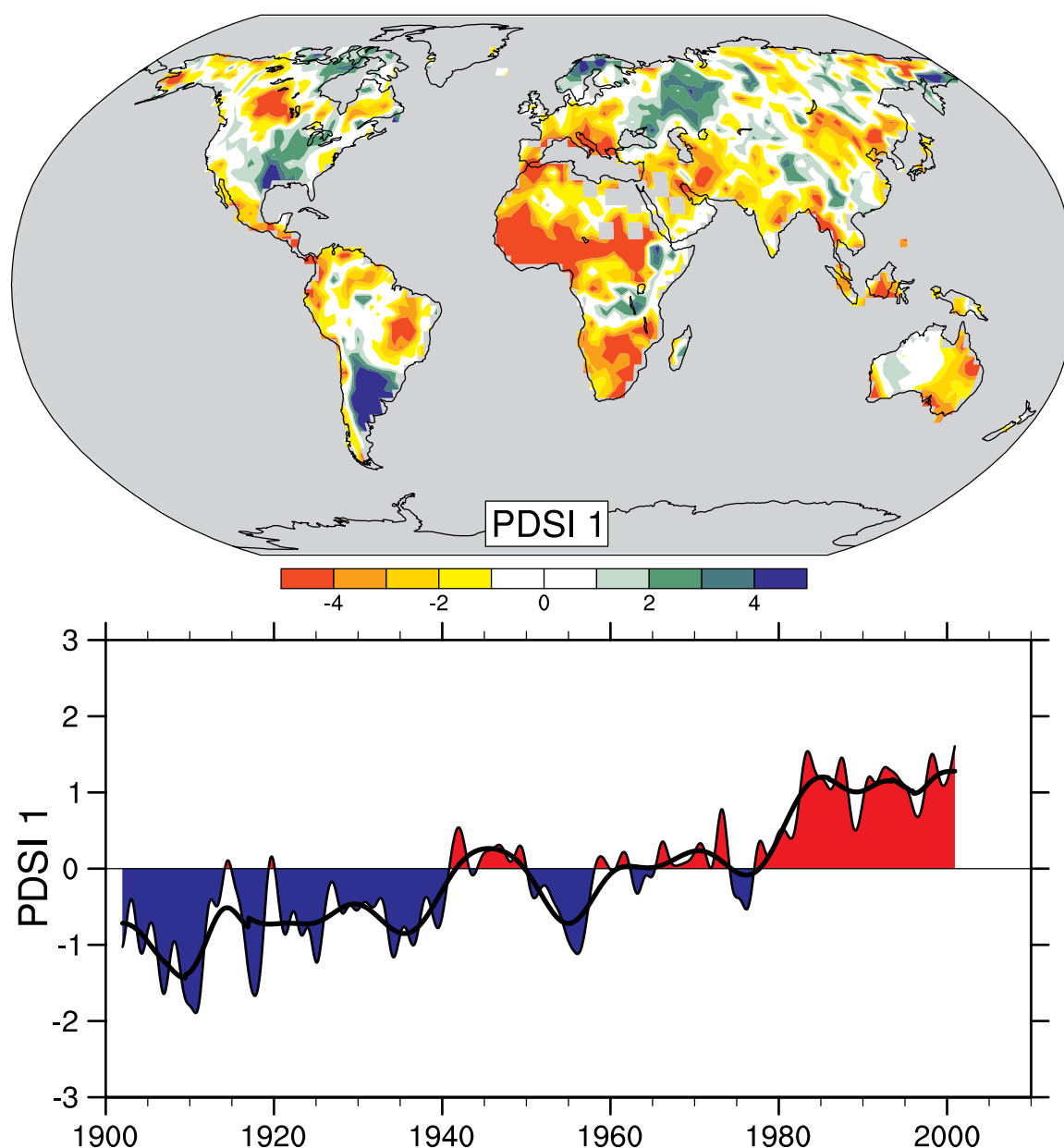
Figure 3.1: The most important spatial pattern (the first component of a principal components analysis; top) of the monthly Palmer Drought Severity Index (PDSI) for 1900 to 2002. The PDSI is a prominent index of drought and measures the cumulative deficit (relative to local mean conditions) in surface land moisture by incorporating previous precipitation and estimates of moisture drawn into the atmosphere (based on atmospheric temperatures) into a hydrological accounting system. 13 The lower panel shows how the sign and strength of this pattern has changed since 1900. When the values shown in the lower plot are positive (or negative), the red and orange areas in the upper map are drier (or wetter) and the blue and green areas are wetter (or drier) than average. The smooth black curve shows decadal variations. The time-series approximately corresponds to a trend, and this pattern and its variations account for 67% of the linear trend of PDSI from 1900 to 2002 over the global land area. It therefore features widespread increasing African drought, especially in the Sahel, for instance. Note also the wetter areas, especially in eastern North and South America and northern Eurasia (after Dai et al., 2004b). [WGI FAQ 3.2]
